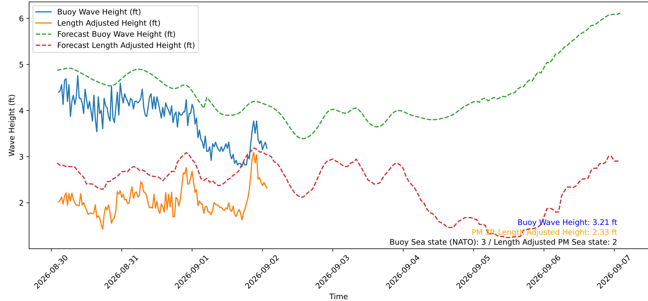
Wave Heights over Time for Green Beach at 2026-09-02 02:21:16
