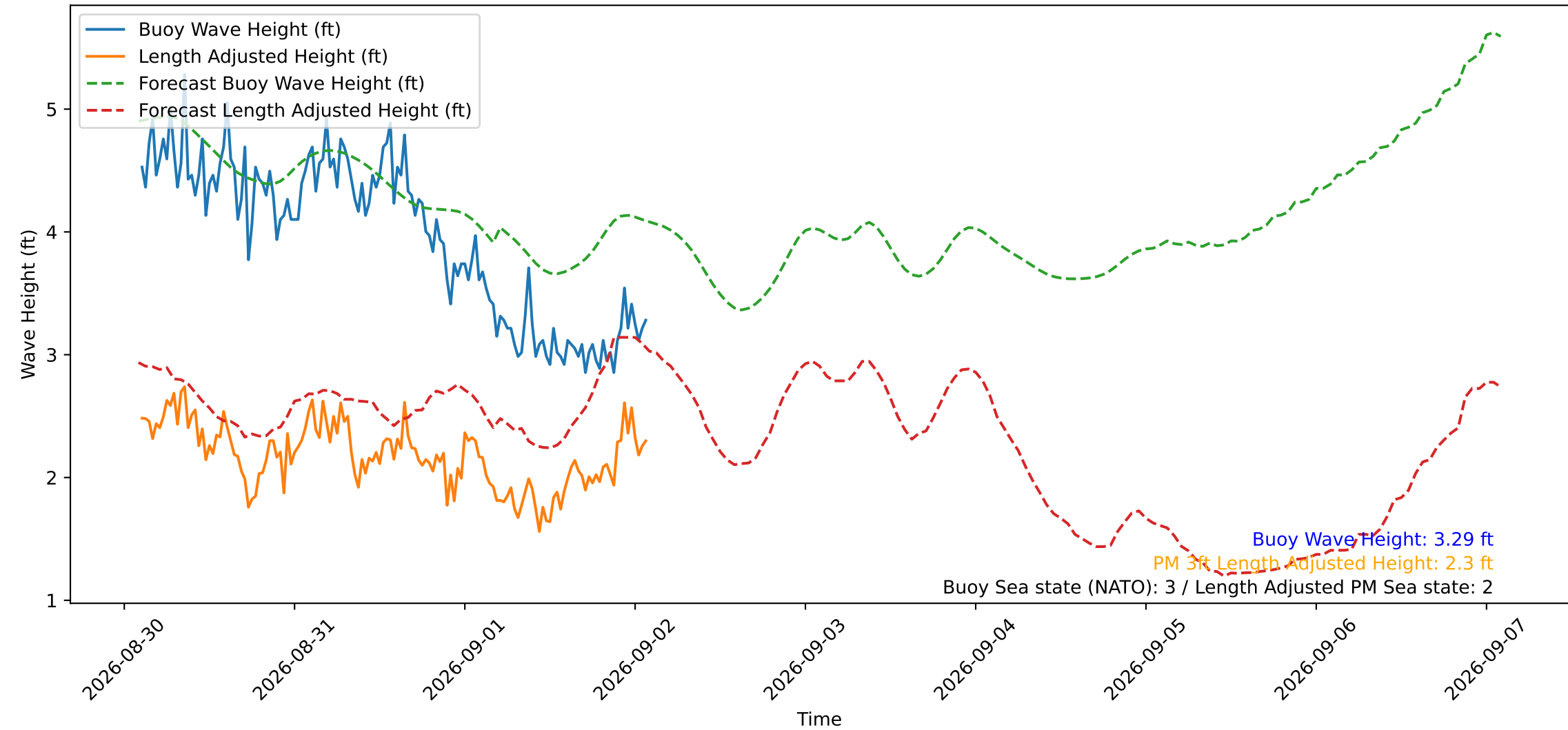
Wave Heights over Time for Oceanside Harbor at 2026-09-02 02:20:30
