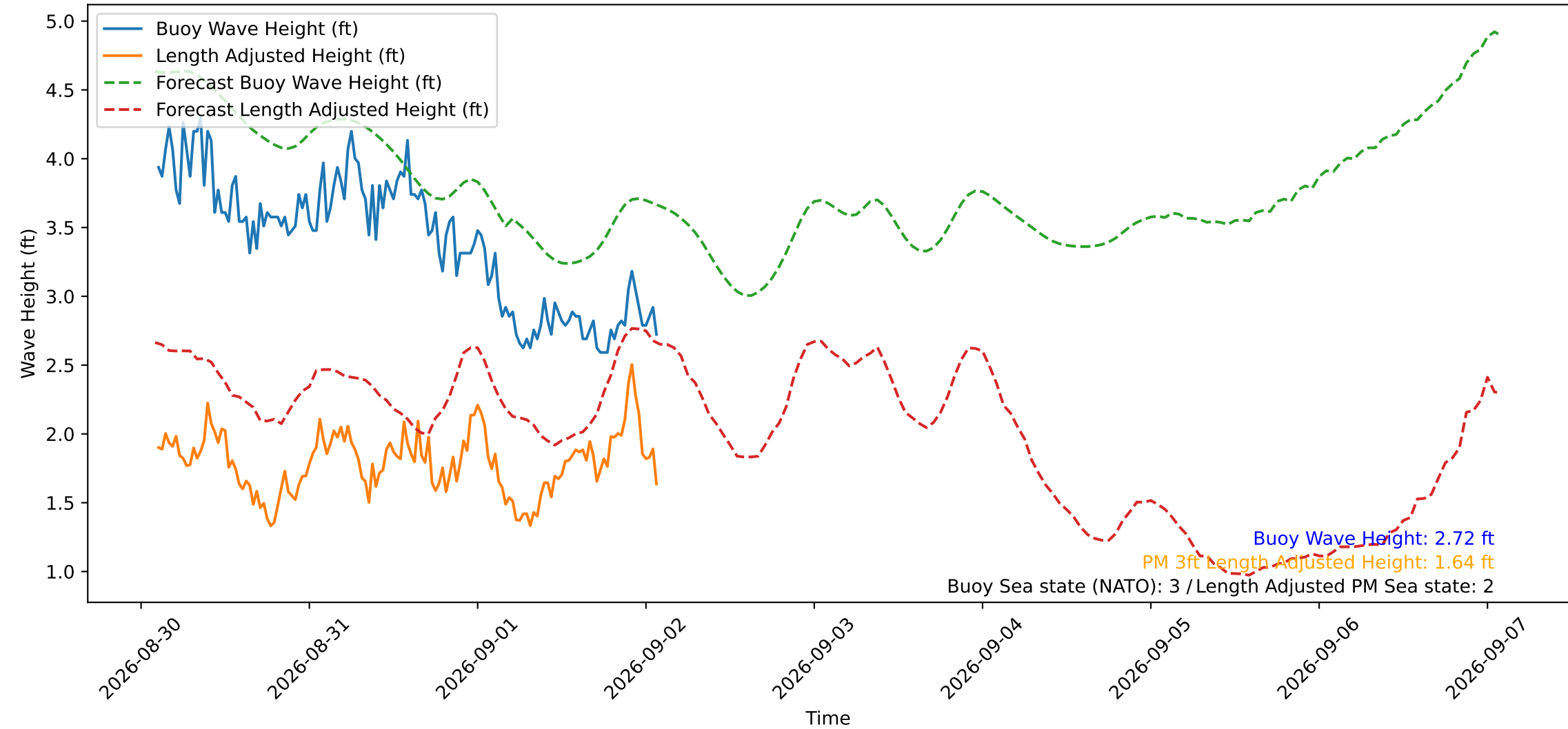
Wave Heights over Time for Red Beach at 2026-09-02 02:20:52
