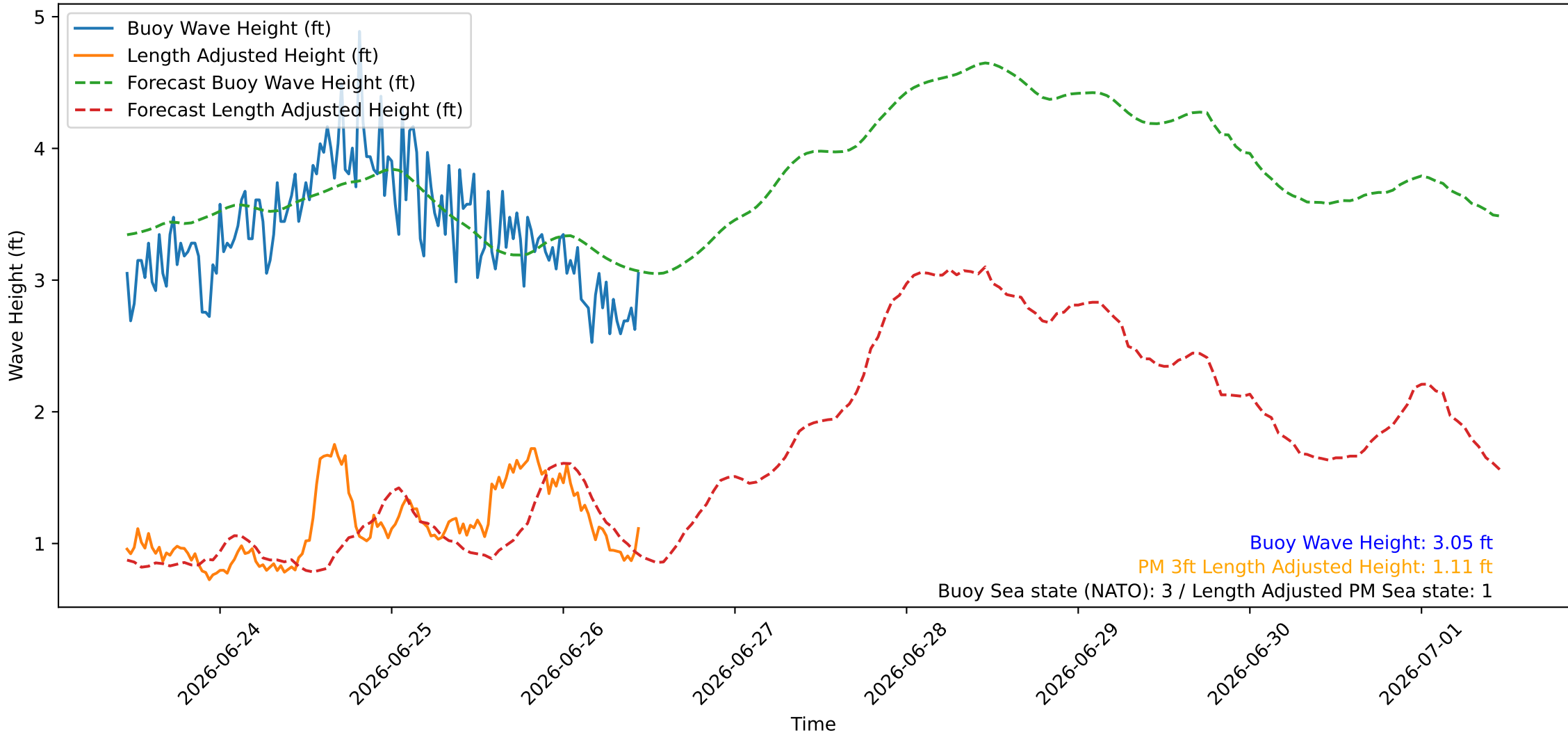
Wave Heights over Time for Oceanside Harbor at 2026-06-26 11:10:26
