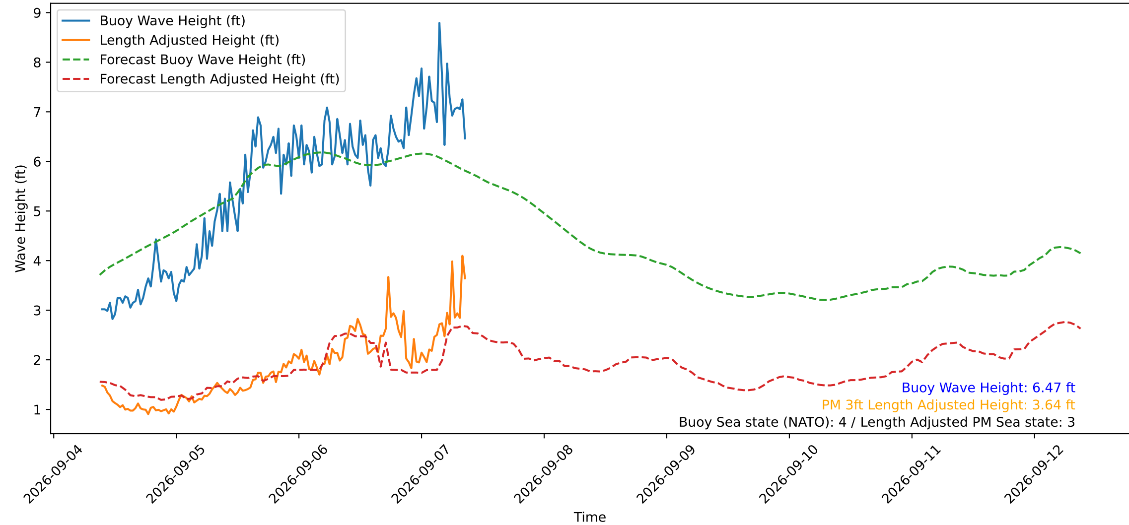
Wave Heights over Time for Green Beach at 2026-09-07 09:11:11
