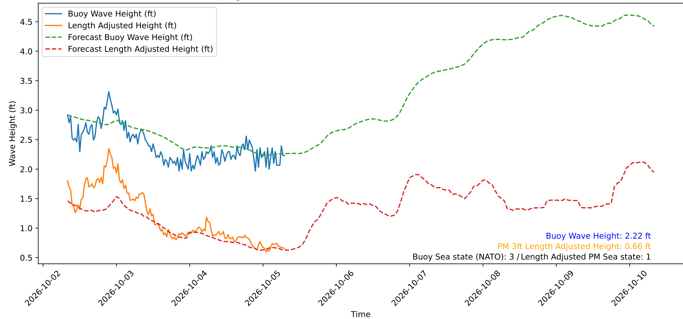
Wave Heights over Time for Oceanside Harbor at 2026-10-05 08:00:30
