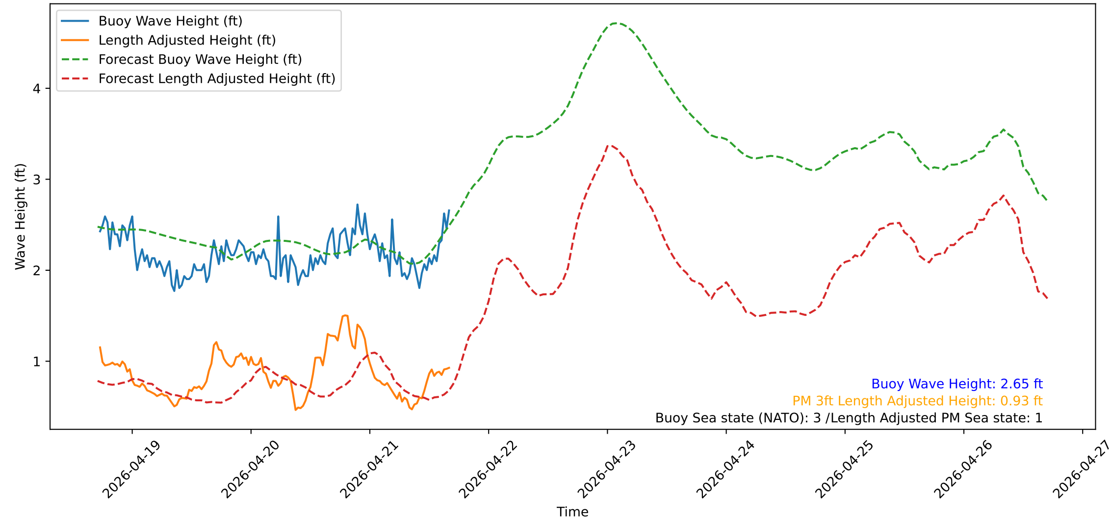
Wave Heights over Time for Red Beach at 2026-04-21 17:00:50
