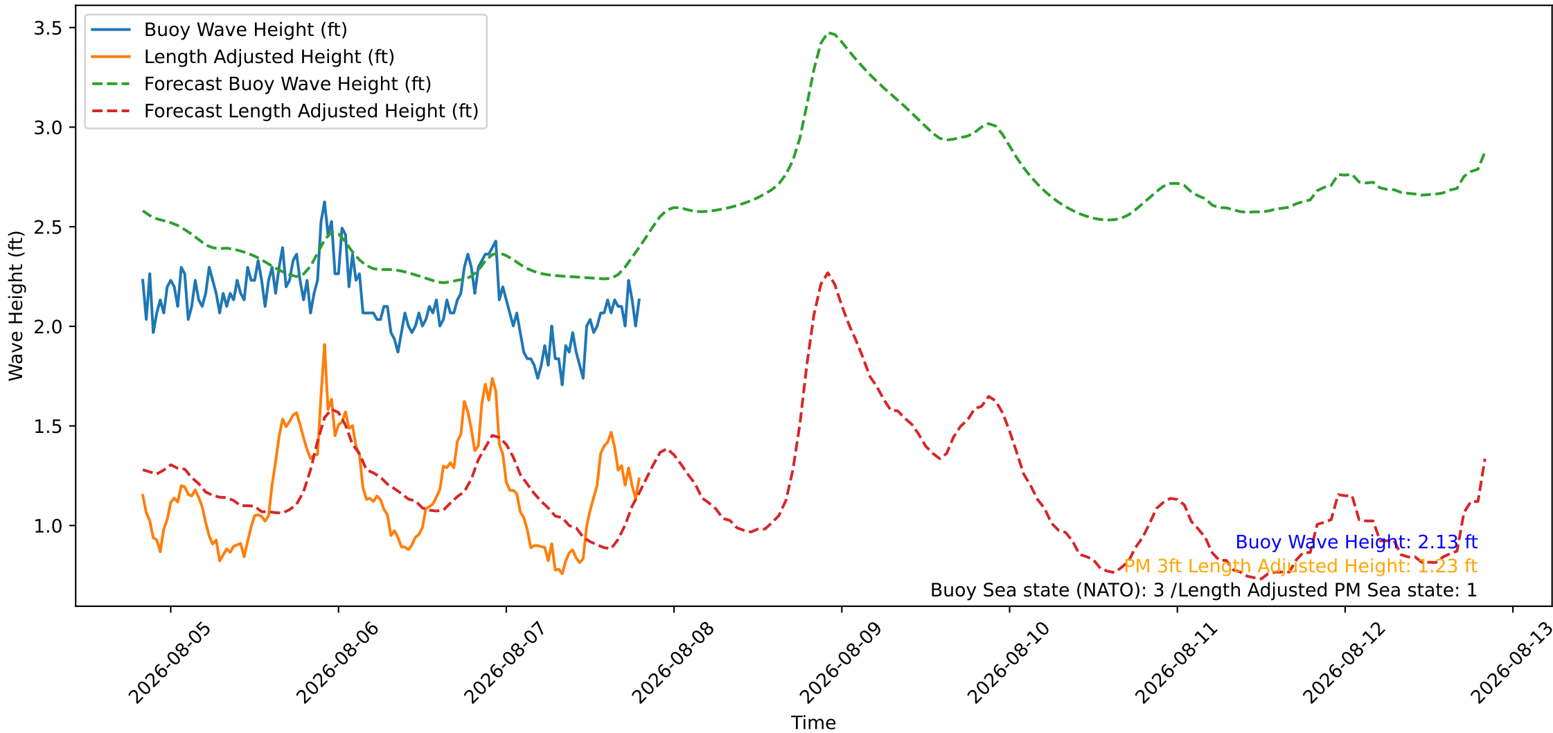
Wave Heights over Time for Green Beach at 2026-08-07 20:01:08
