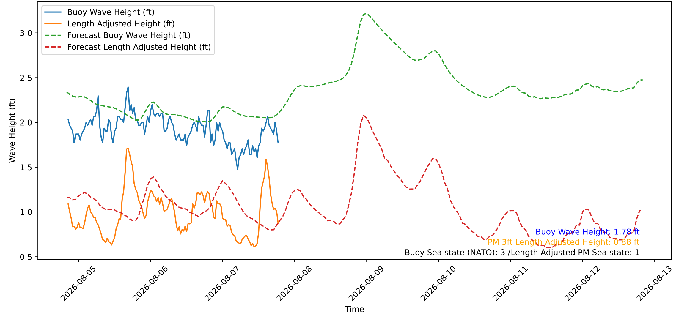
Wave Heights over Time for Red Beach at 2026-08-07 20:00:46
