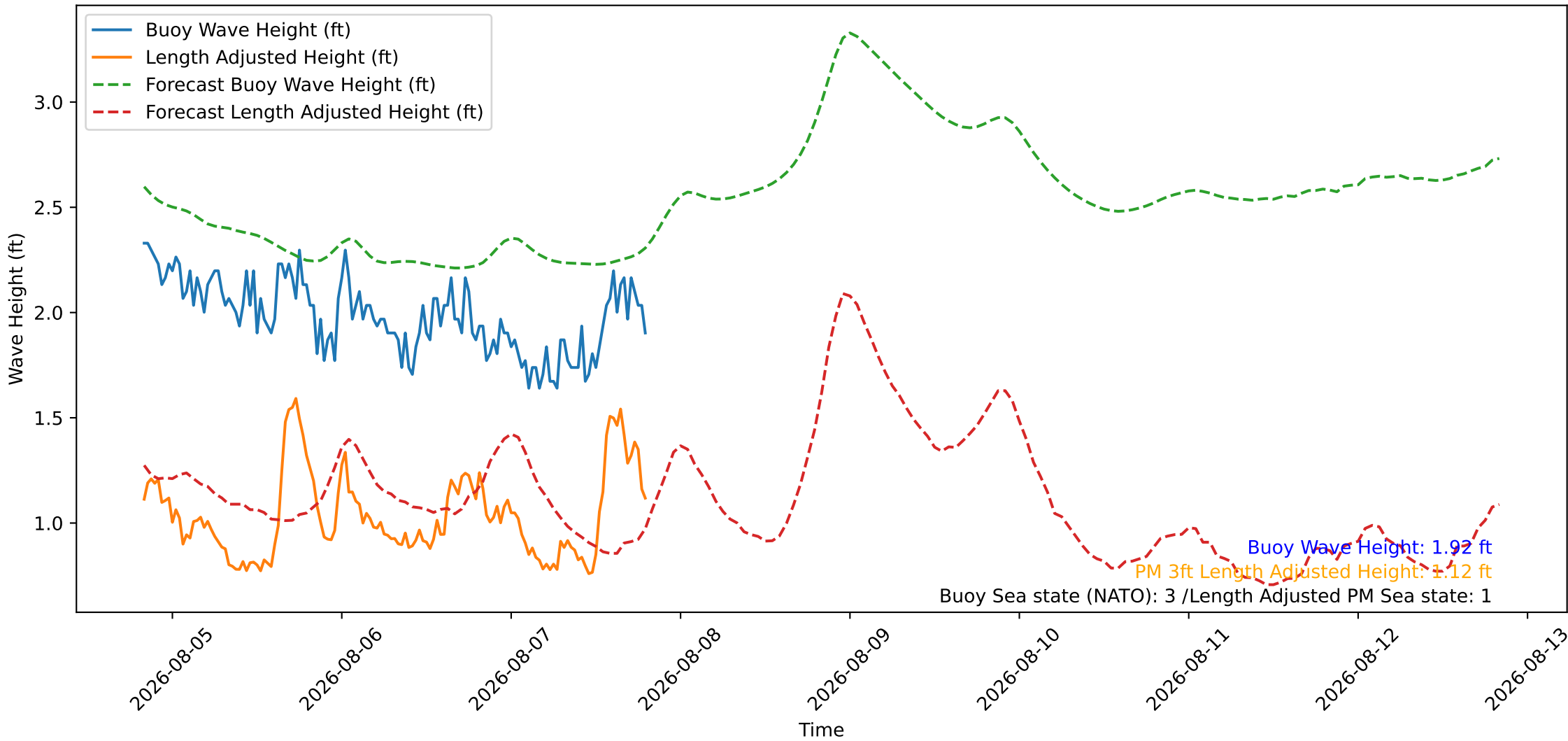
Wave Heights over Time for Oceanside Harbor at 2026-08-07 20:00:26
