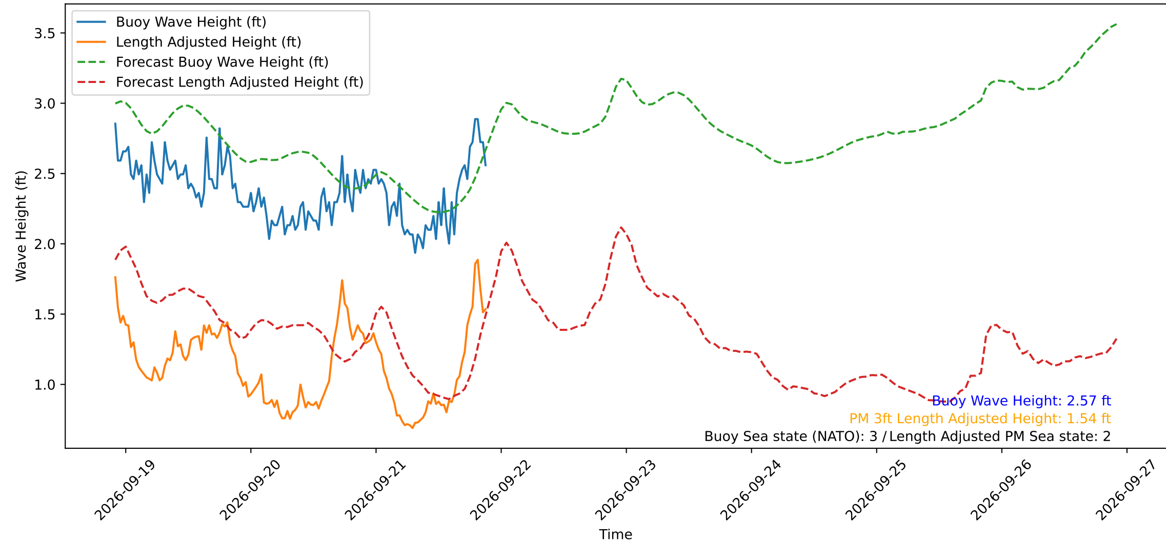
Wave Heights over Time for Red Beach at 2026-09-21 21:40:50
