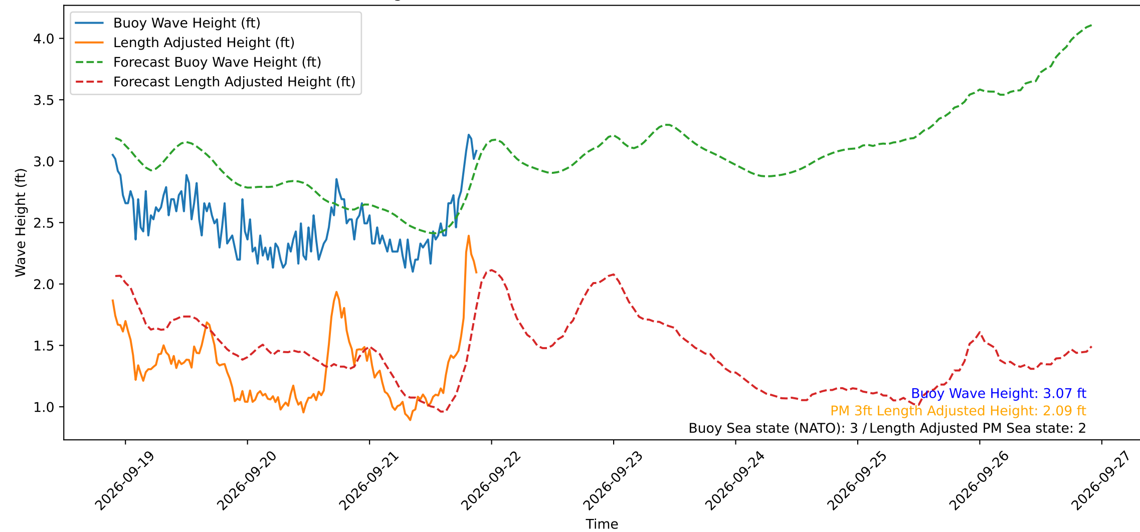
Wave Heights over Time for Oceanside Harbor at 2026-09-21 21:40:30
