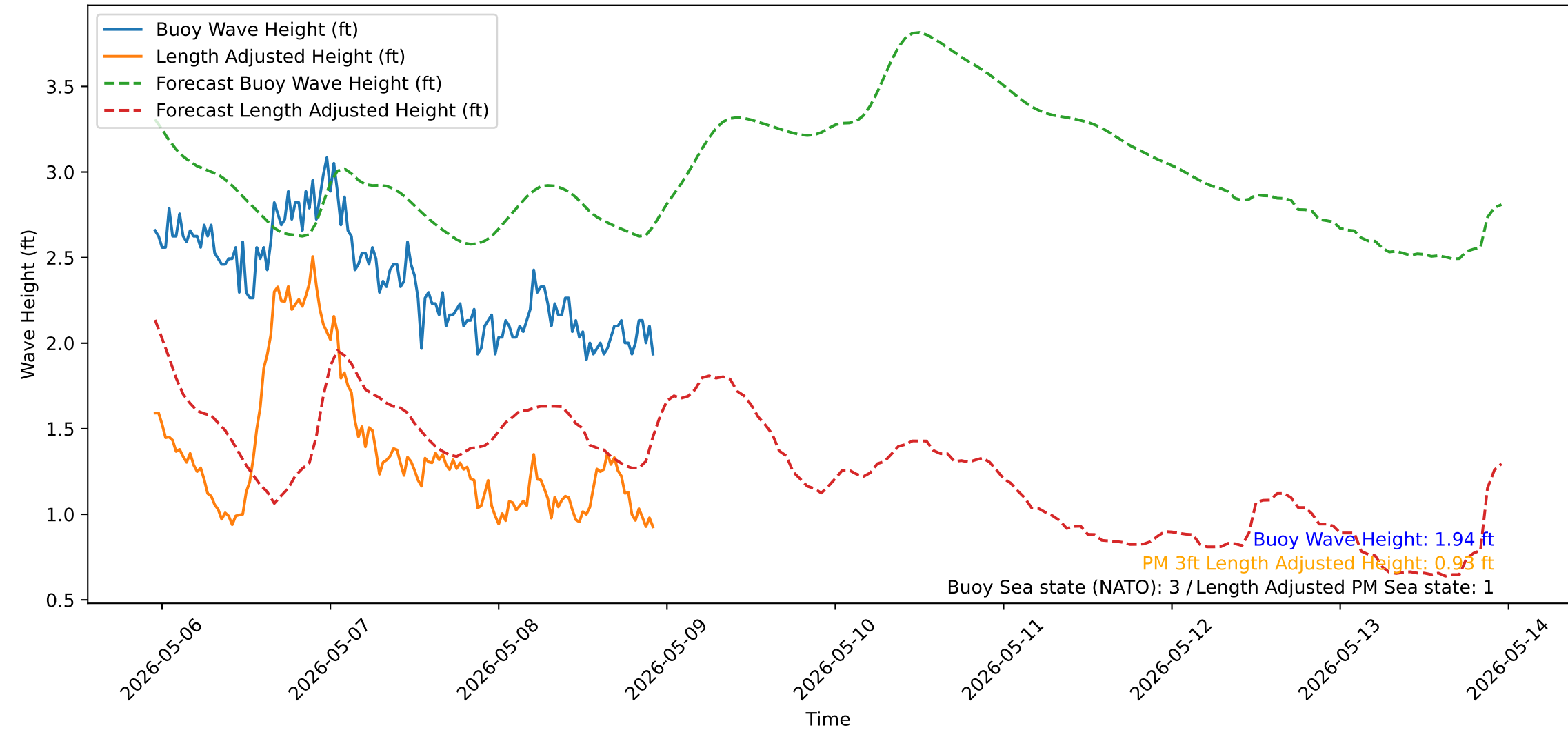
Wave Heights over Time for Red Beach at 2026-05-08 22:40:51
