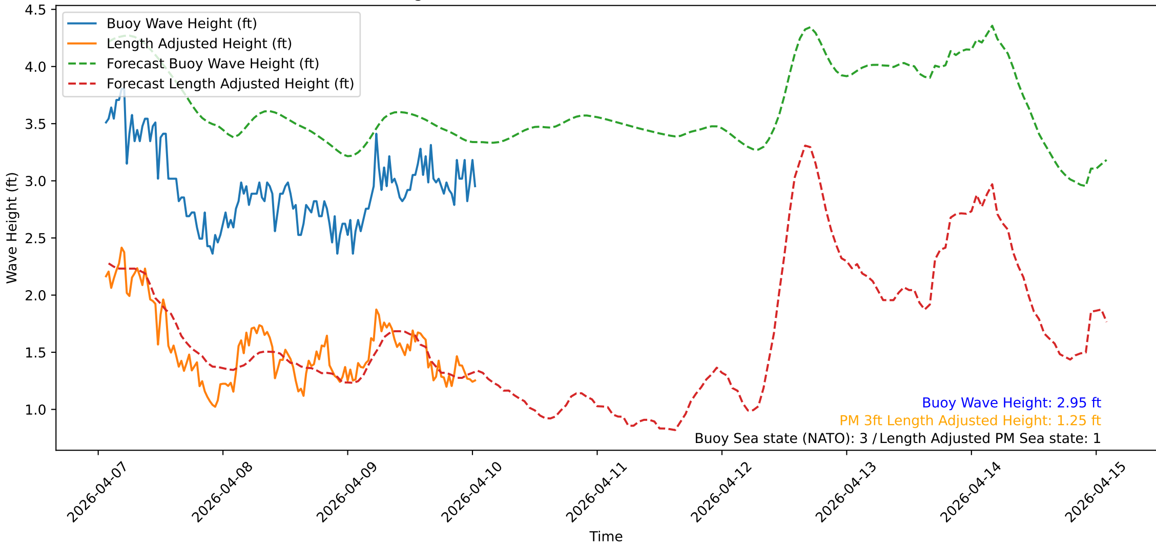
Wave Heights over Time for Green Beach at 2026-04-10 01:31:14
