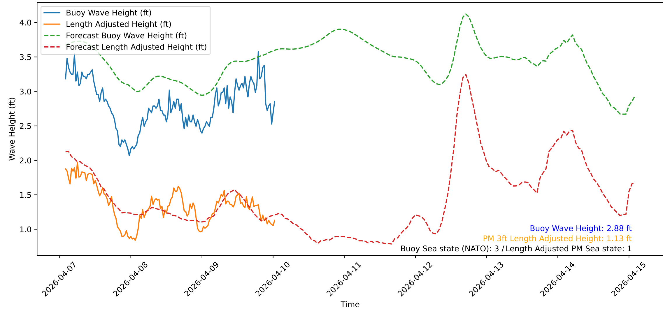
Wave Heights over Time for Red Beach at 2026-04-10 01:30:51
