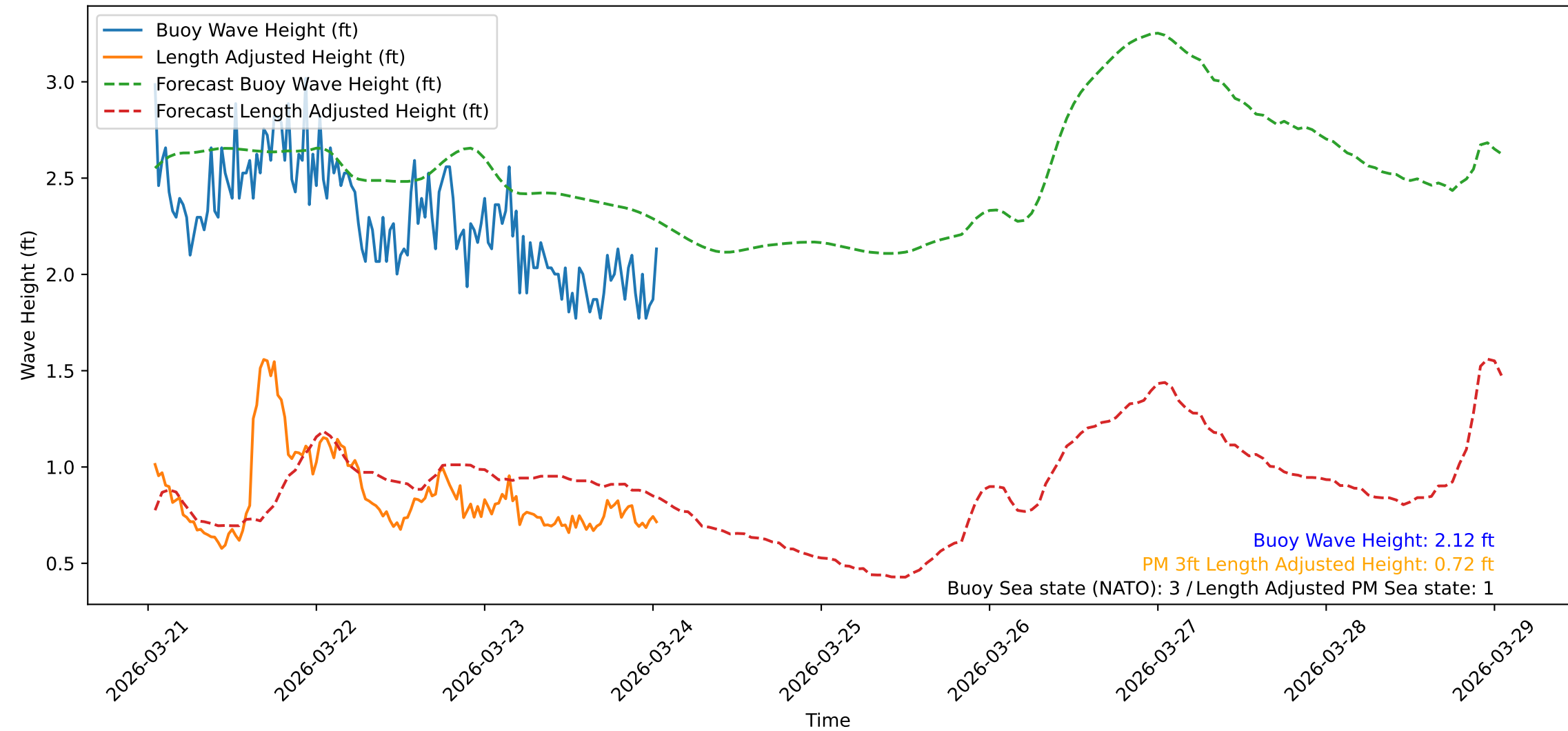
Wave Heights over Time for Oceanside Harbor at 2026-03-24 01:00:31
