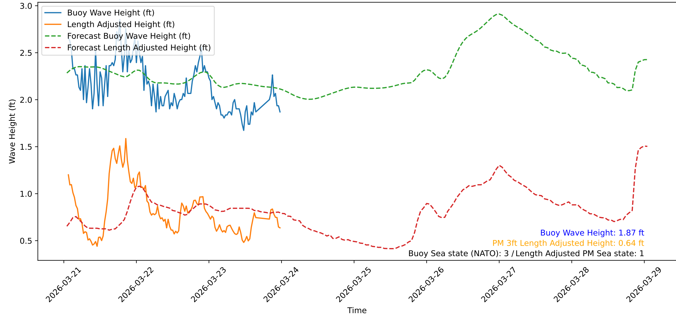
Wave Heights over Time for Red Beach at 2026-03-24 01:00:46
