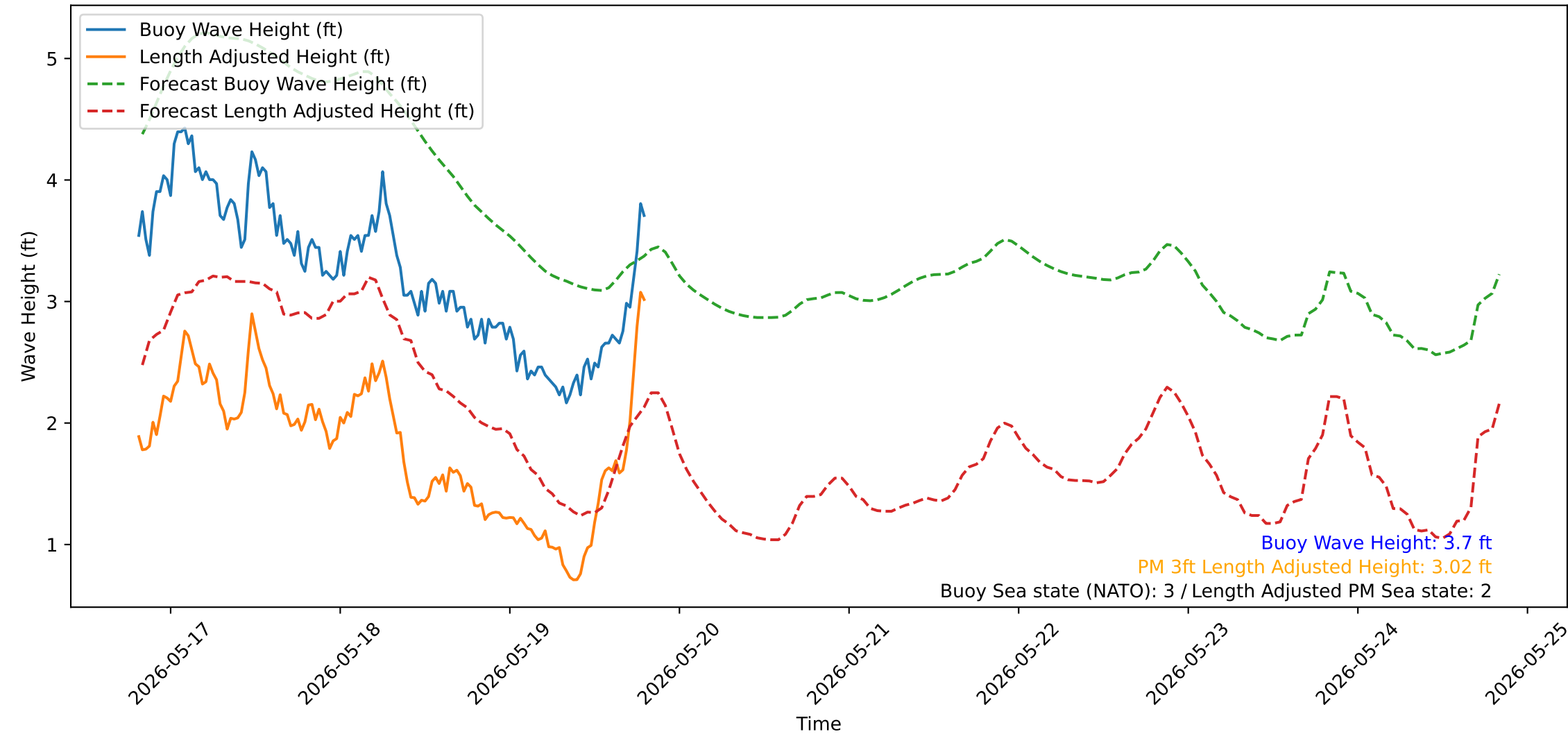
Wave Heights over Time for Green Beach at 2026-05-19 19:41:14
