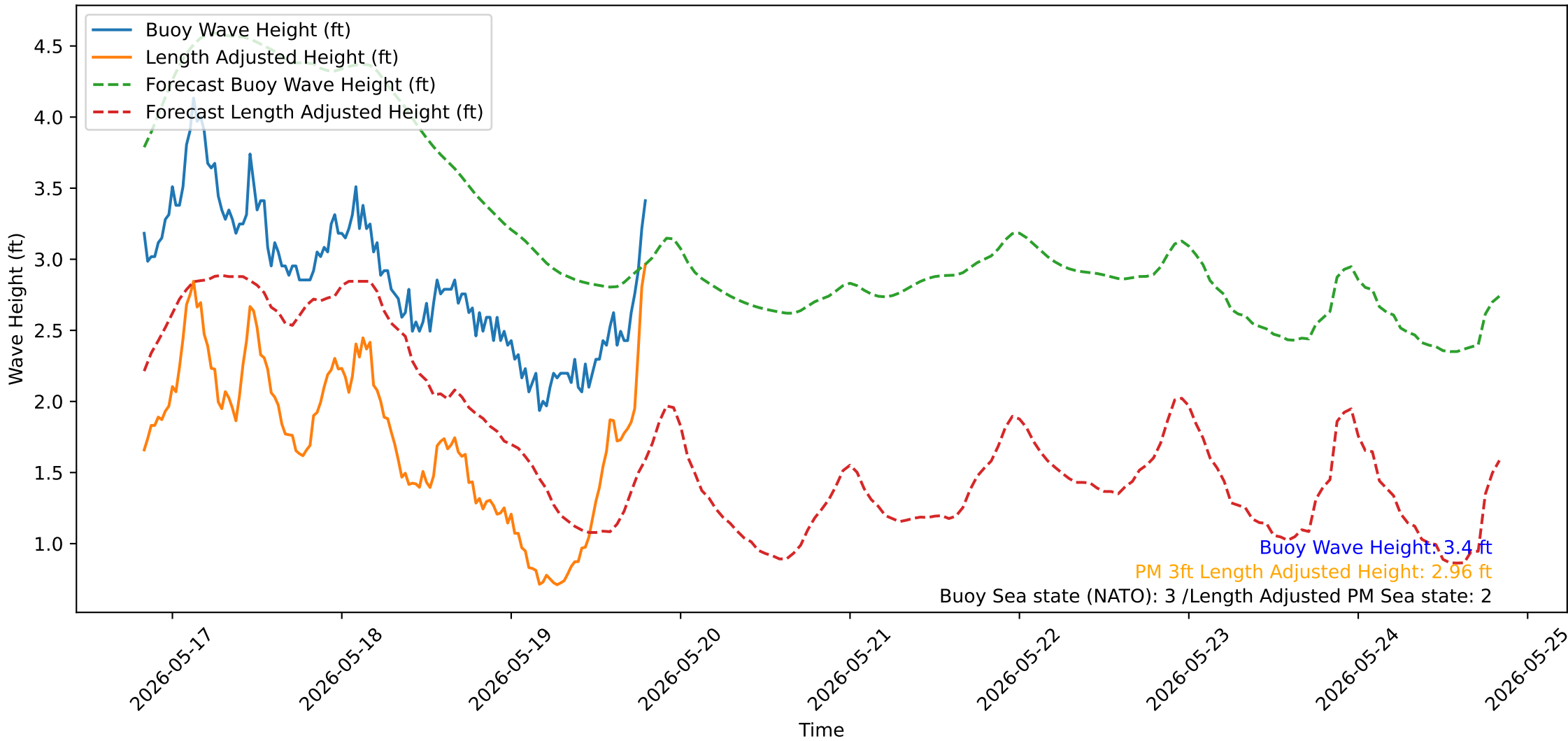
Wave Heights over Time for Red Beach at 2026-05-19 19:40:52
