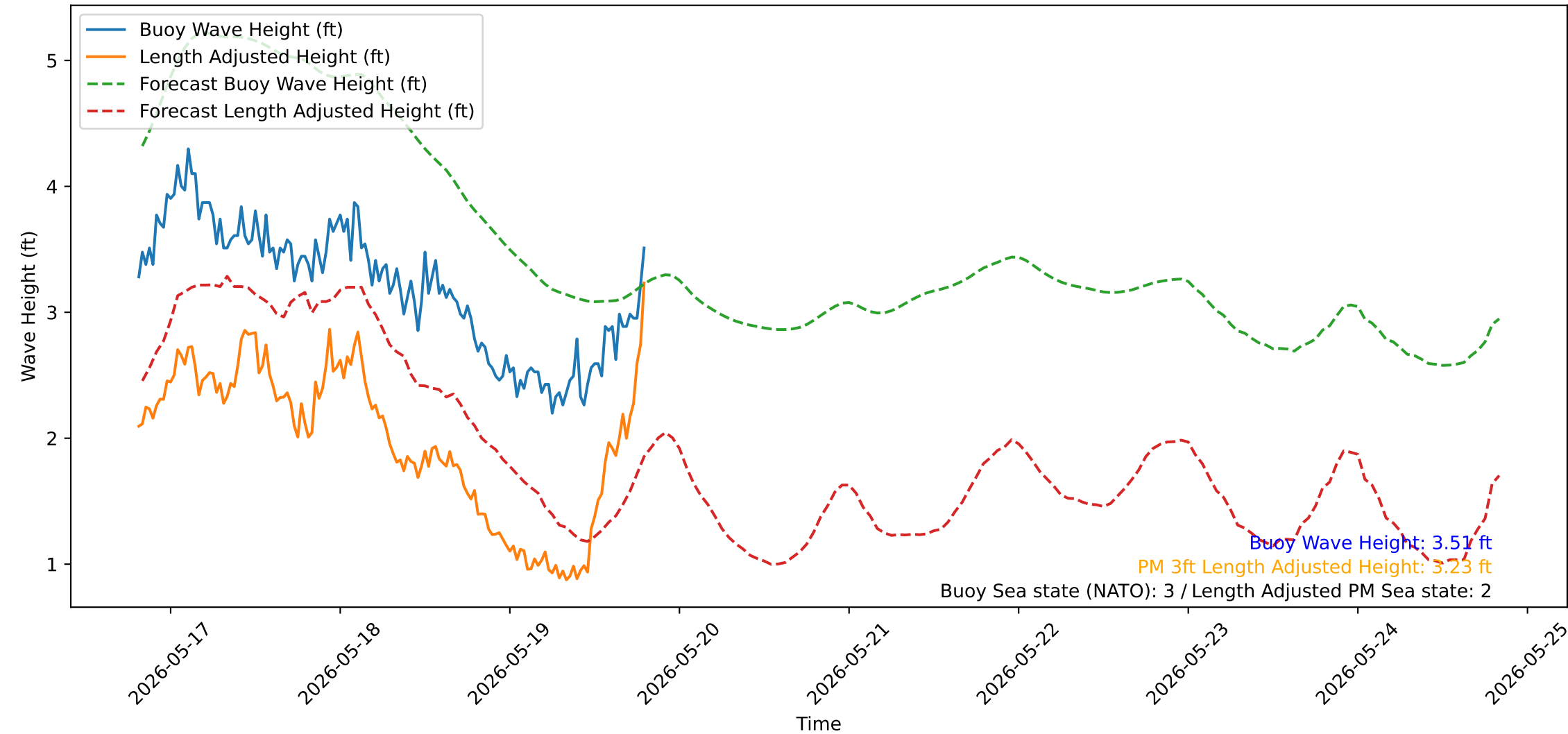
Wave Heights over Time for Oceanside Harbor at 2026-05-19 19:40:32
