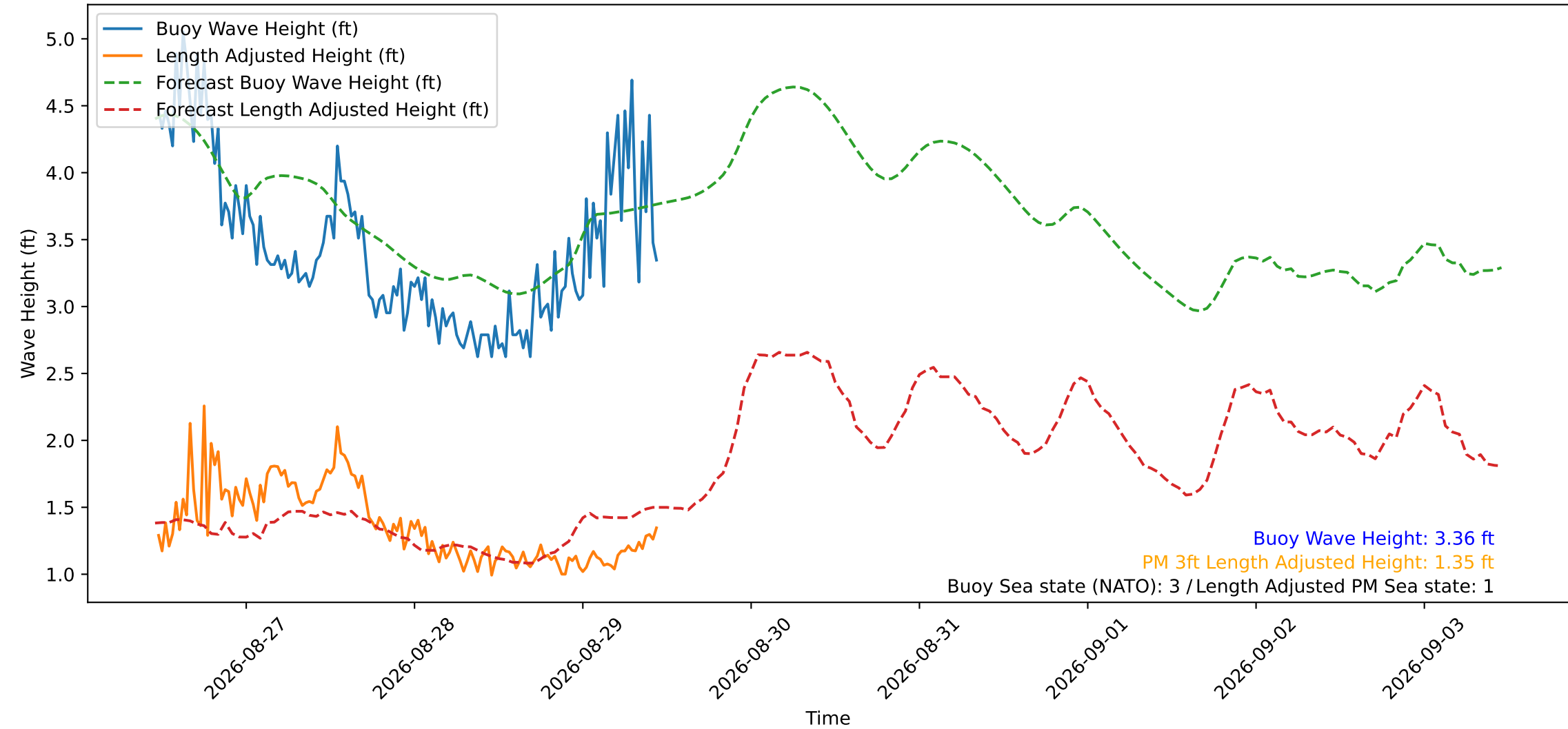
Wave Heights over Time for Red Beach at 2026-08-29 11:10:49
