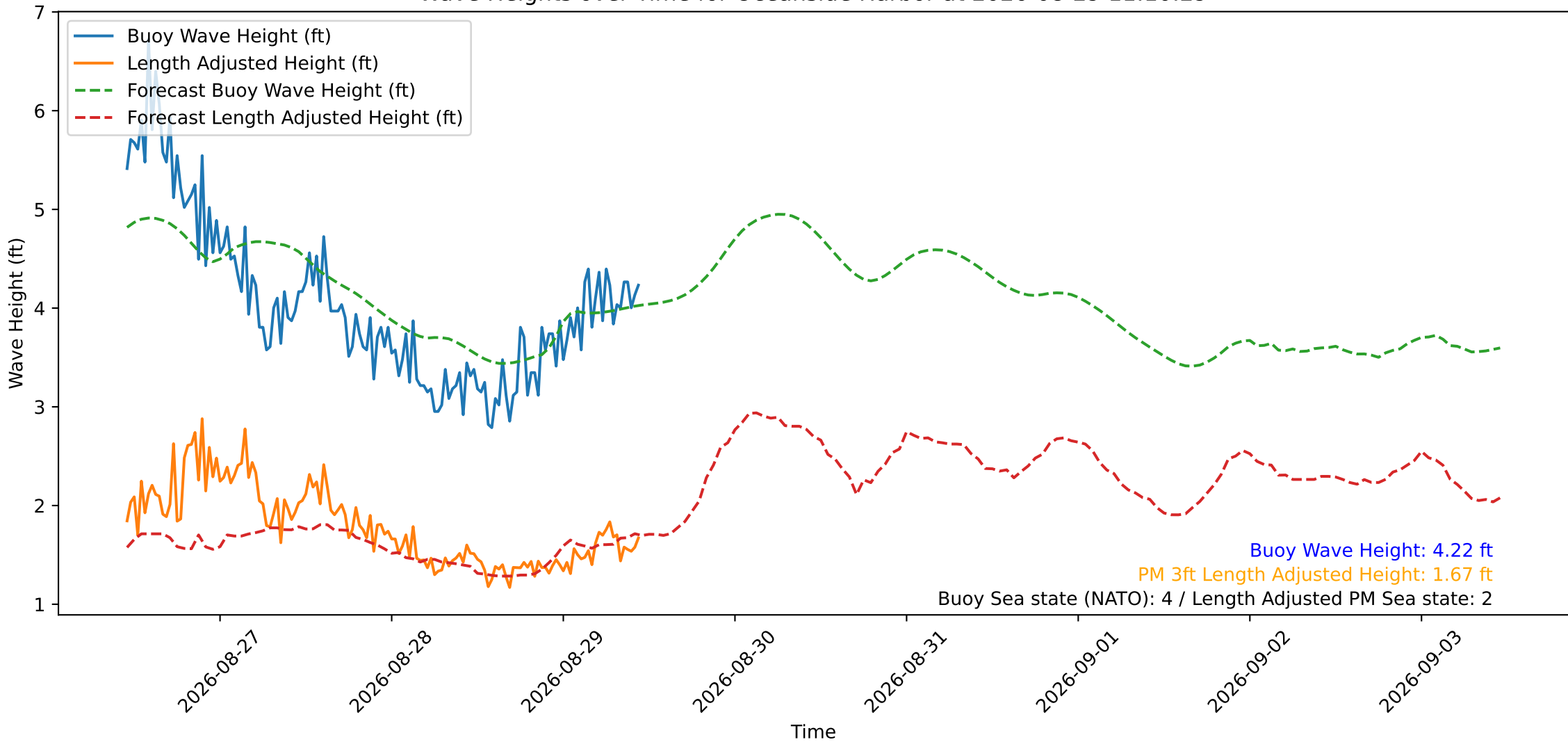
Wave Heights over Time for Oceanside Harbor at 2026-08-29 11:10:29
