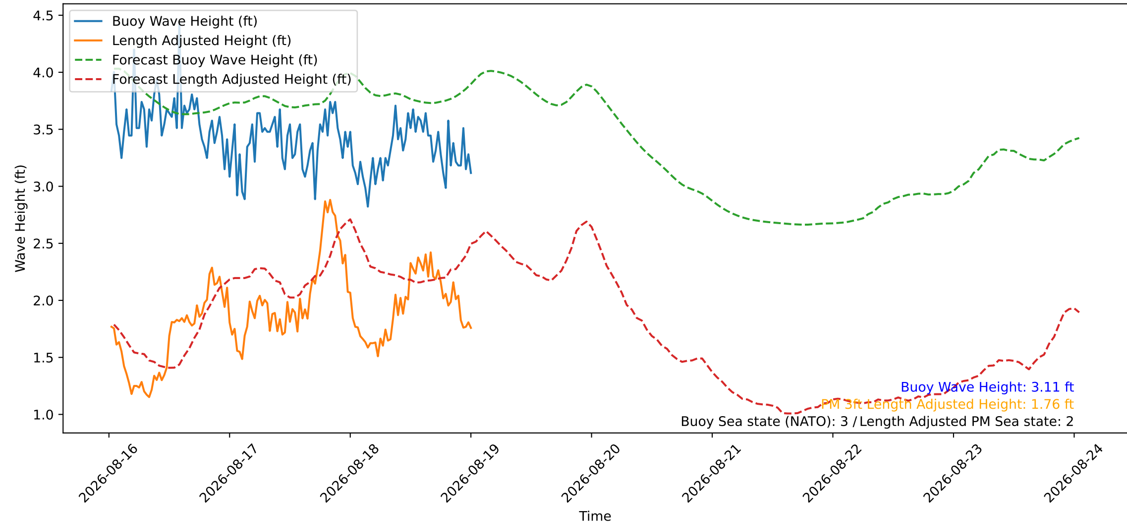
Wave Heights over Time for Oceanside Harbor at 2026-08-19 00:40:26
