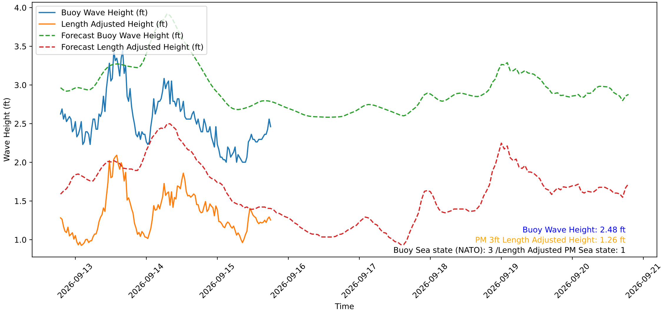
Wave Heights over Time for Red Beach at 2026-09-15 18:40:50
