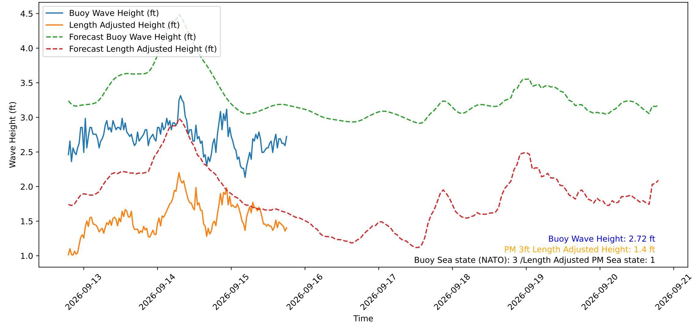
Wave Heights over Time for Green Beach at 2026-09-15 18:41:13
