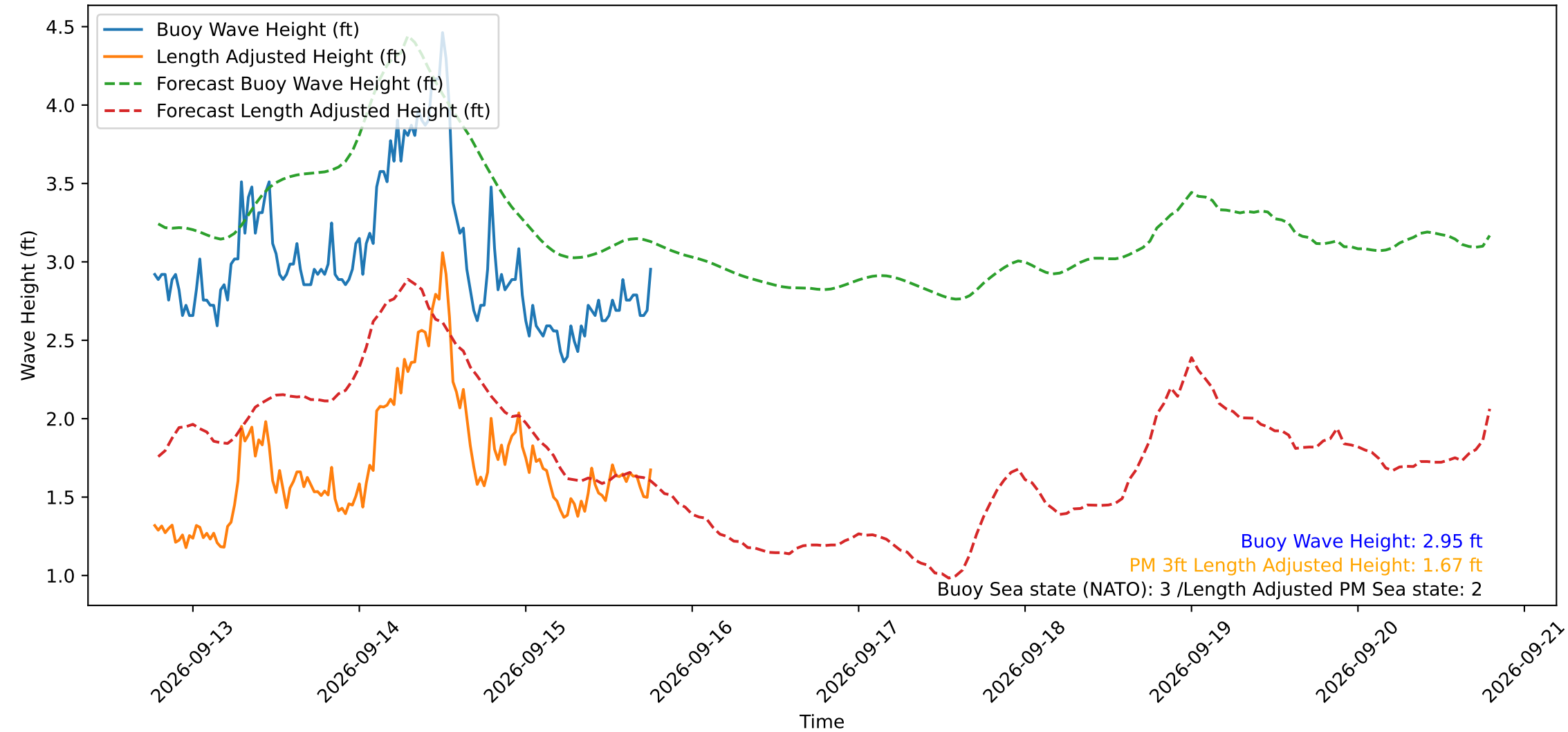
Wave Heights over Time for Oceanside Harbor at 2026-09-15 18:40:29
