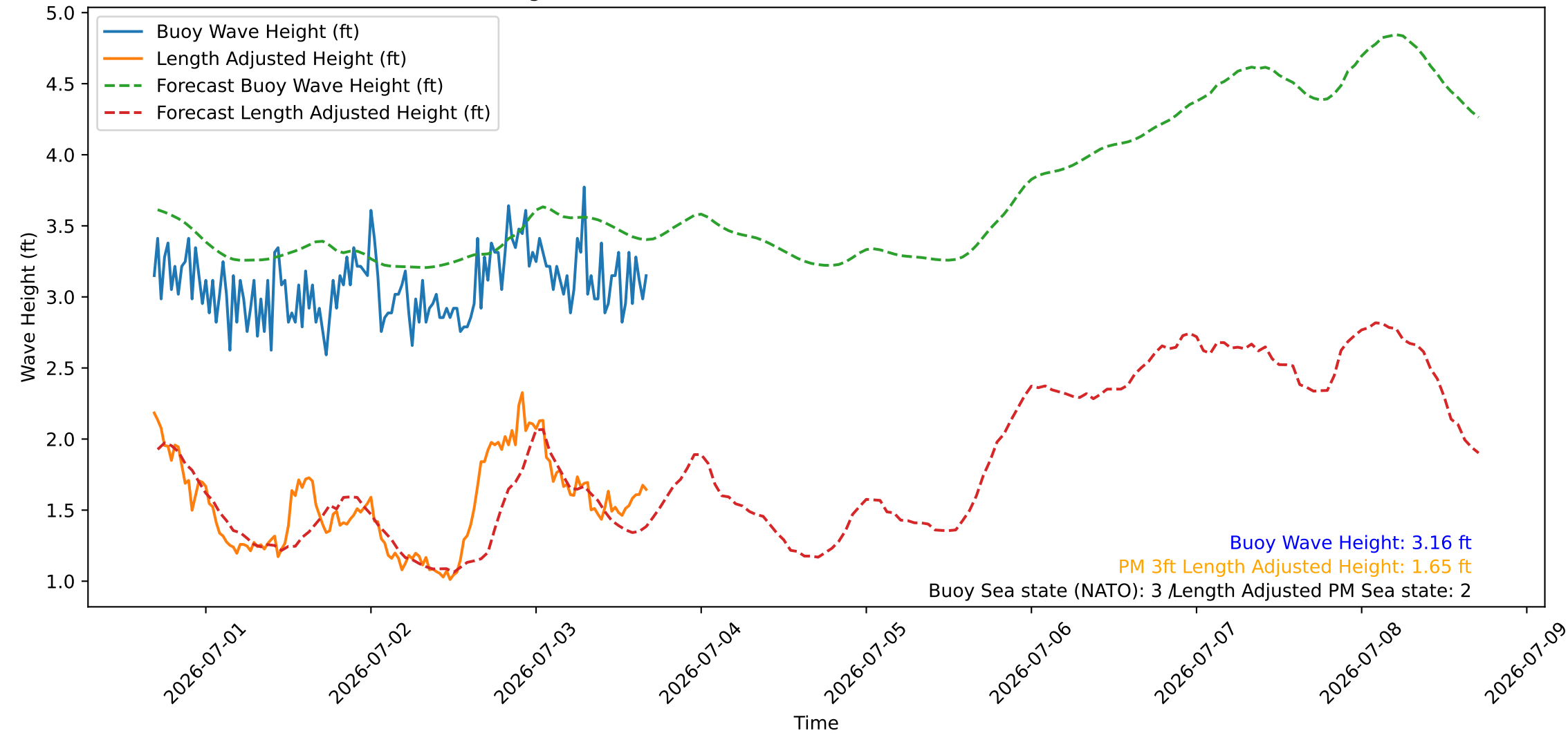
Wave Heights over Time for Oceanside Harbor at 2026-07-03 16:40:26
