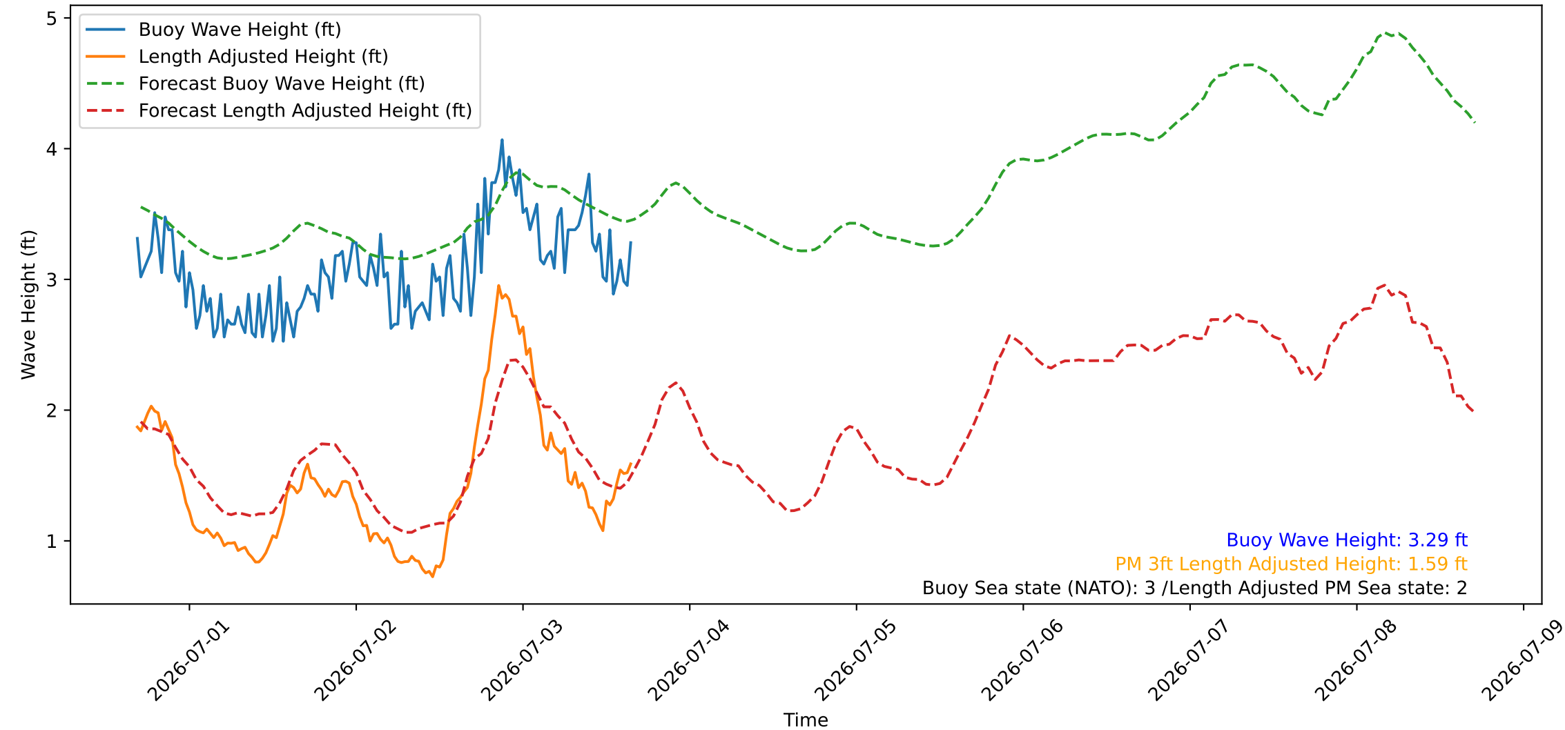
Wave Heights over Time for Green Beach at 2026-07-03 16:41:08
