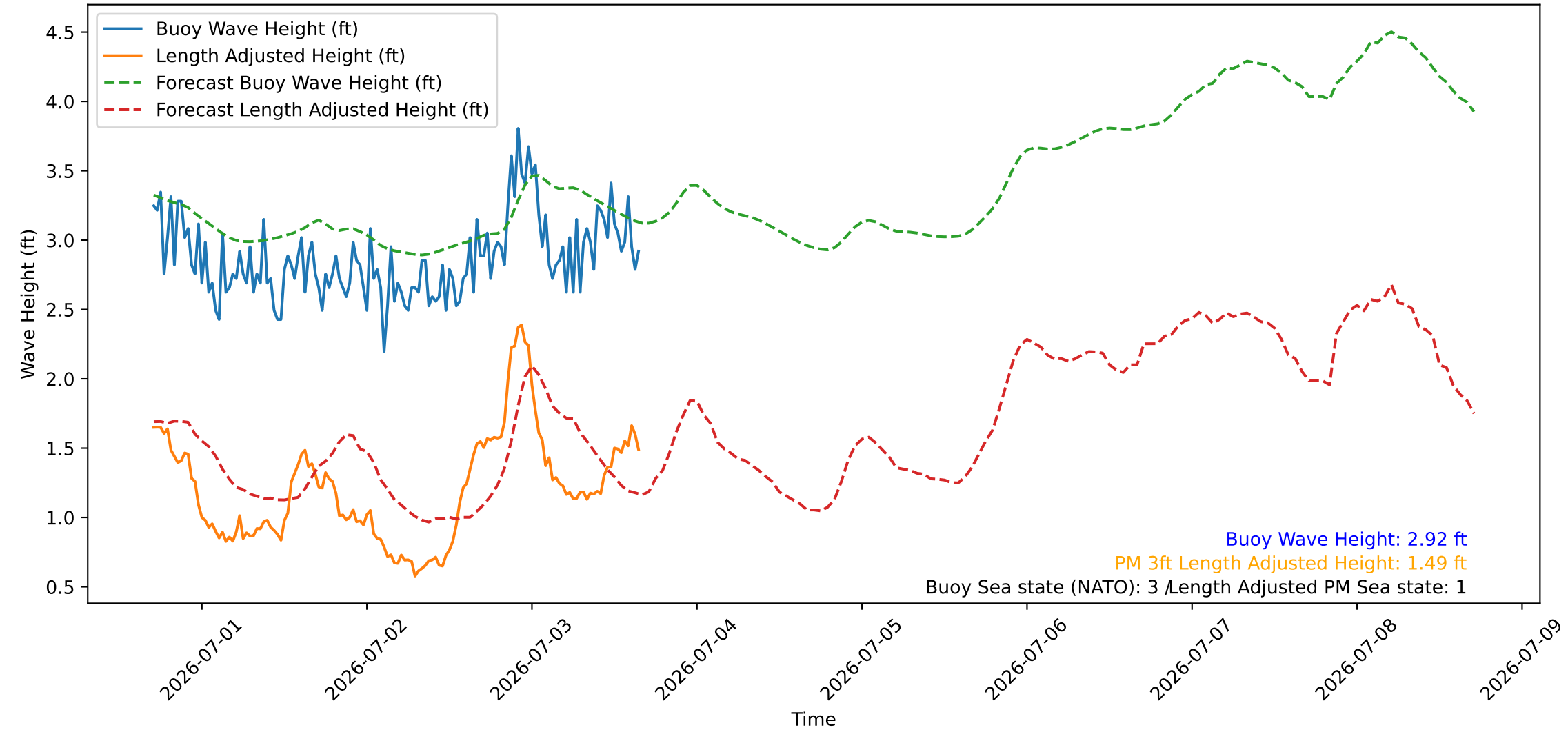
Wave Heights over Time for Red Beach at 2026-07-03 16:40:45
