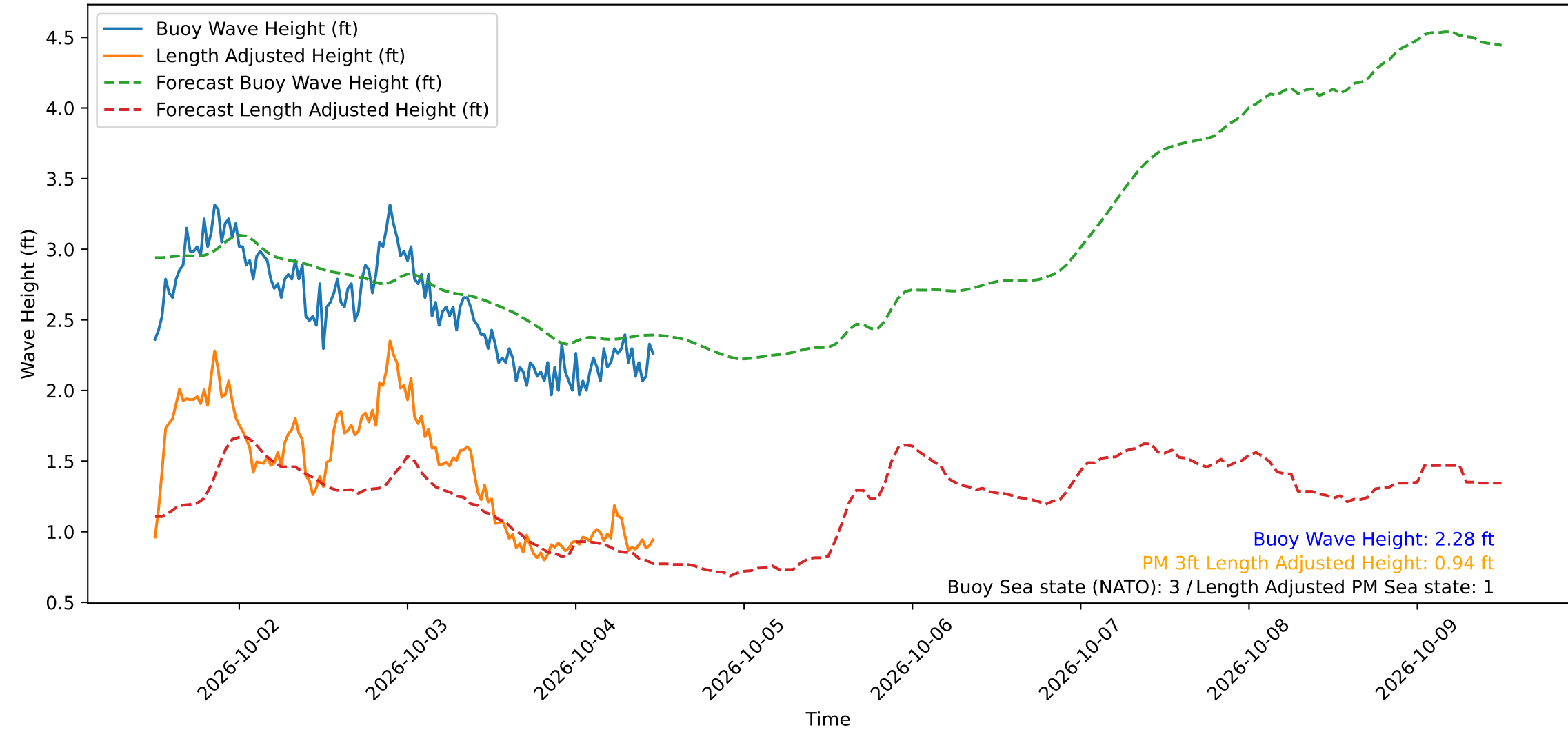
Wave Heights over Time for Oceanside Harbor at 2026-10-04 12:00:29
