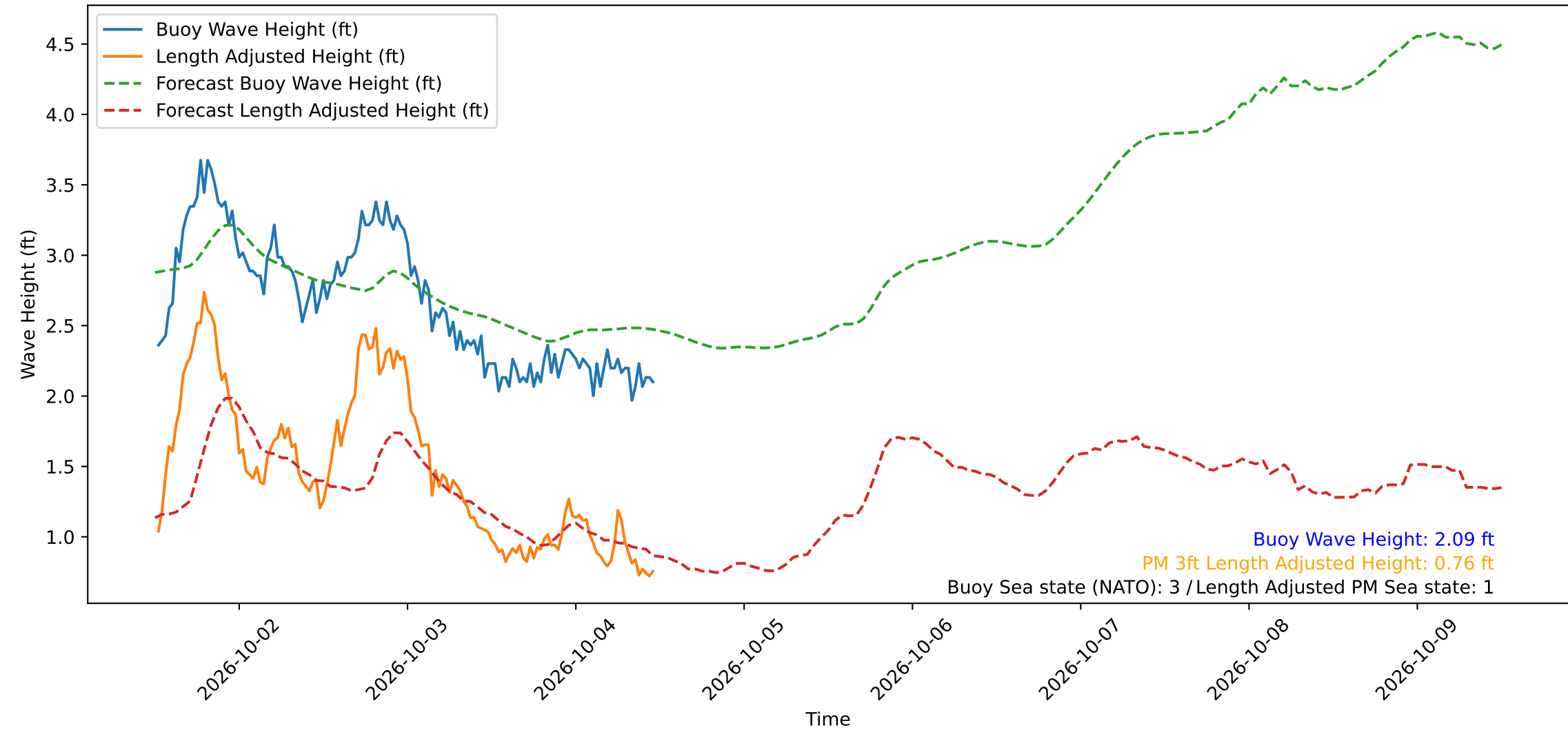
Wave Heights over Time for Green Beach at 2026-10-04 12:01:11
