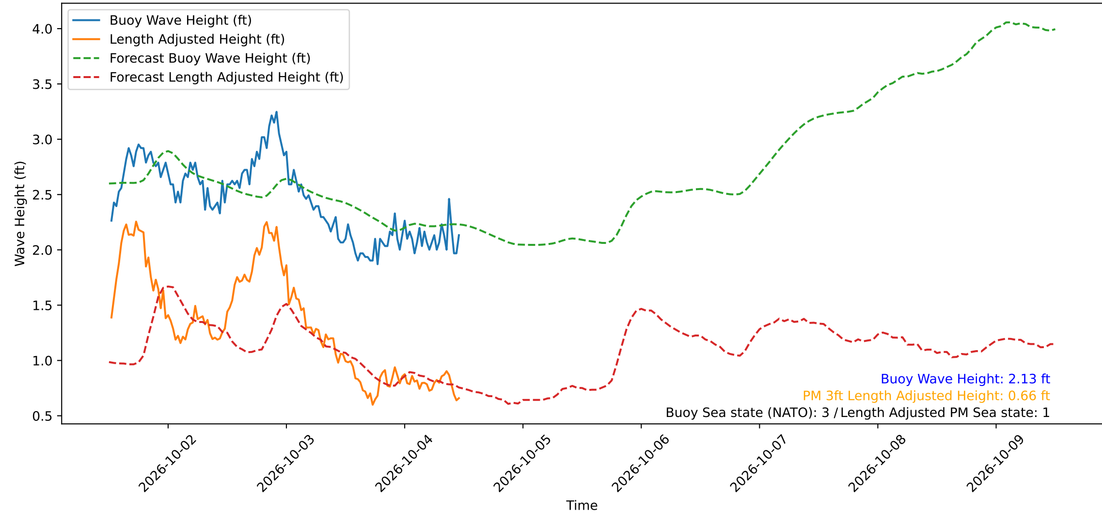
Wave Heights over Time for Red Beach at 2026-10-04 12:00:49
