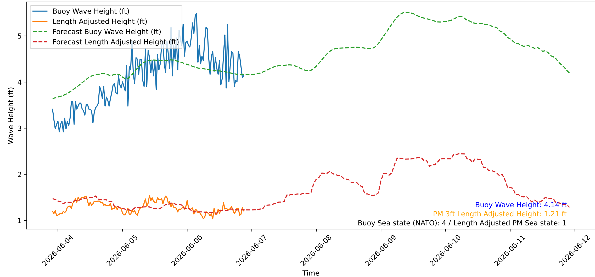
Wave Heights over Time for Oceanside Harbor at 2026-06-06 21:50:26
