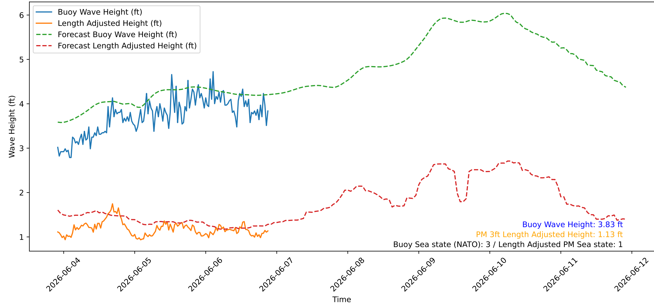
Wave Heights over Time for Green Beach at 2026-06-06 21:51:09
