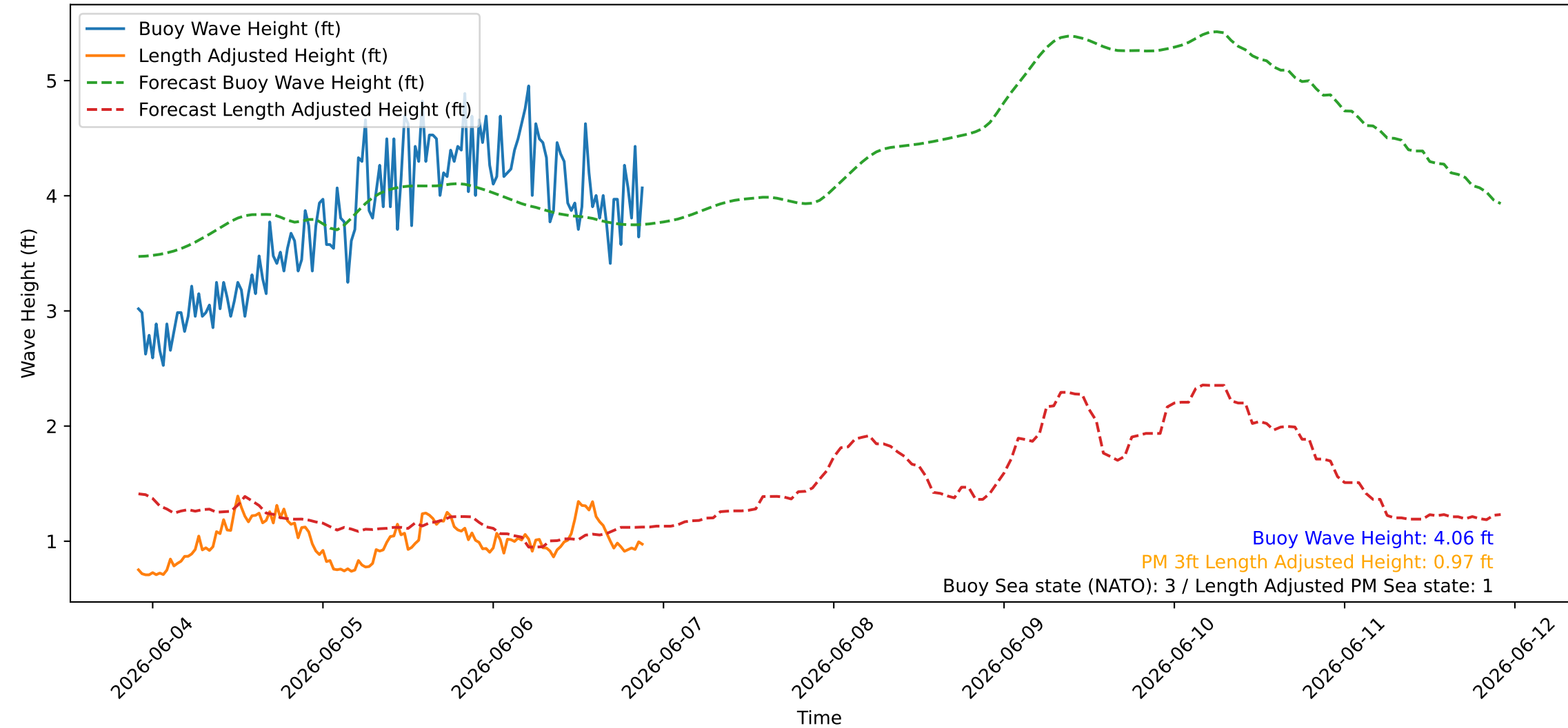
Wave Heights over Time for Red Beach at 2026-06-06 21:50:47
