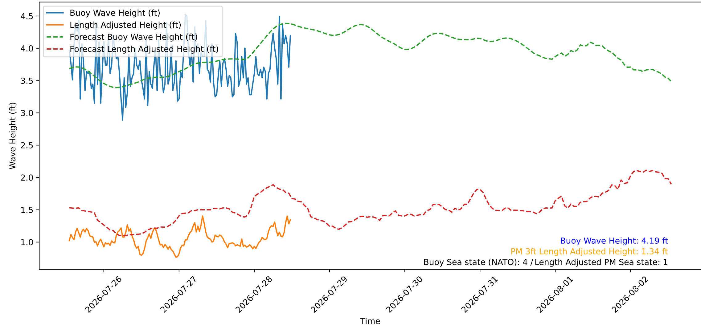
Wave Heights over Time for Red Beach at 2026-07-28 12:30:46
