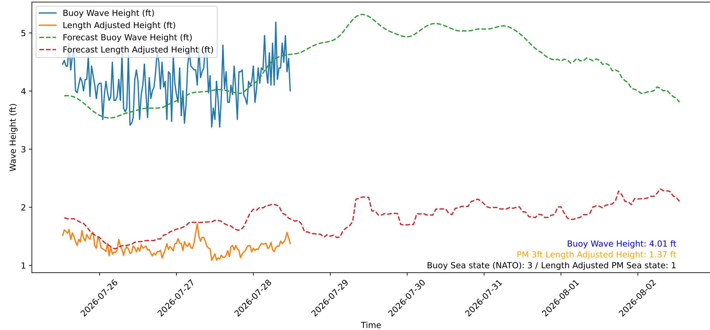
Wave Heights over Time for Green Beach at 2026-07-28 12:31:08
