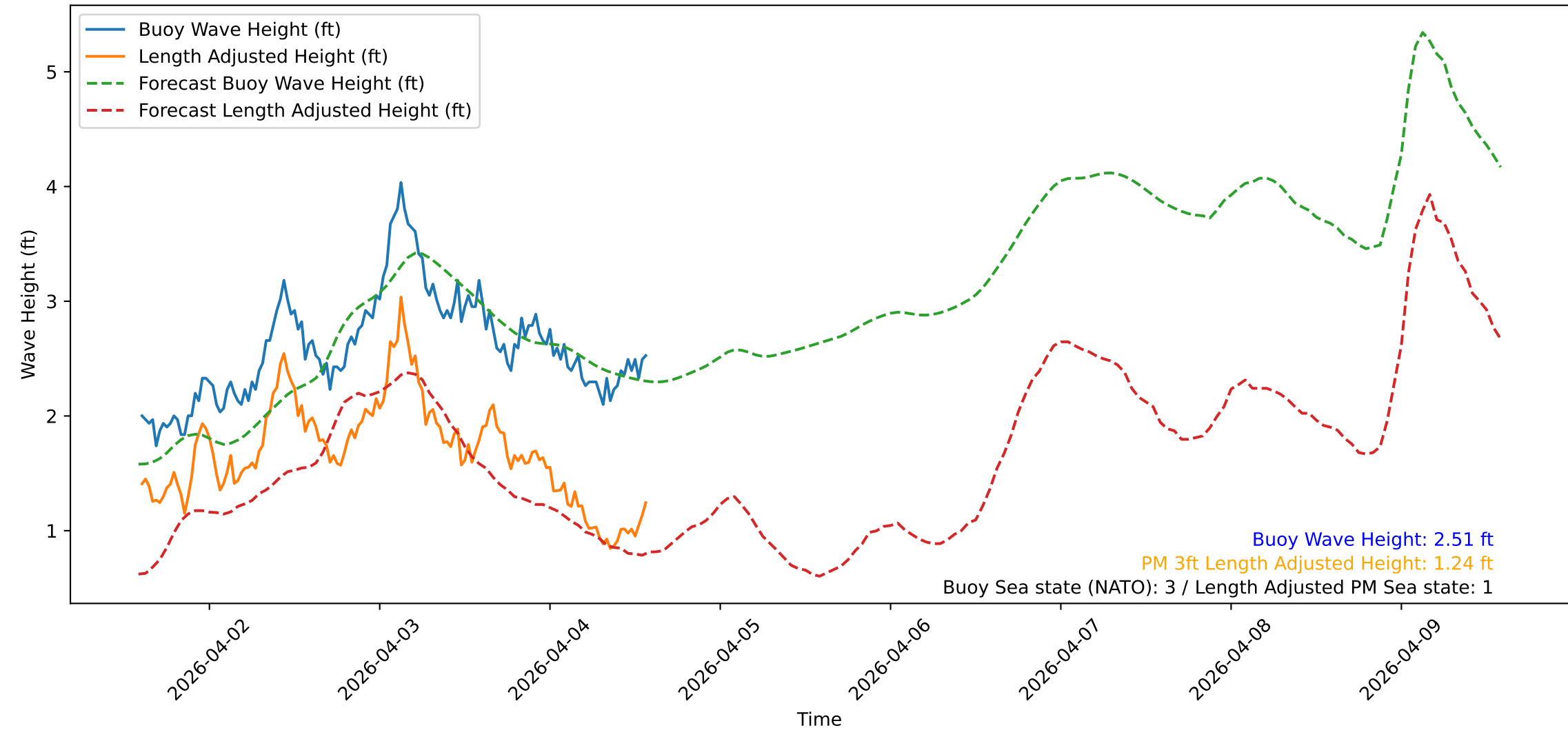
Wave Heights over Time for Oceanside Harbor at 2026-04-04 14:20:31
