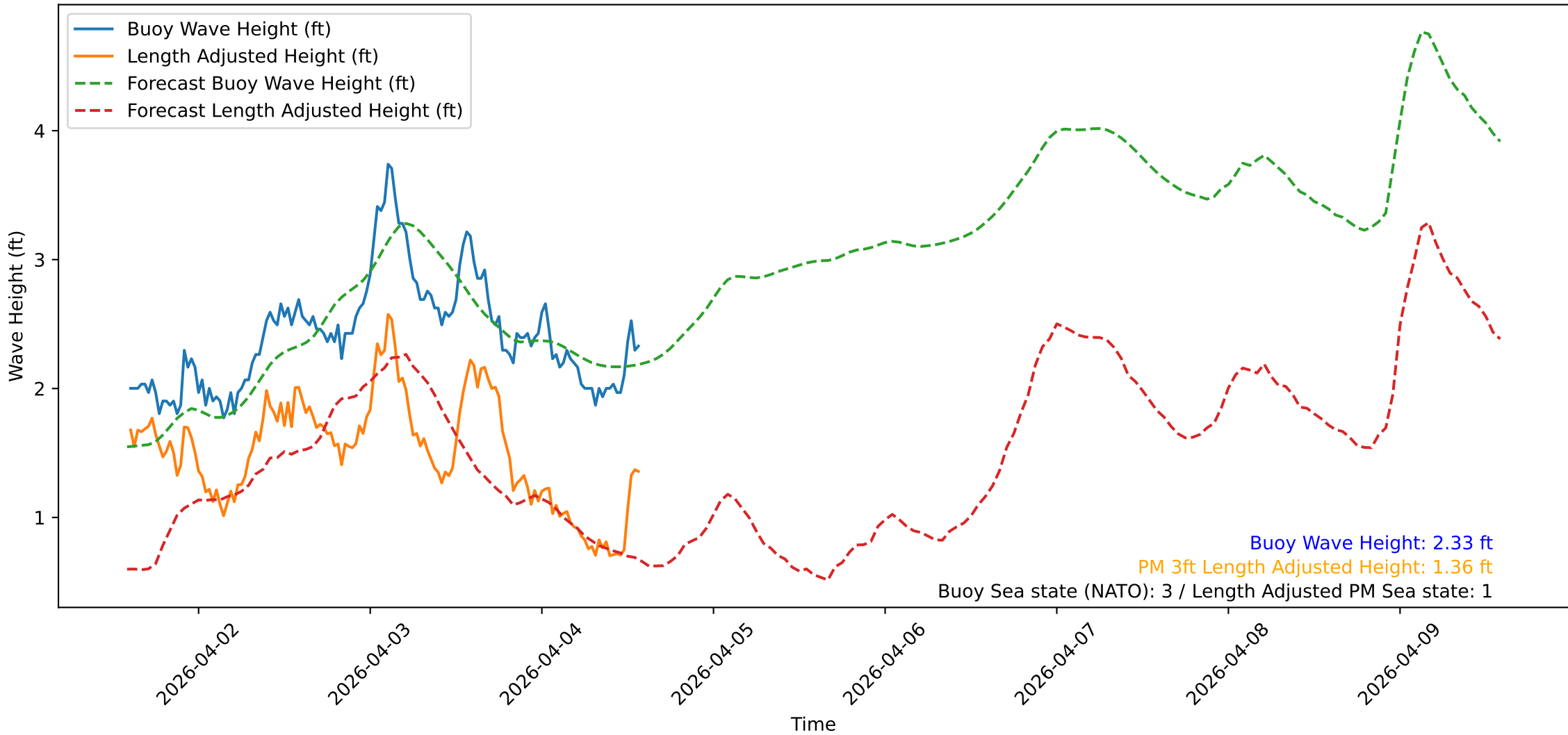
Wave Heights over Time for Red Beach at 2026-04-04 14:20:47
