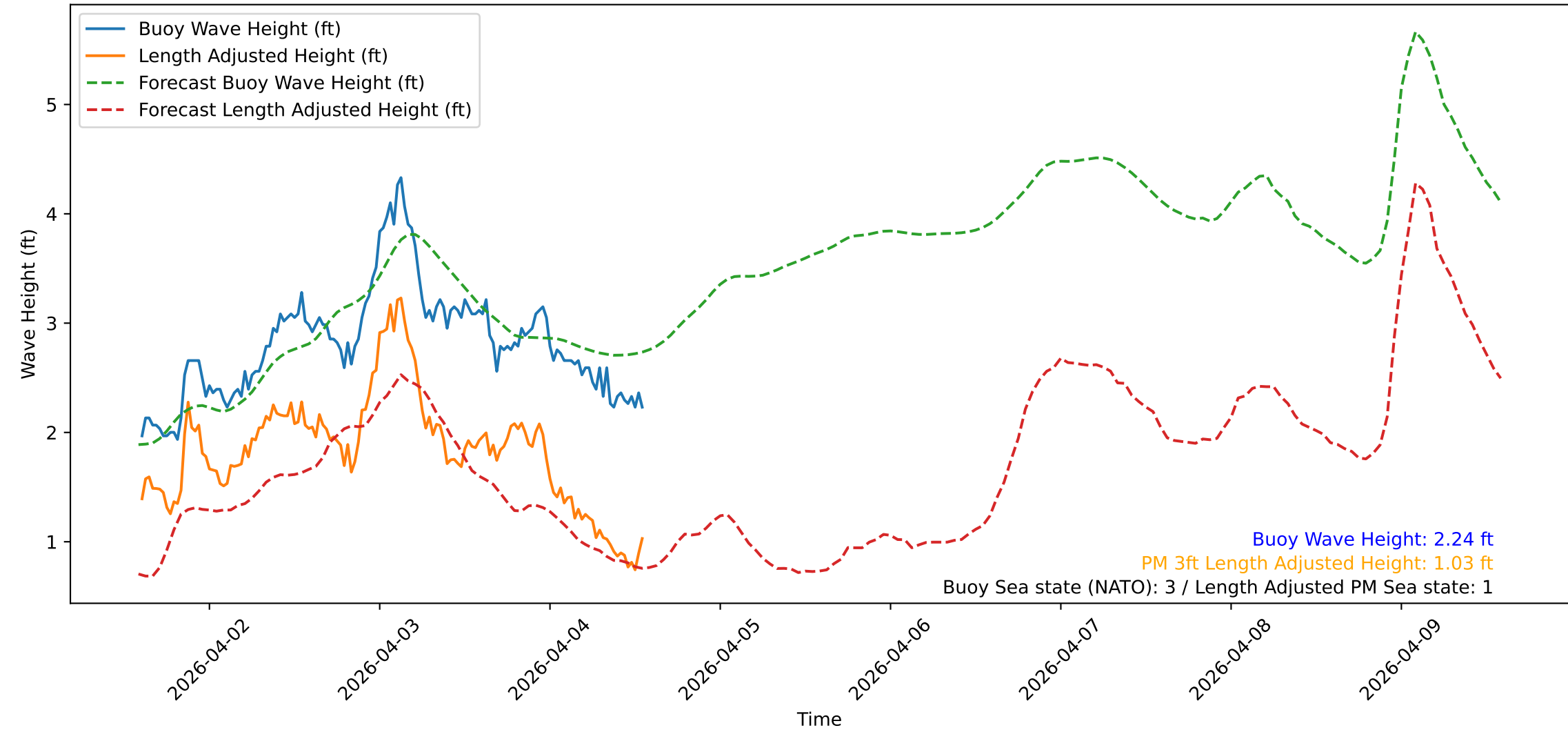
Wave Heights over Time for Green Beach at 2026-04-04 14:21:09
