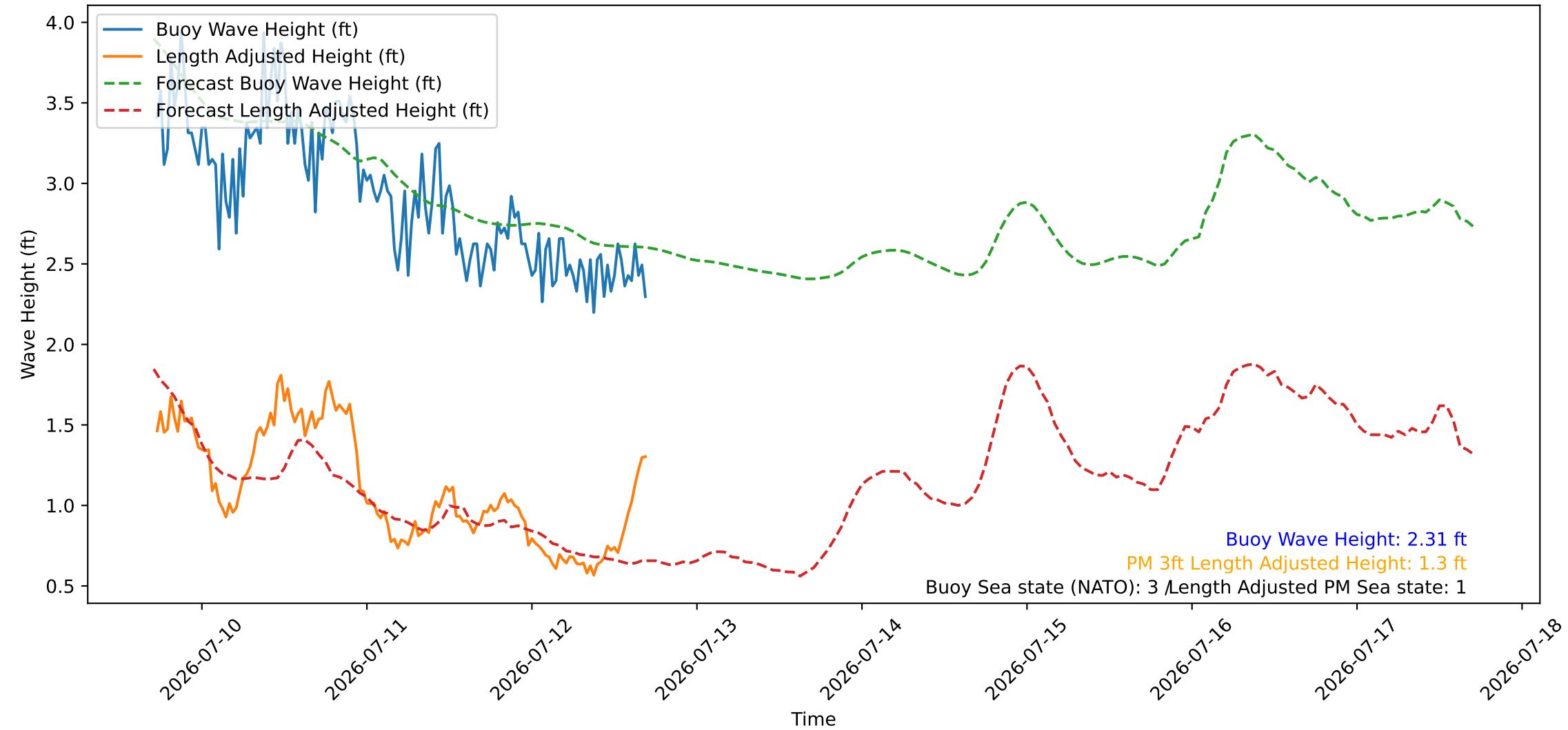
Wave Heights over Time for Red Beach at 2026-07-12 17:10:45
