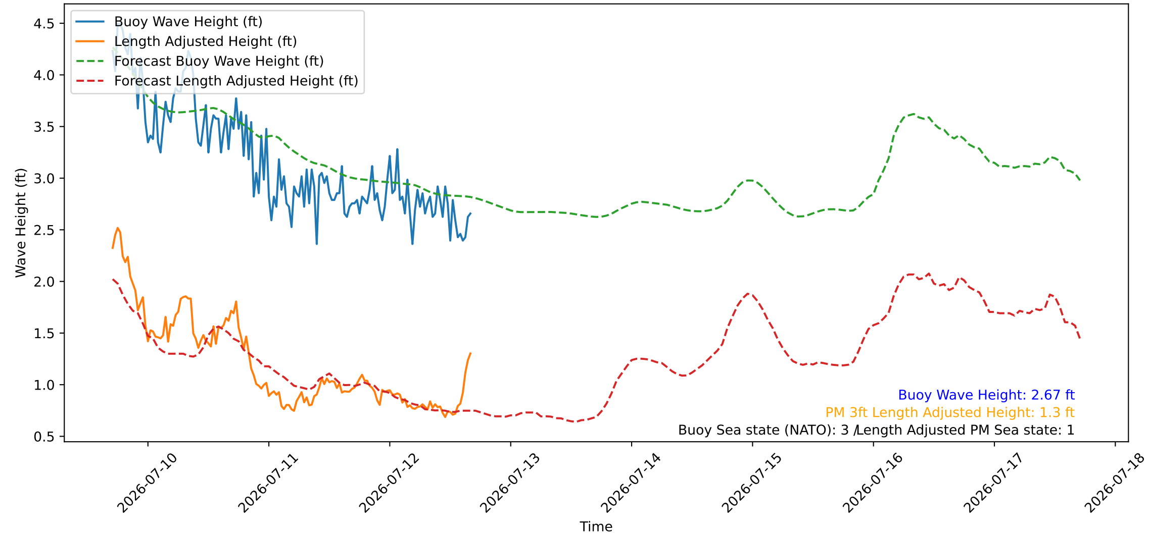
Wave Heights over Time for Oceanside Harbor at 2026-07-12 17:10:26
