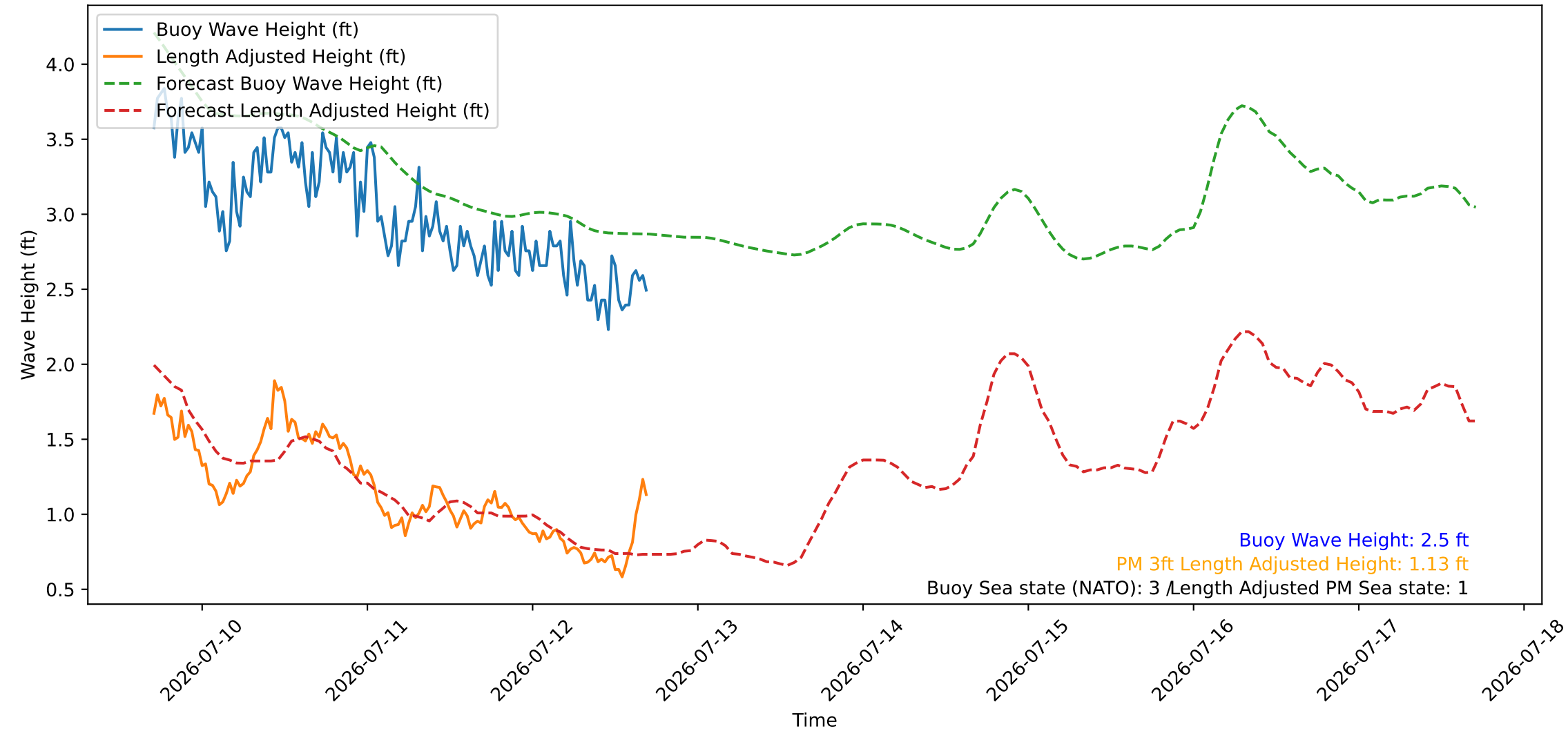
Wave Heights over Time for Green Beach at 2026-07-12 17:11:07
