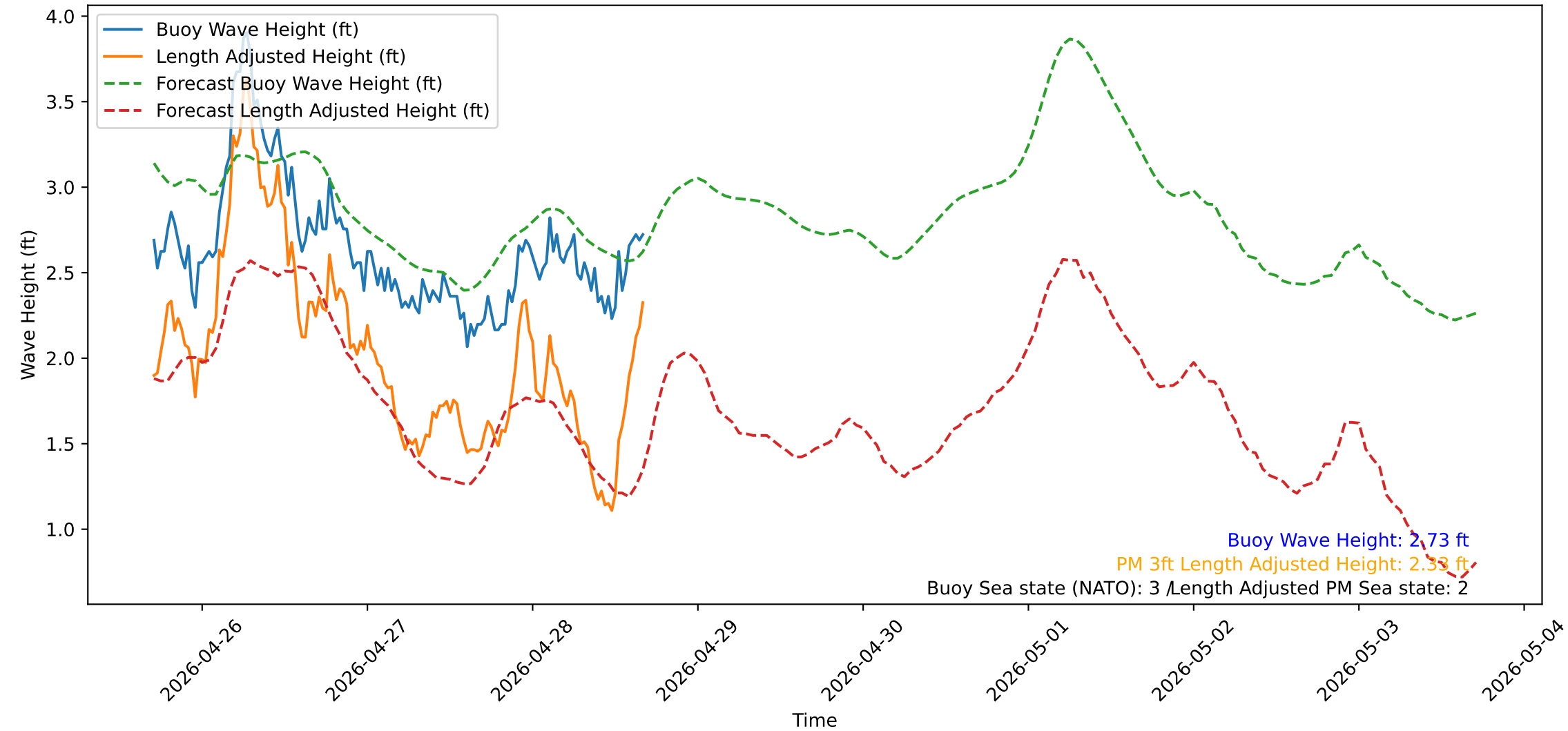
Wave Heights over Time for Oceanside Harbor at 2026-04-28 17:00:31
