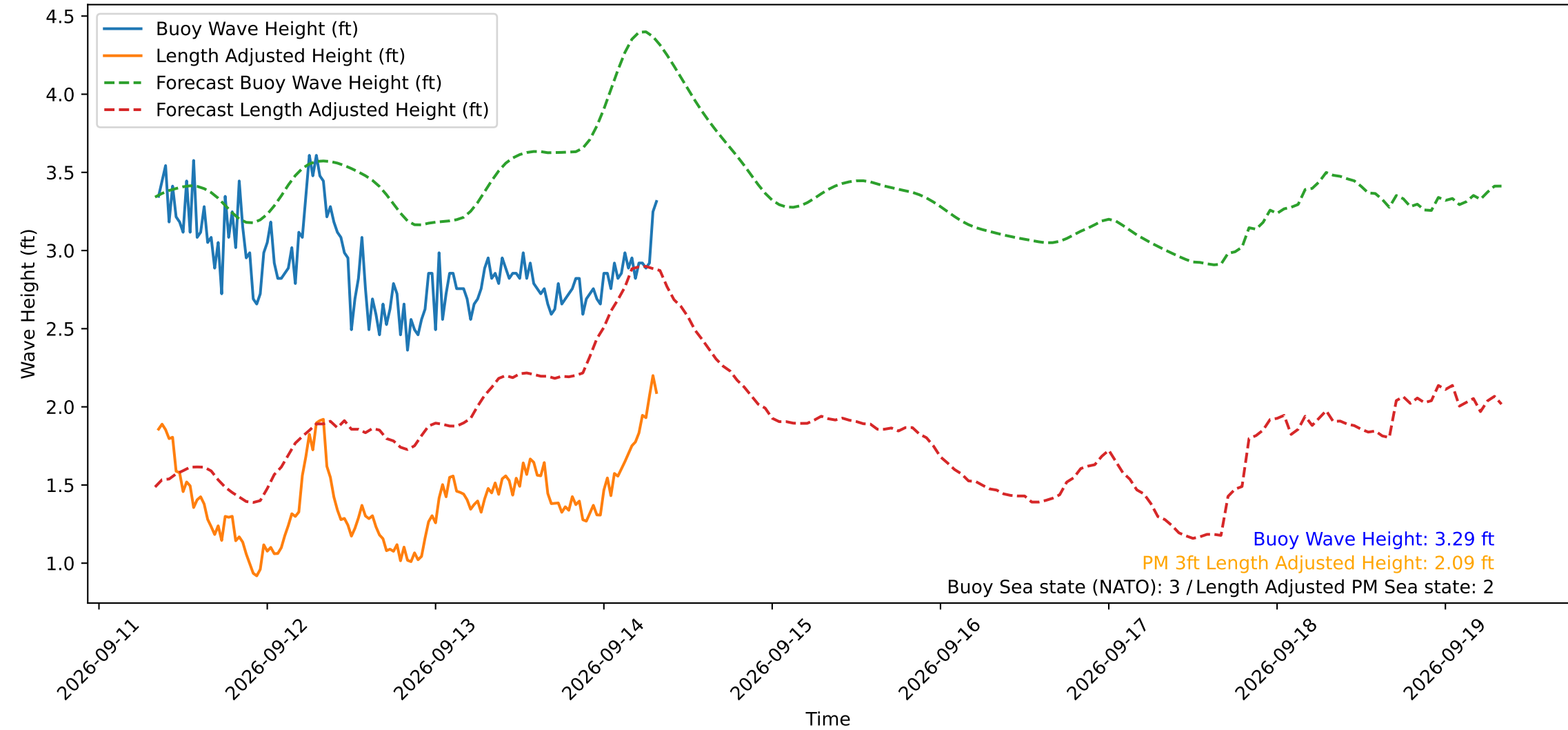
Wave Heights over Time for Green Beach at 2026-09-14 08:21:14
