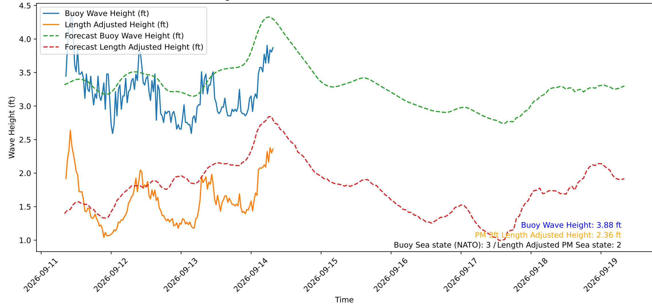
Wave Heights over Time for Oceanside Harbor at 2026-09-14 08:20:29
