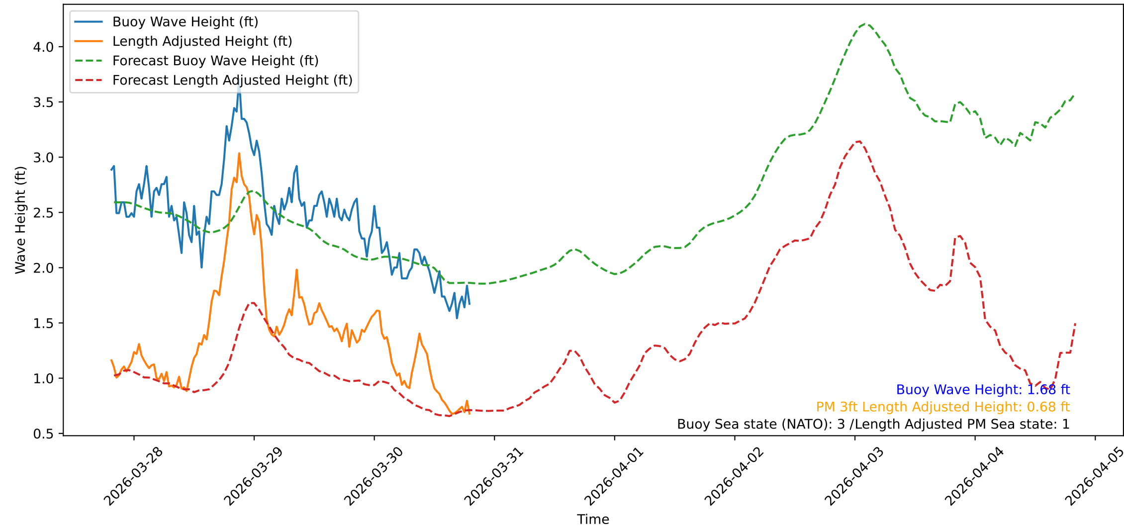
Wave Heights over Time for Green Beach at 2026-03-30 19:41:08
