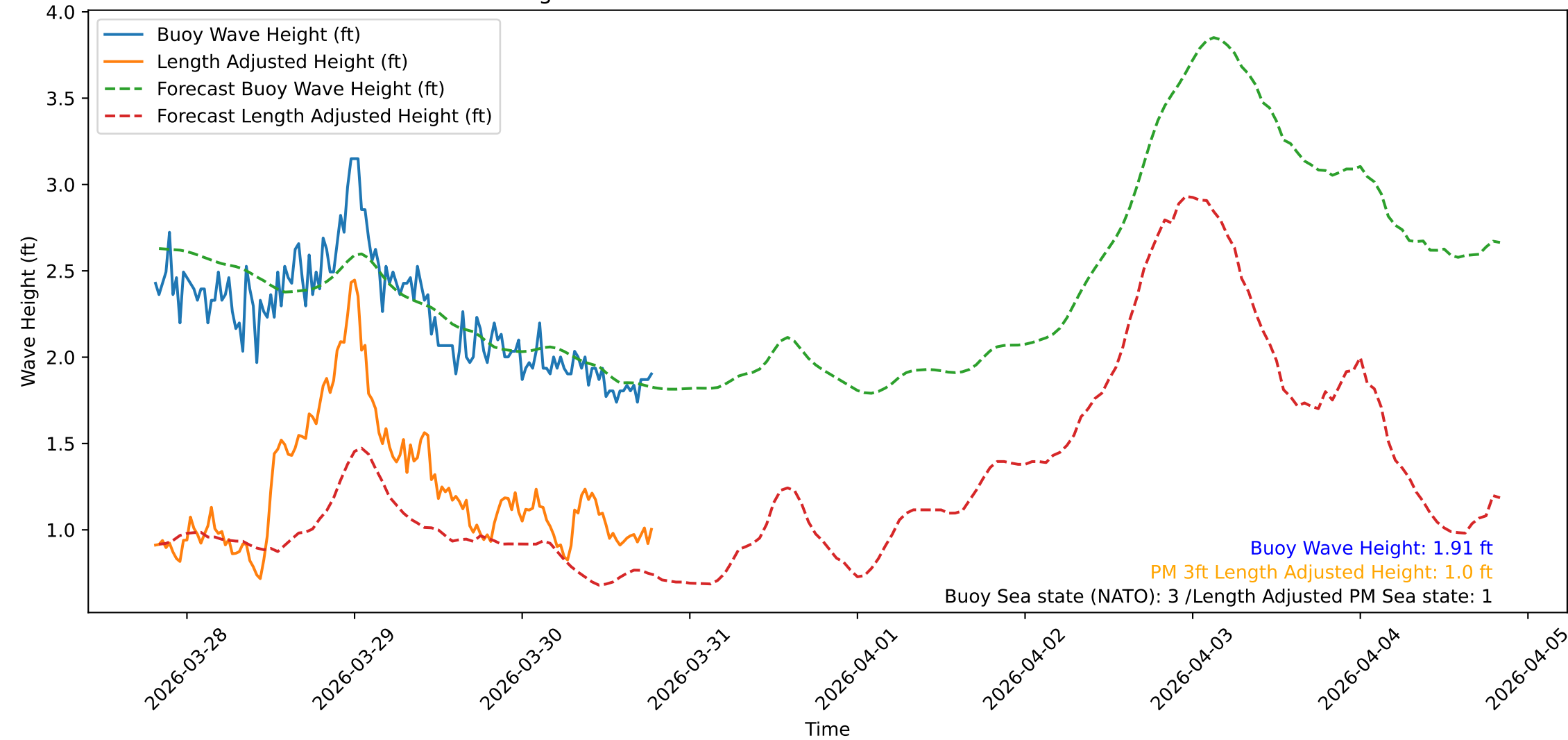
Wave Heights over Time for Oceanside Harbor at 2026-03-30 19:40:30
