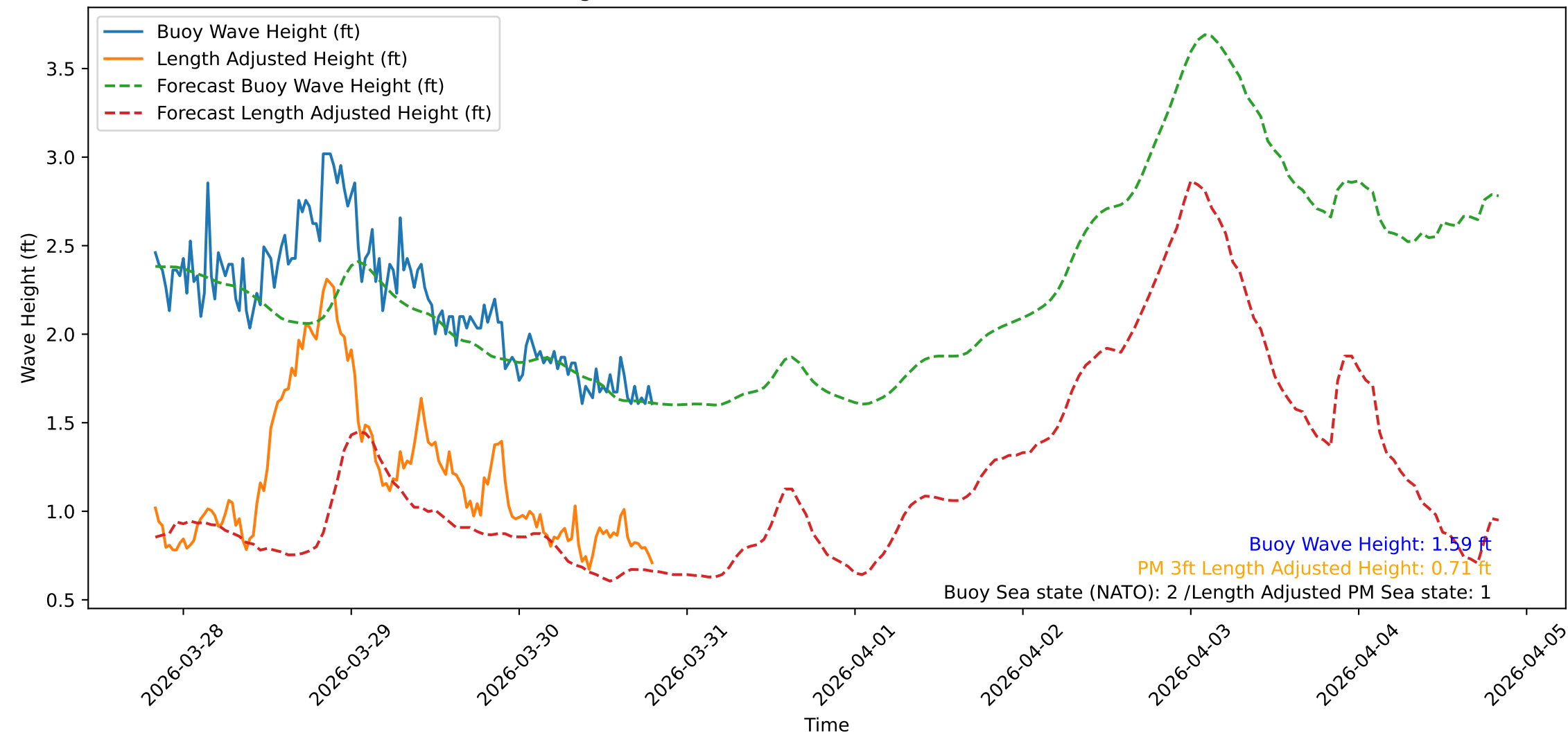
Wave Heights over Time for Red Beach at 2026-03-30 19:40:46
