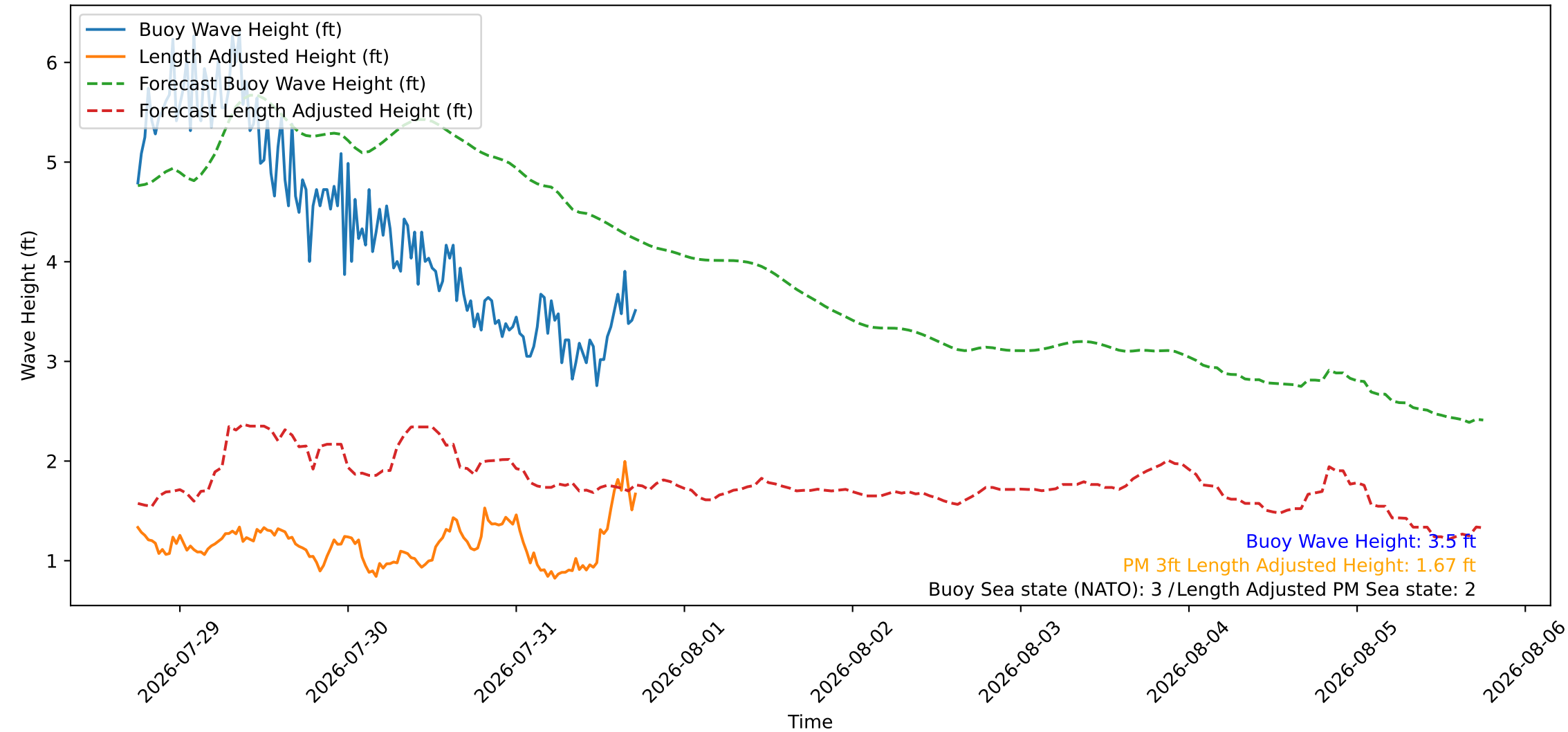
Wave Heights over Time for Green Beach at 2026-07-31 18:01:09
