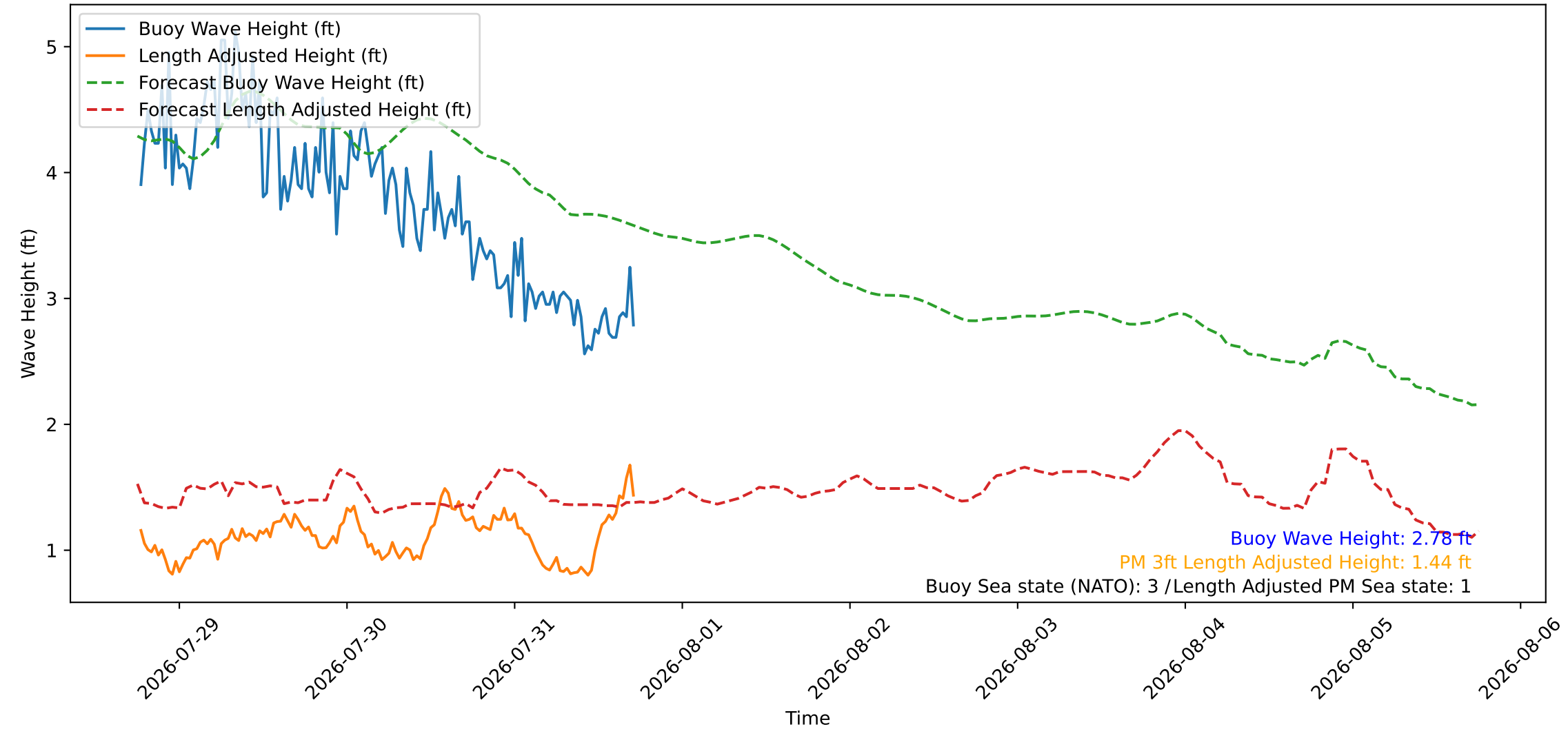
Wave Heights over Time for Red Beach at 2026-07-31 18:00:45
