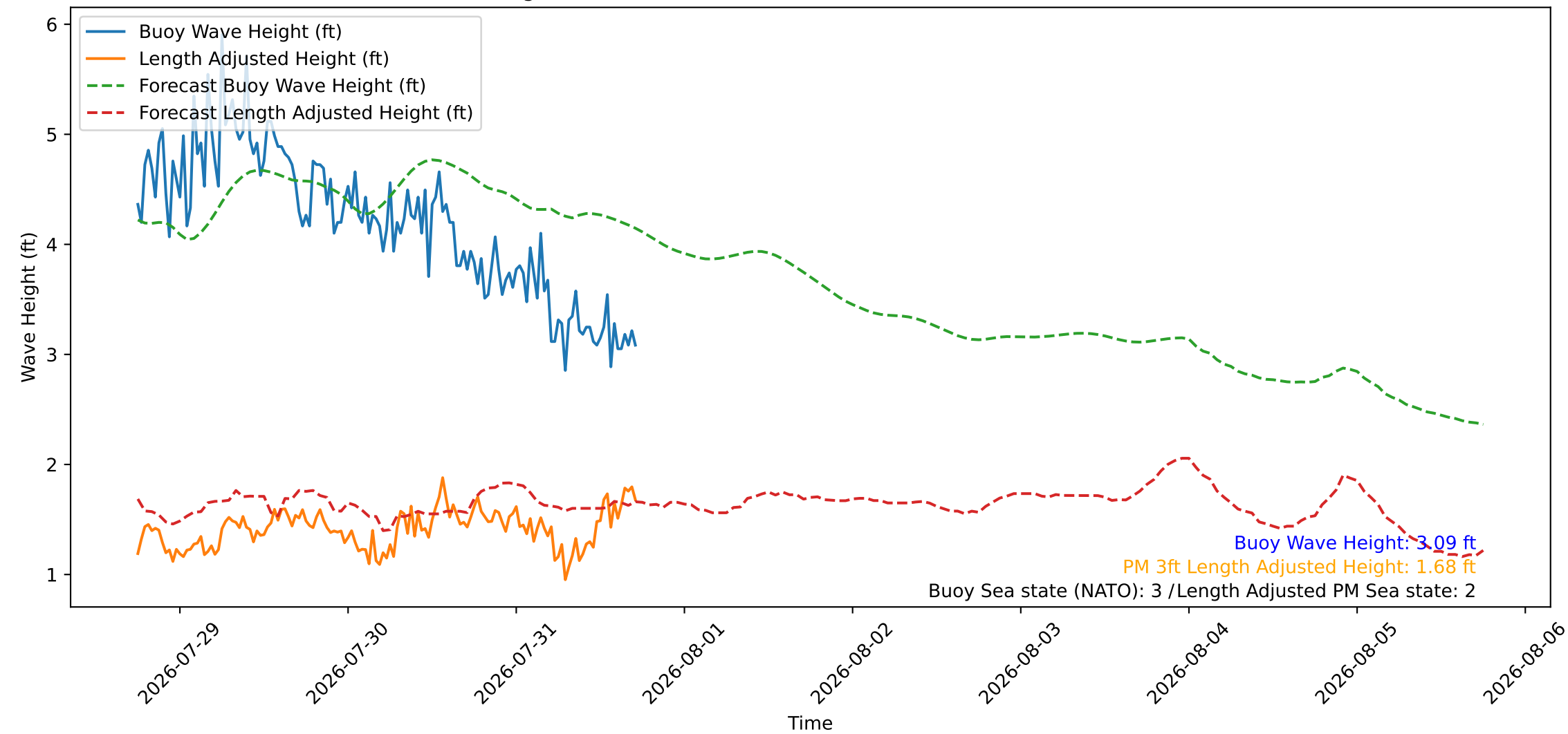
Wave Heights over Time for Oceanside Harbor at 2026-07-31 18:00:26
