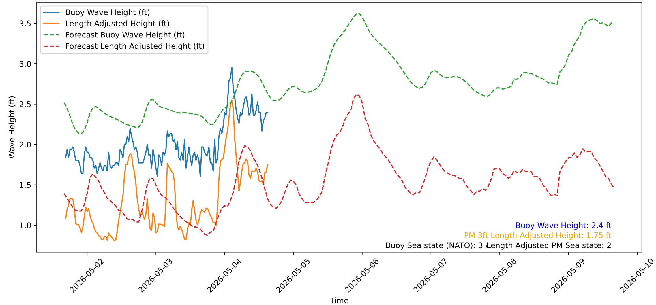
Wave Heights over Time for Red Beach at 2026-05-04 16:20:52
