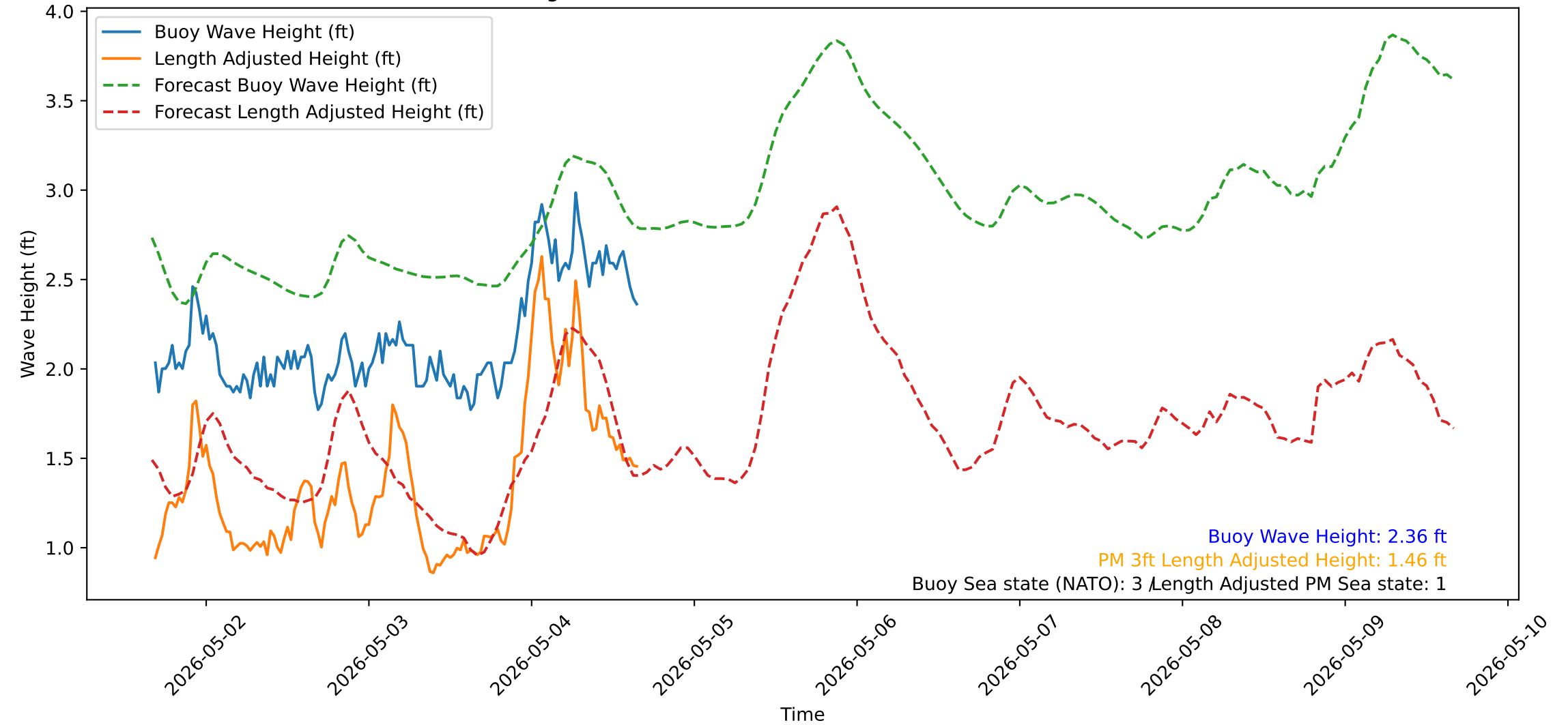
Wave Heights over Time for Green Beach at 2026-05-04 16:21:14
