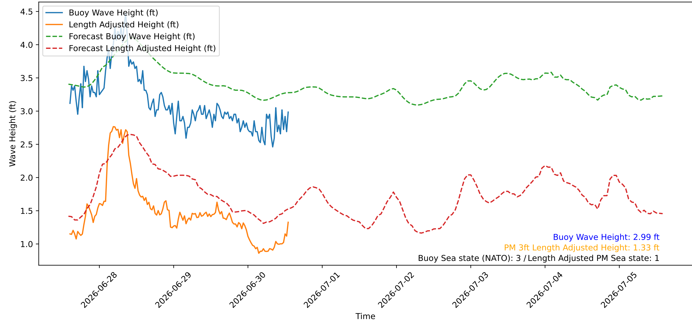
Wave Heights over Time for Red Beach at 2026-06-30 14:00:45
