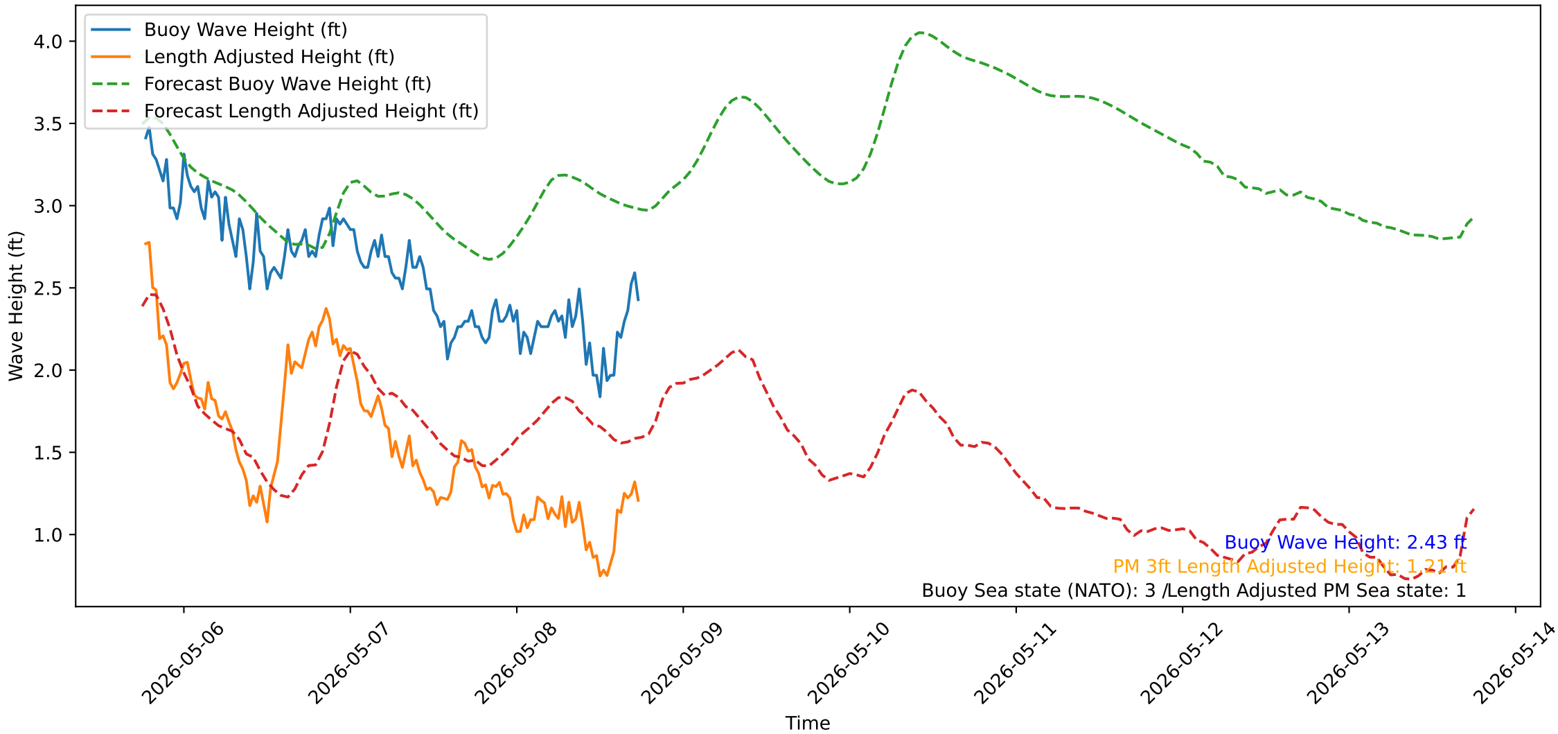
Wave Heights over Time for Green Beach at 2026-05-08 18:21:13
