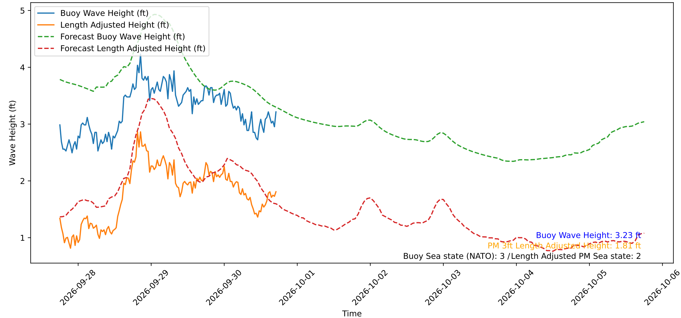
Wave Heights over Time for Oceanside Harbor at 2026-09-30 18:00:30
