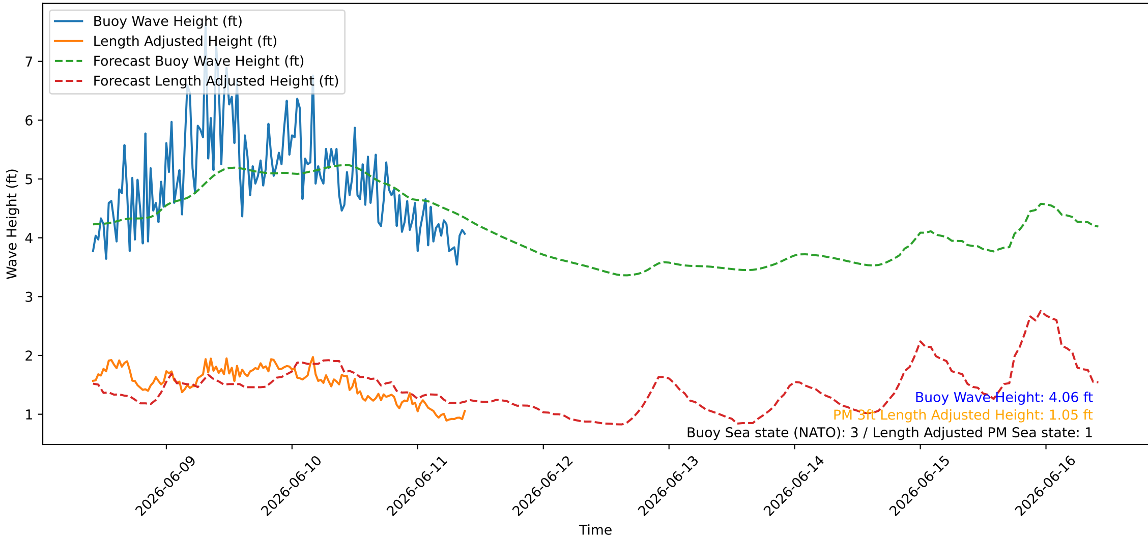
Wave Heights over Time for Red Beach at 2026-06-11 09:50:47
