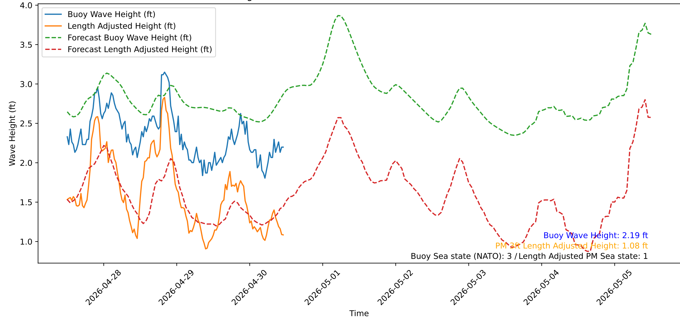
Wave Heights over Time for Green Beach at 2026-04-30 11:51:14
