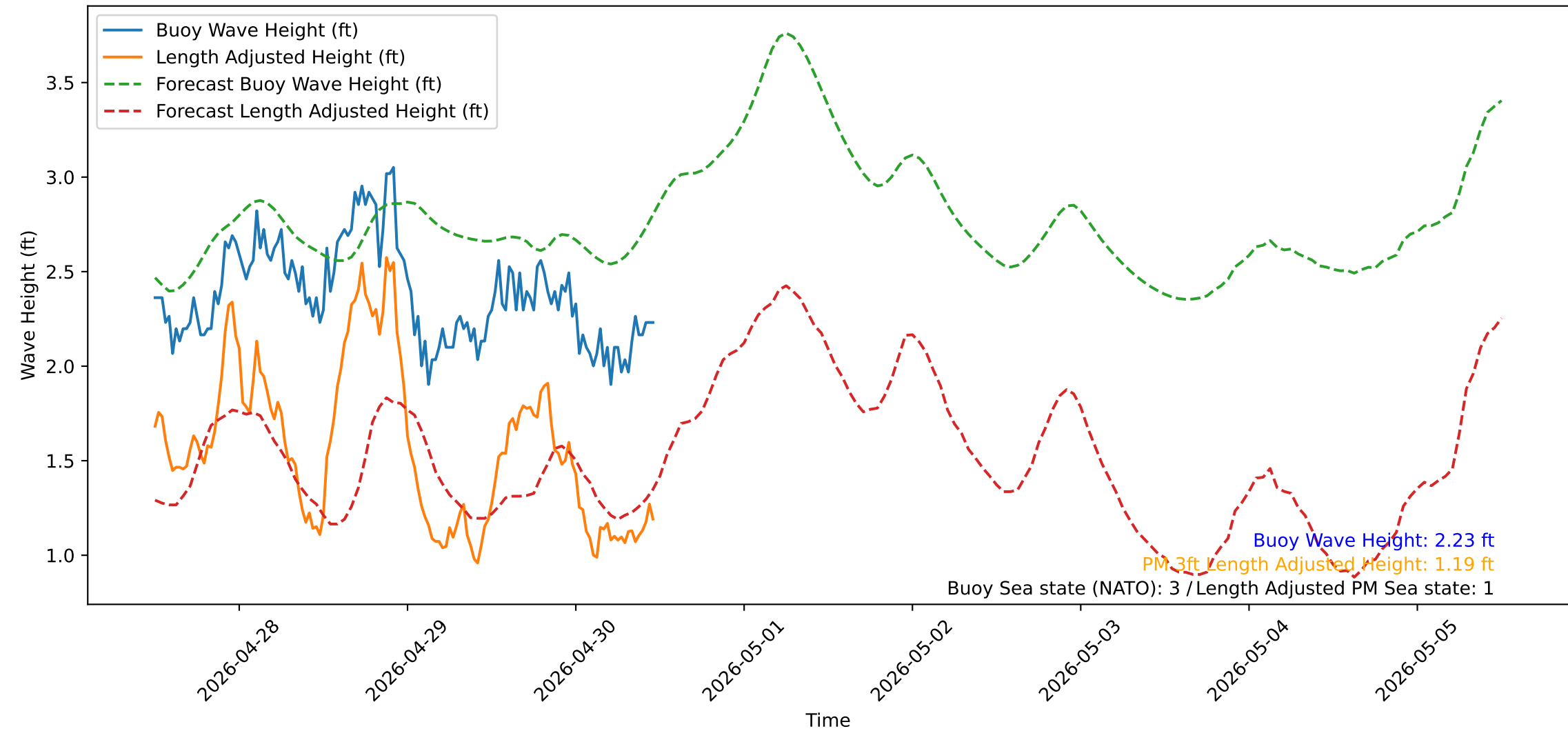
Wave Heights over Time for Oceanside Harbor at 2026-04-30 11:50:31
