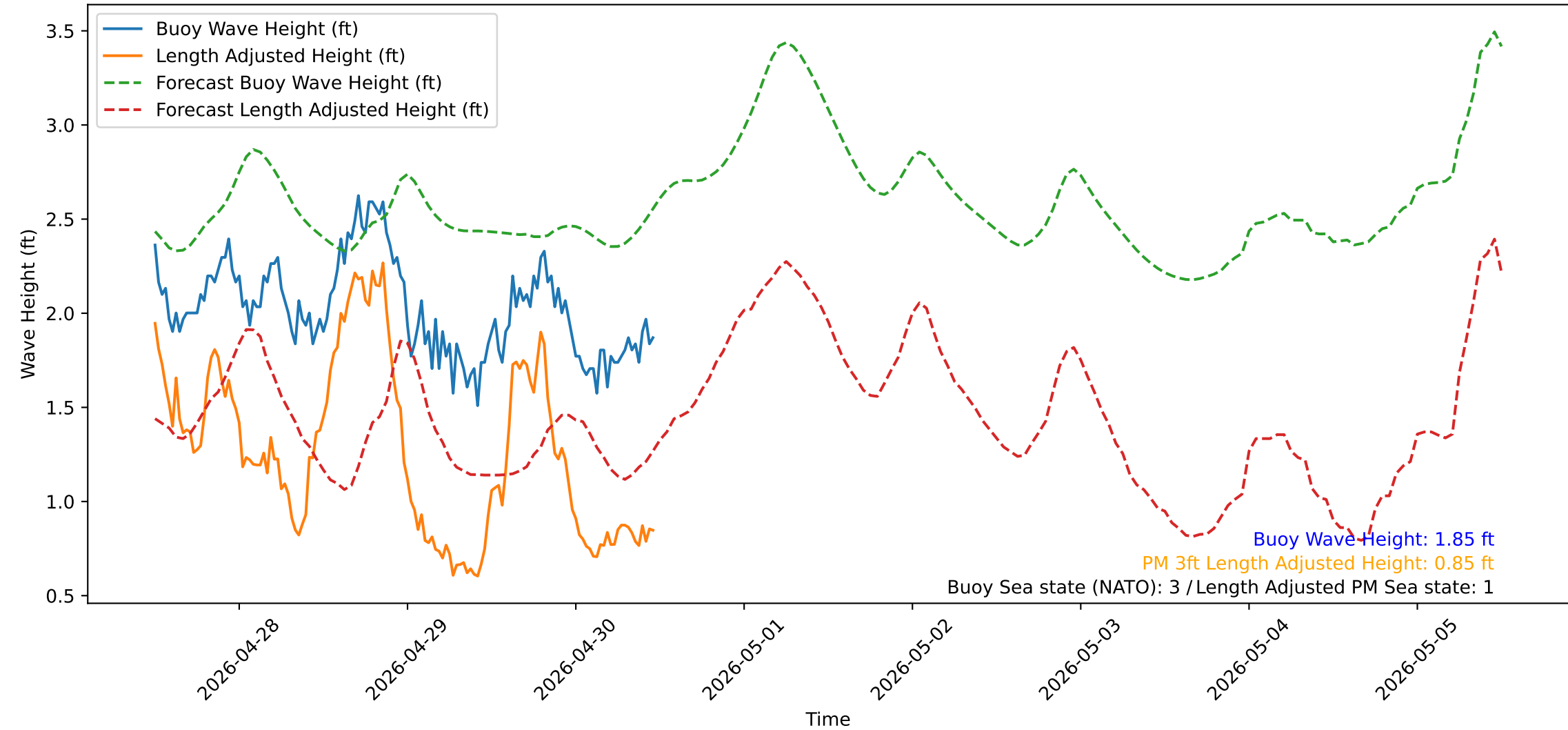
Wave Heights over Time for Red Beach at 2026-04-30 11:50:51
