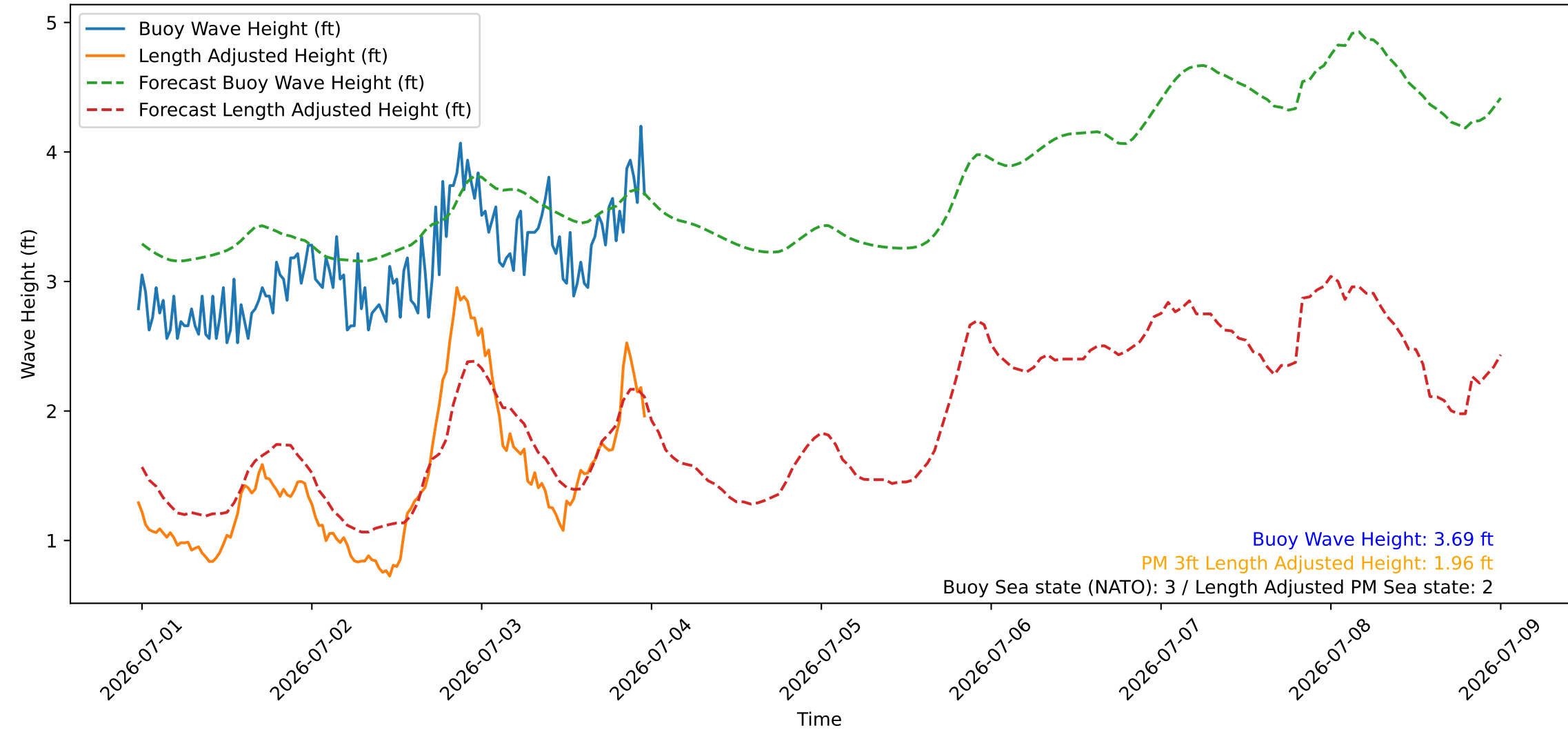
Wave Heights over Time for Green Beach at 2026-07-03 23:41:10
