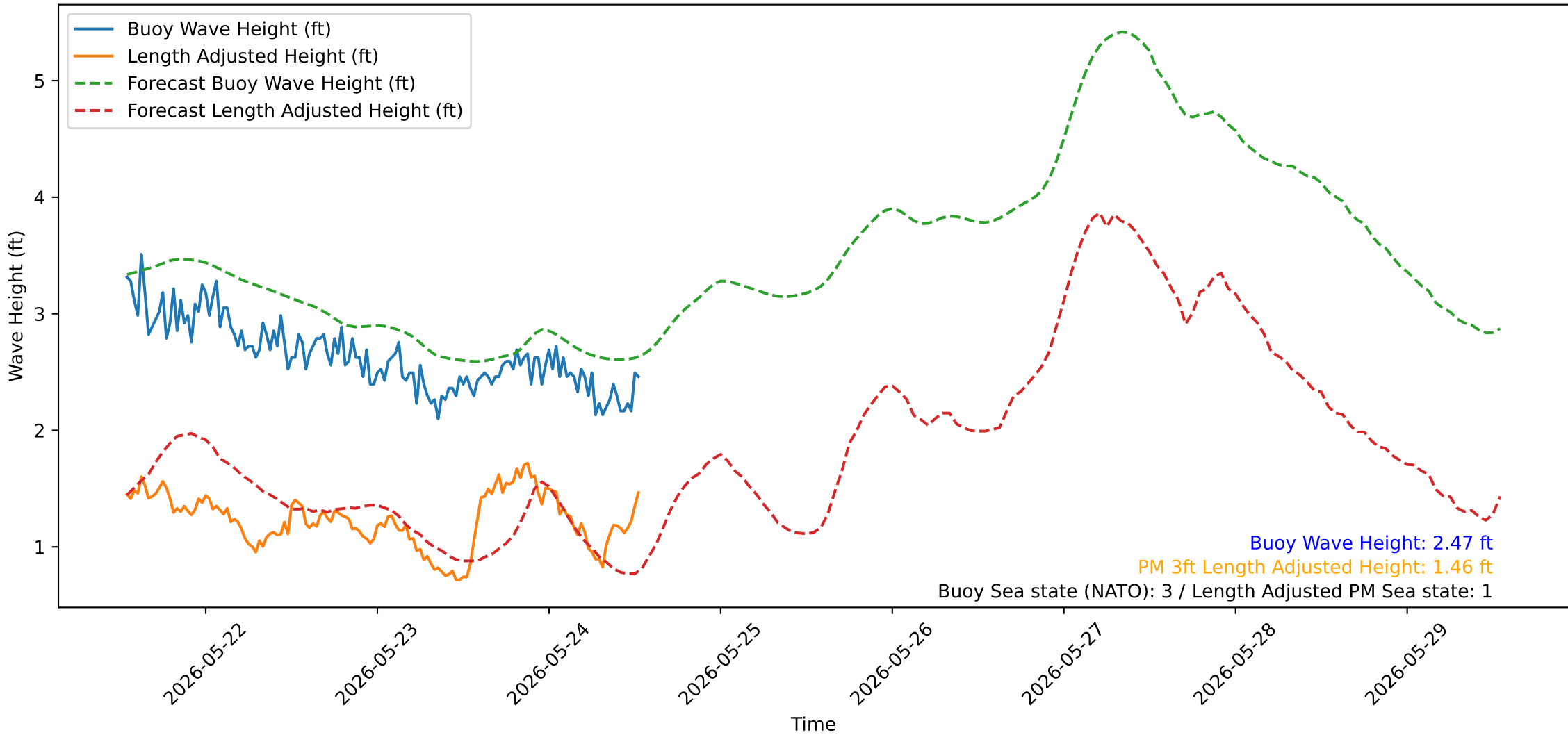
Wave Heights over Time for Oceanside Harbor at 2026-05-24 13:10:32
