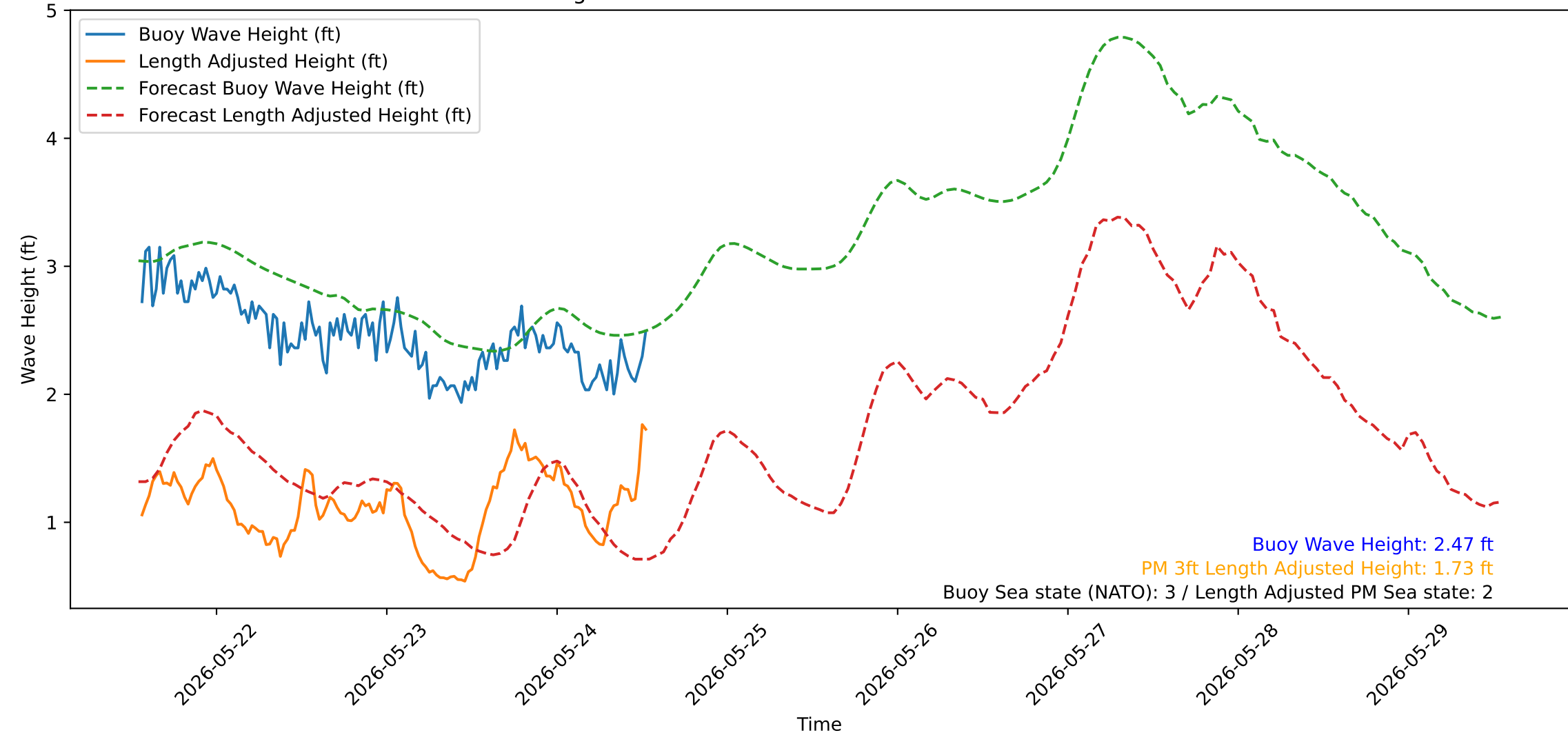
Wave Heights over Time for Red Beach at 2026-05-24 13:10:52
