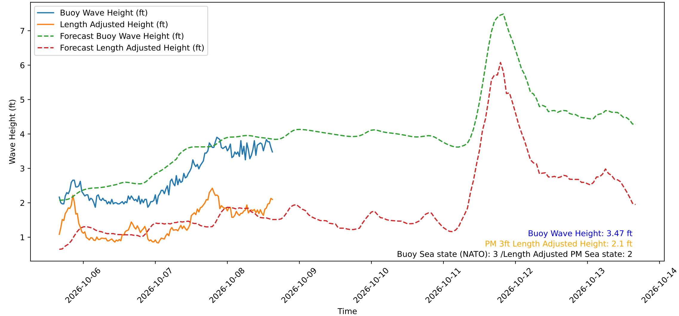
Wave Heights over Time for Red Beach at 2026-10-08 15:40:49
