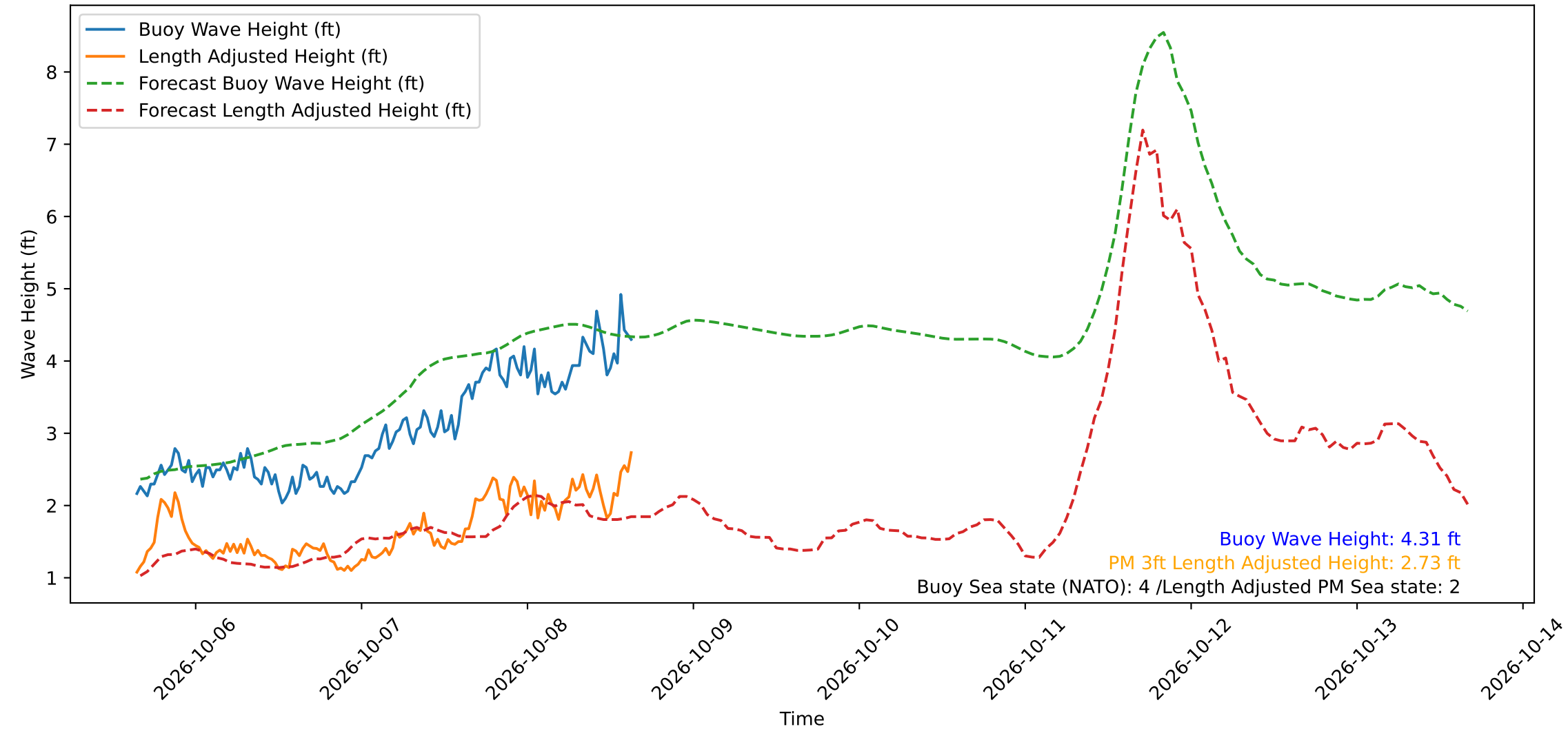
Wave Heights over Time for Oceanside Harbor at 2026-10-08 15:40:30
