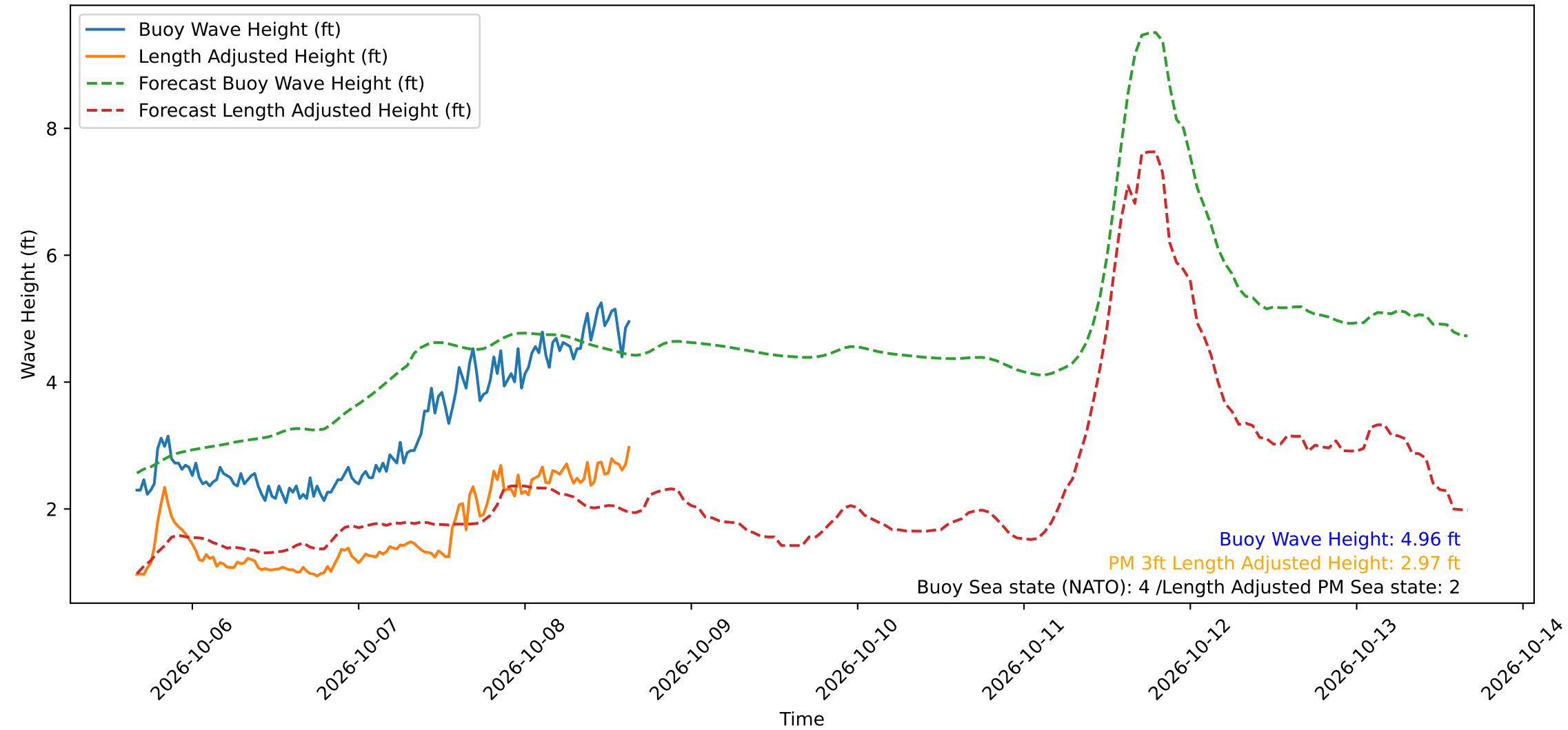
Wave Heights over Time for Green Beach at 2026-10-08 15:41:12
