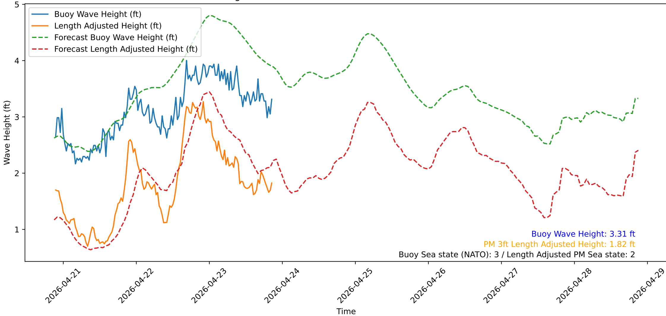
Wave Heights over Time for Green Beach at 2026-04-23 21:21:13
