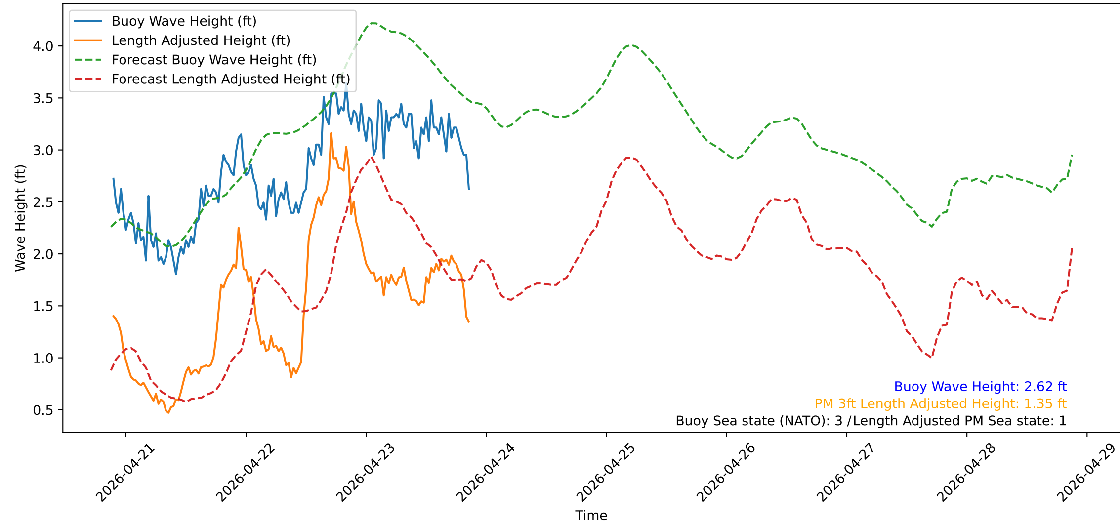
Wave Heights over Time for Red Beach at 2026-04-23 21:20:51
