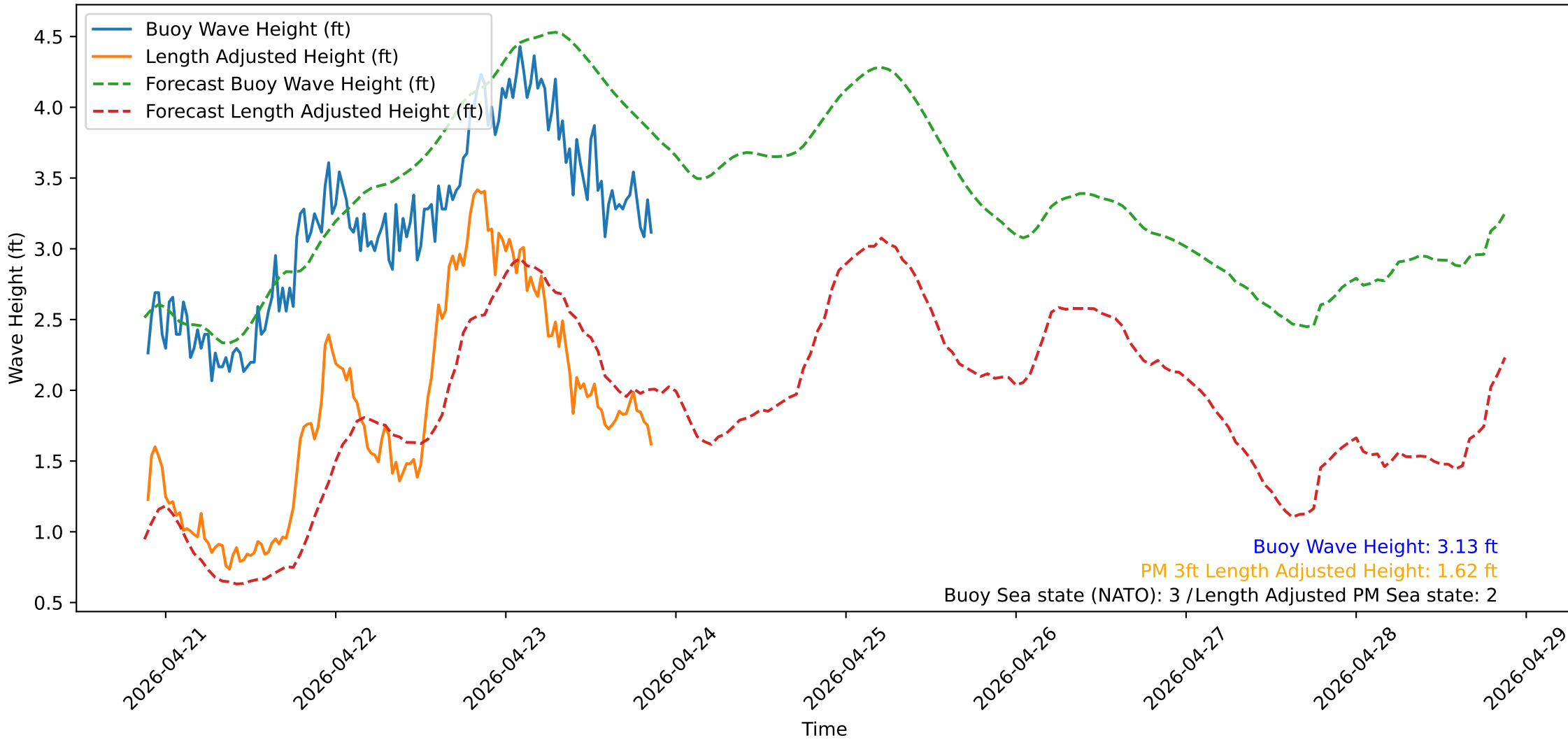
Wave Heights over Time for Oceanside Harbor at 2026-04-23 21:20:31
