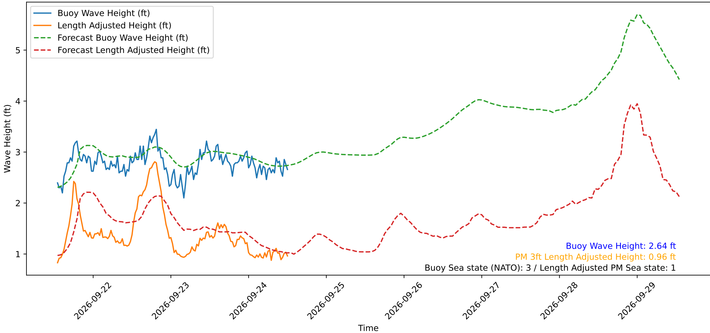
Wave Heights over Time for Green Beach at 2026-09-24 12:51:13
