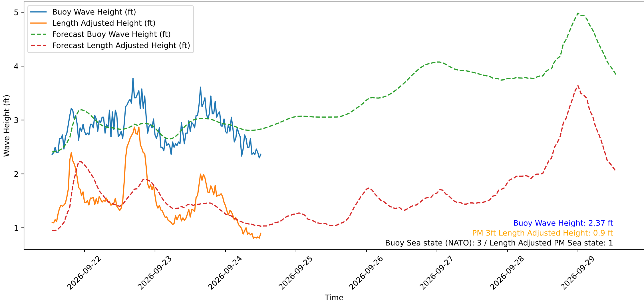
Wave Heights over Time for Oceanside Harbor at 2026-09-24 12:50:29
