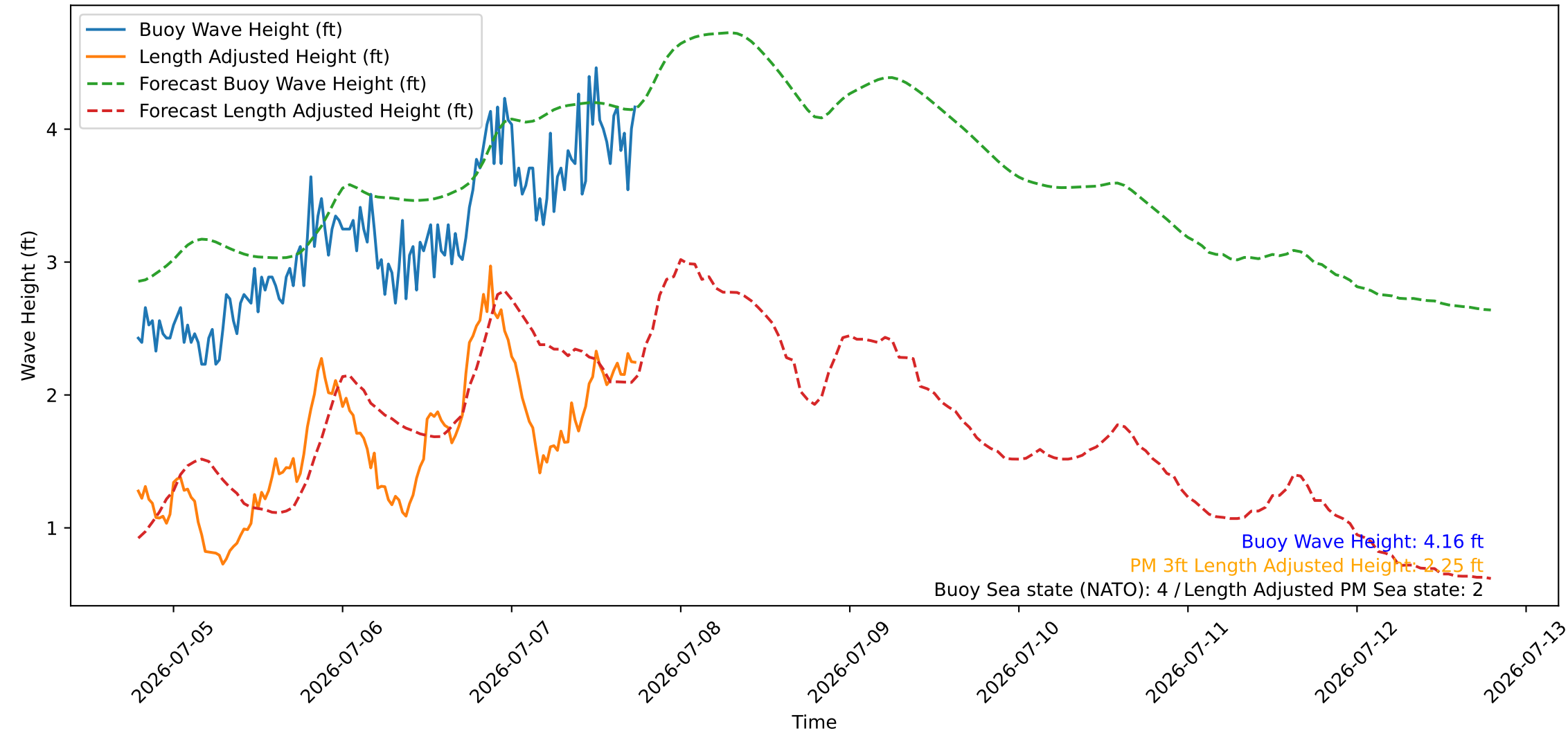
Wave Heights over Time for Red Beach at 2026-07-07 18:50:47
