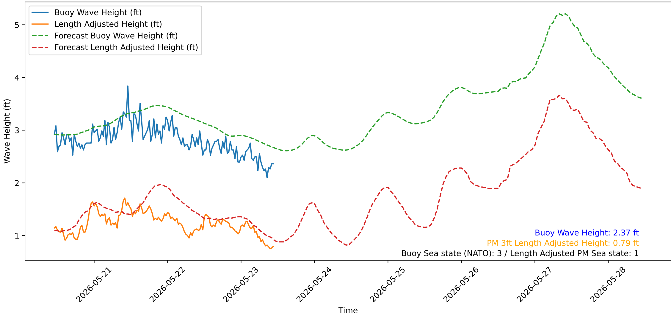
Wave Heights over Time for Oceanside Harbor at 2026-05-23 11:10:31
