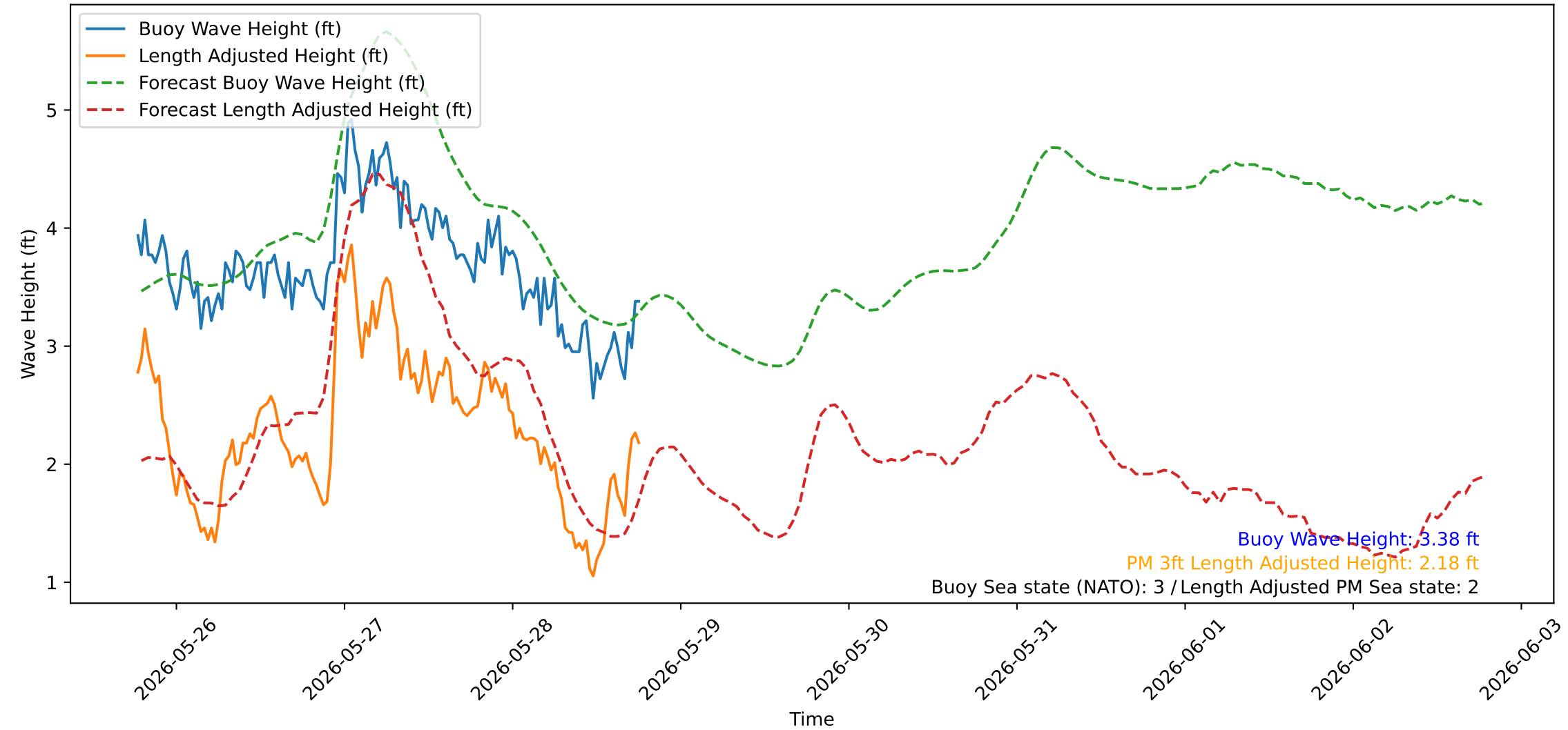
Wave Heights over Time for Green Beach at 2026-05-28 18:41:01
