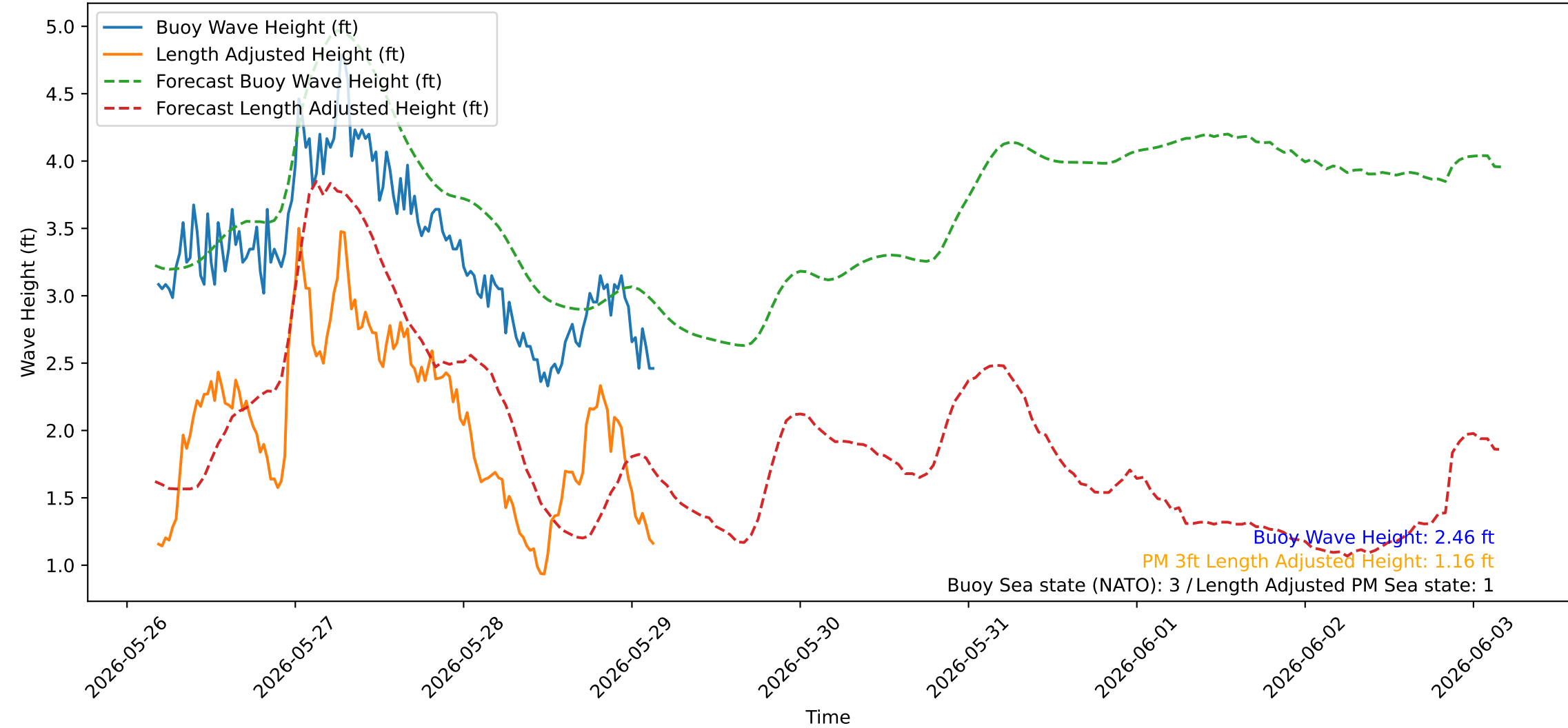
Wave Heights over Time for Red Beach at 2026-05-29 04:00:40
