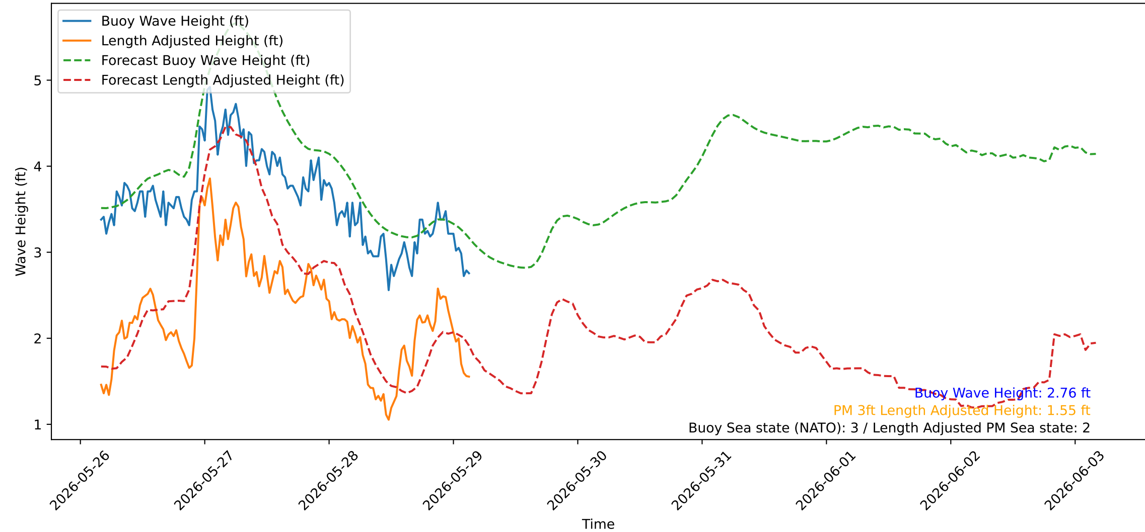
Wave Heights over Time for Green Beach at 2026-05-29 04:01:02
