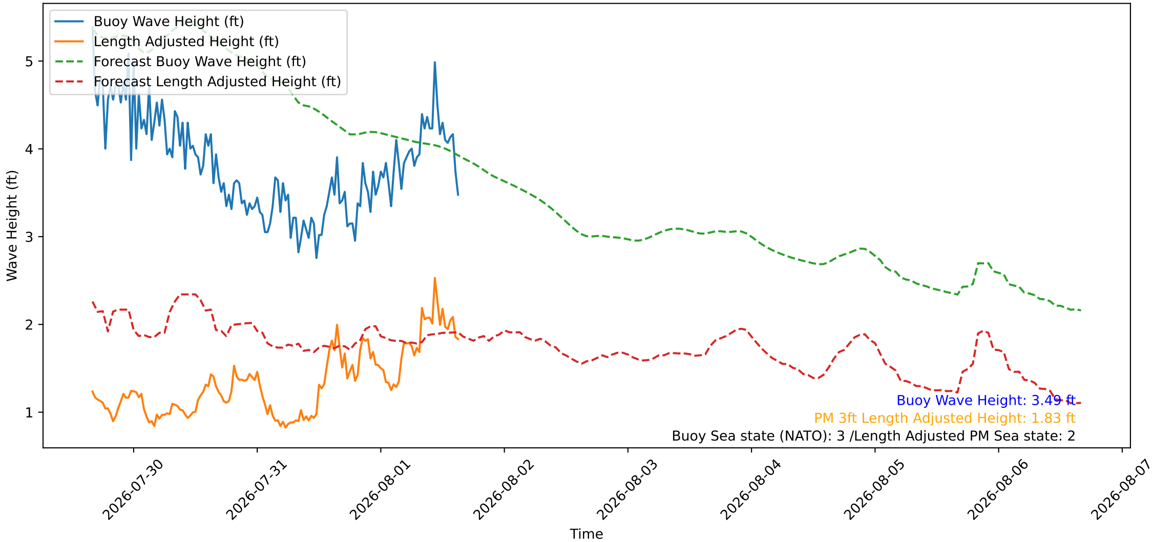
Wave Heights over Time for Green Beach at 2026-08-01 15:51:10
