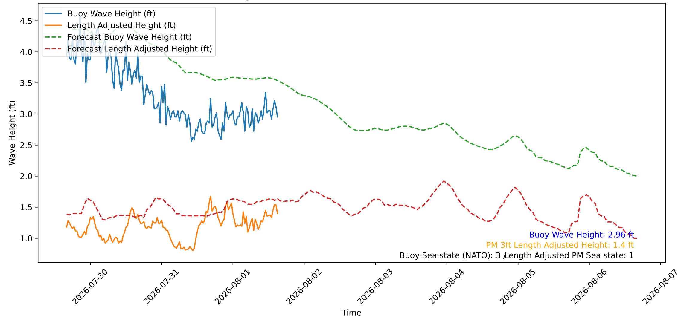
Wave Heights over Time for Red Beach at 2026-08-01 15:50:47
