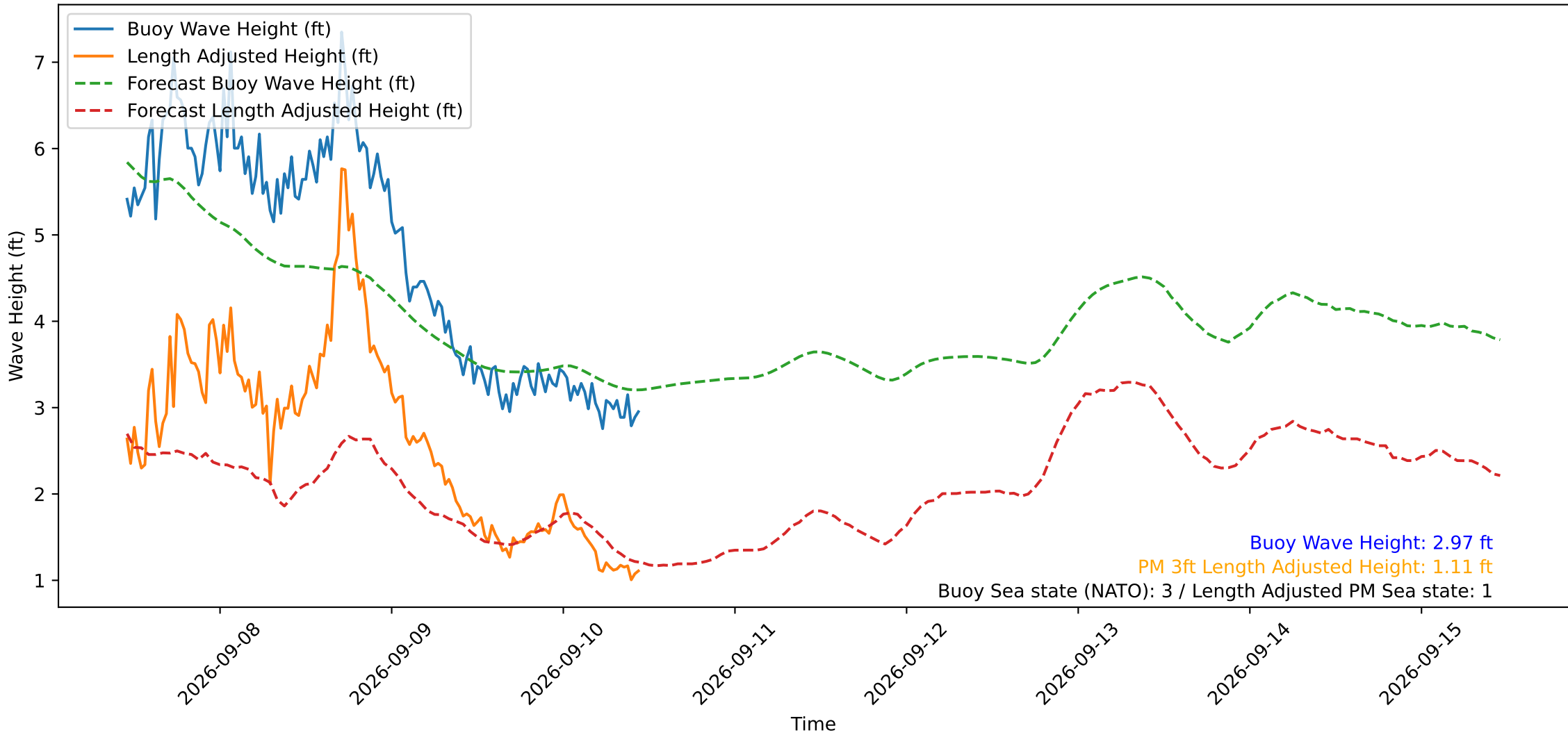
Wave Heights over Time for Oceanside Harbor at 2026-09-10 11:00:30
