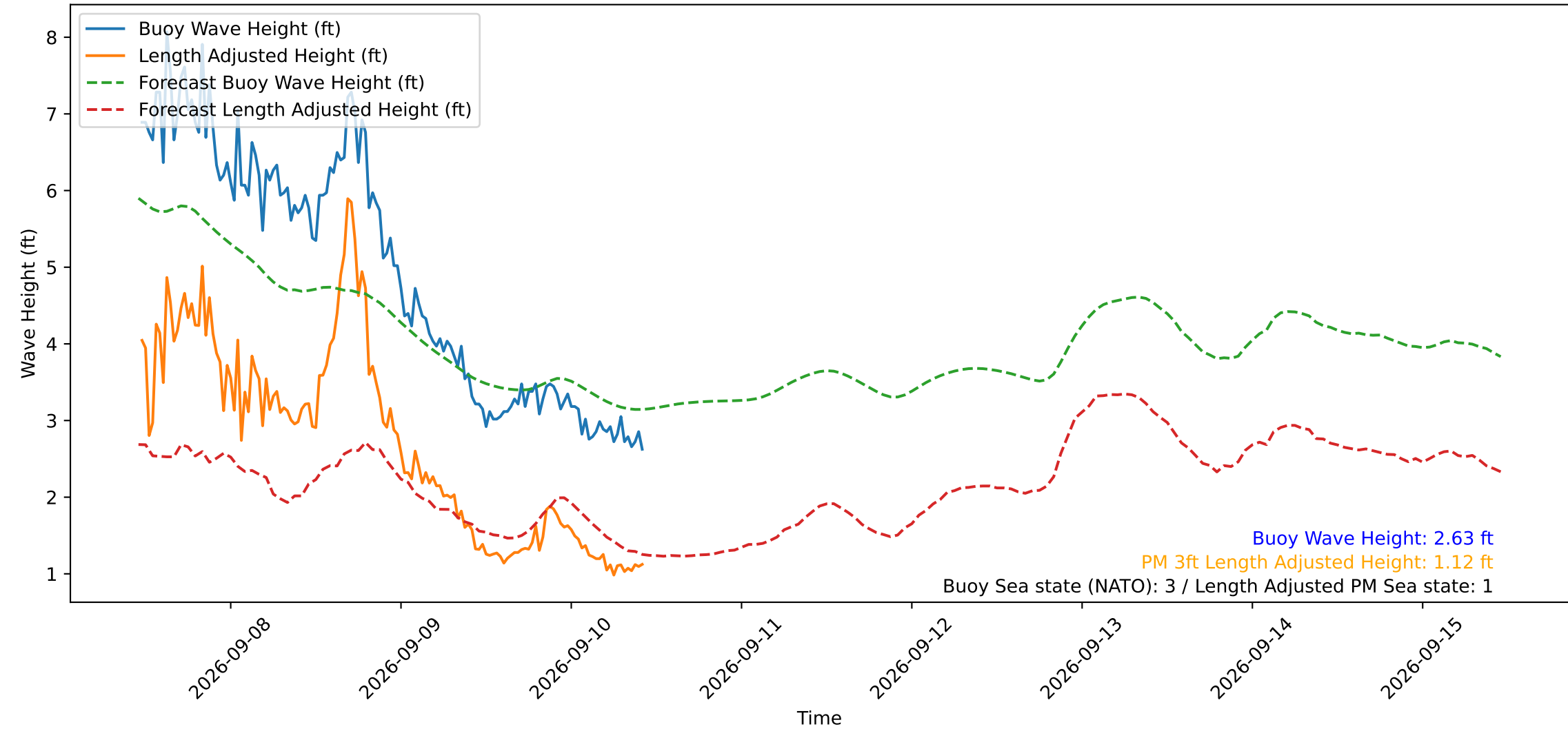
Wave Heights over Time for Green Beach at 2026-09-10 11:01:12
