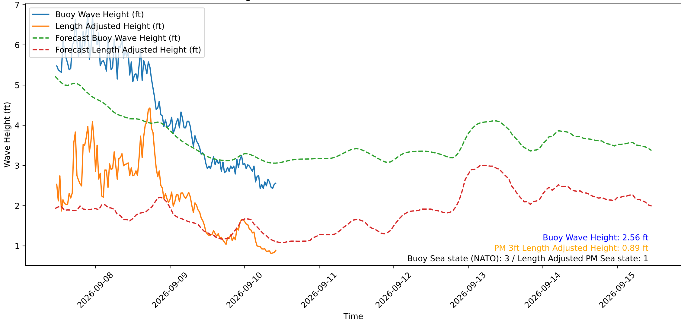
Wave Heights over Time for Red Beach at 2026-09-10 11:00:50
