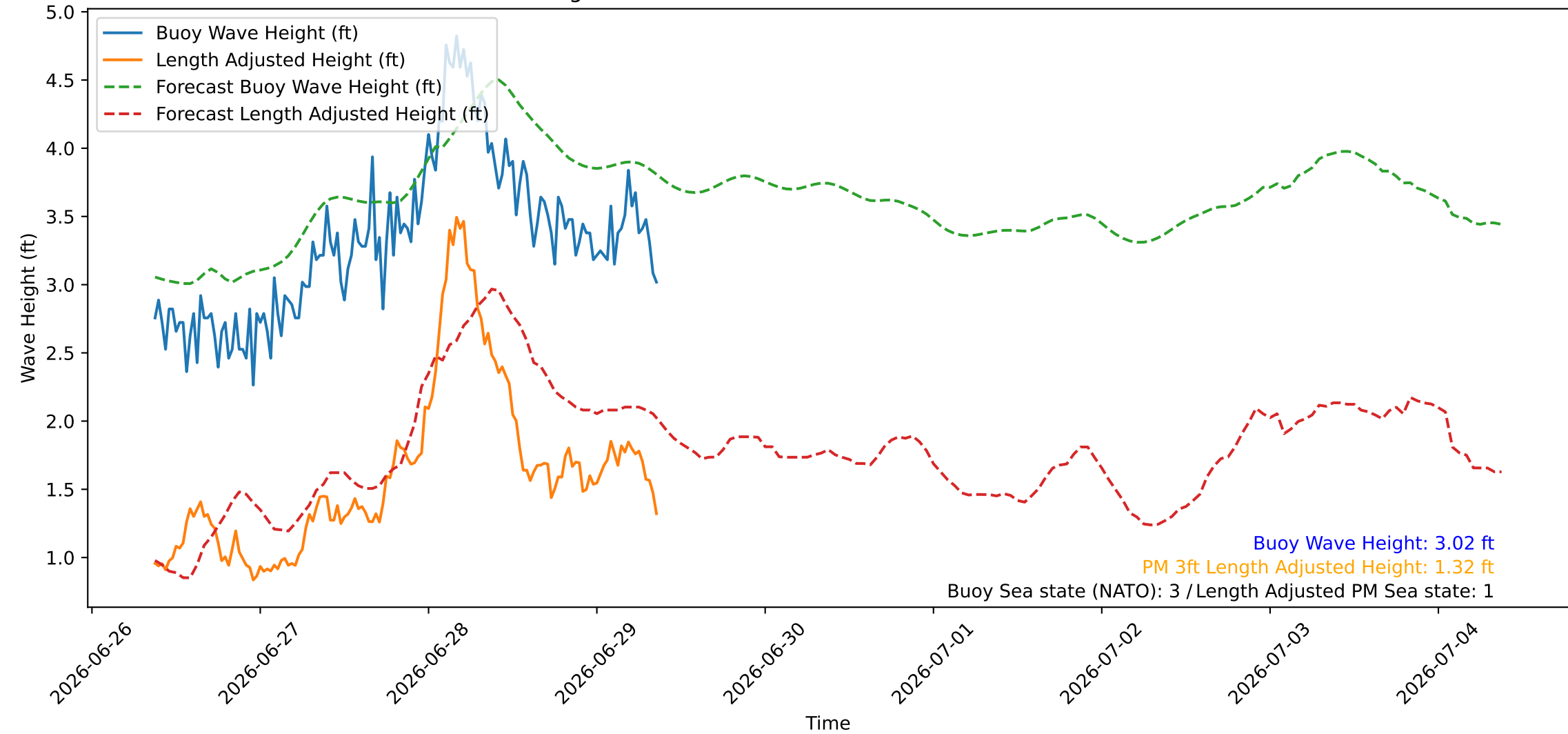
Wave Heights over Time for Green Beach at 2026-06-29 09:11:08
