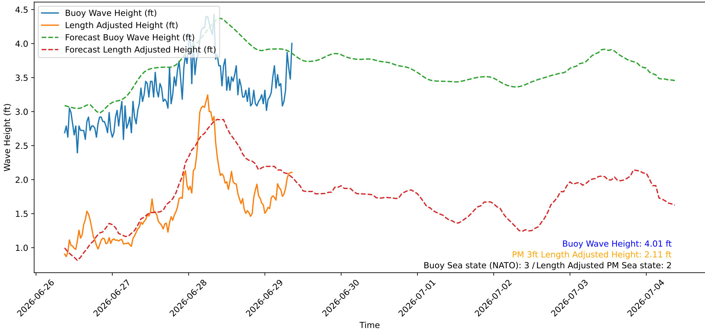
Wave Heights over Time for Oceanside Harbor at 2026-06-29 09:10:26
