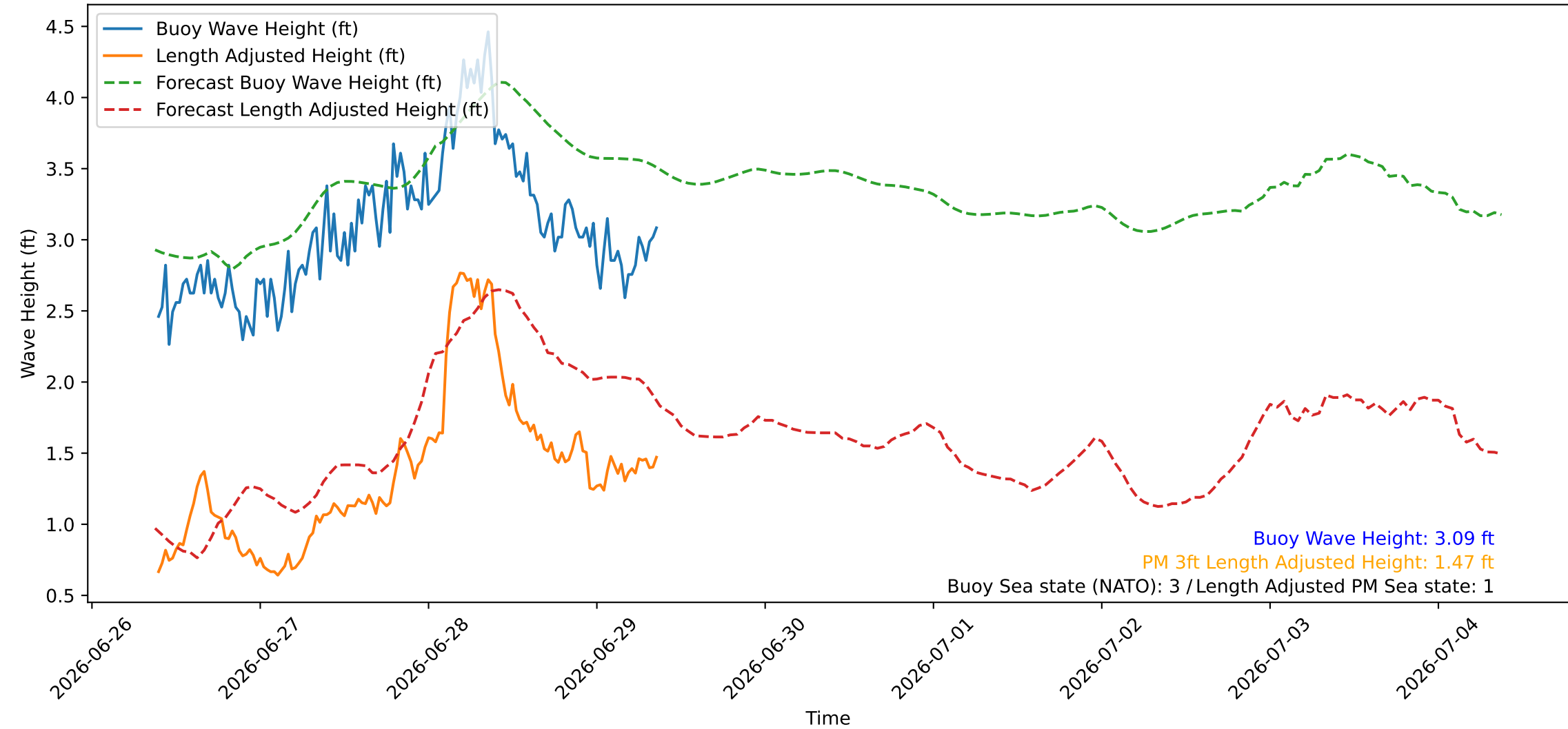
Wave Heights over Time for Red Beach at 2026-06-29 09:10:46
