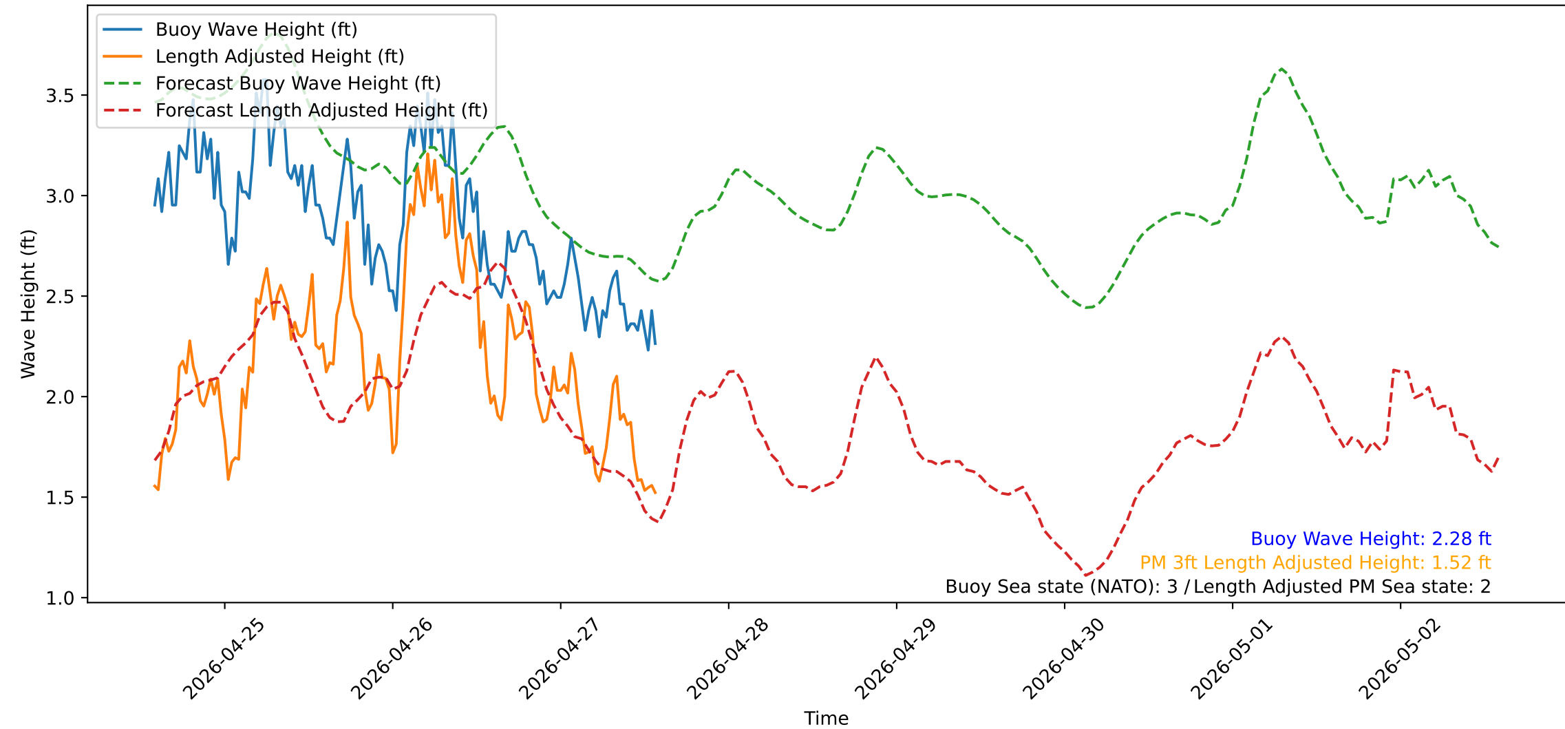
Wave Heights over Time for Green Beach at 2026-04-27 14:11:12
