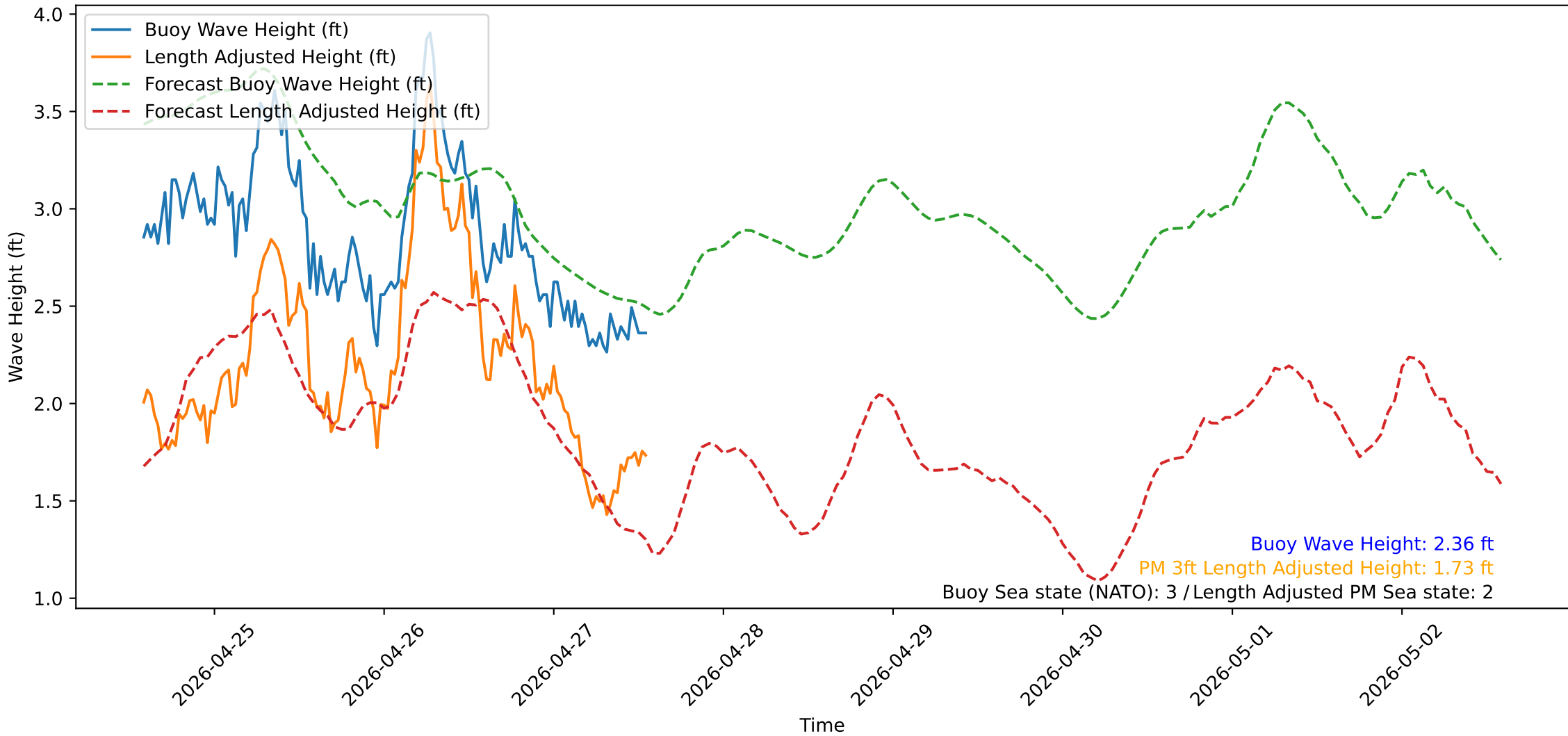
Wave Heights over Time for Oceanside Harbor at 2026-04-27 14:10:30
