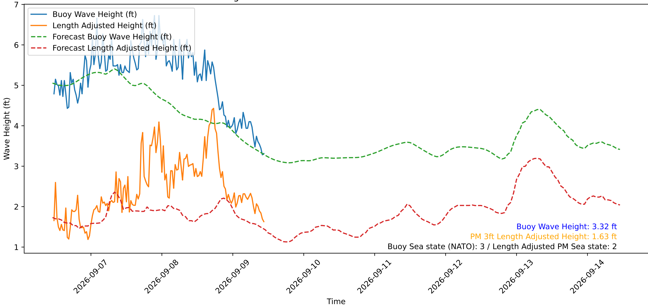
Wave Heights over Time for Red Beach at 2026-09-09 11:20:50
