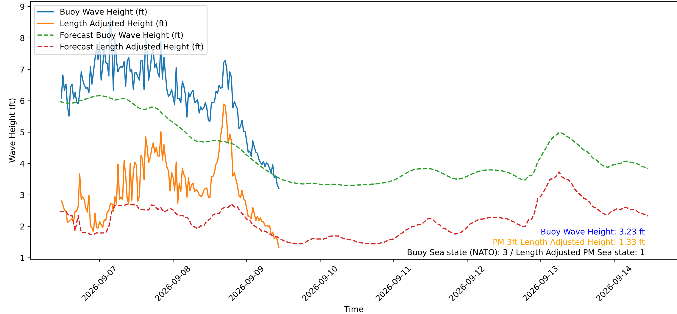
Wave Heights over Time for Green Beach at 2026-09-09 11:21:14
