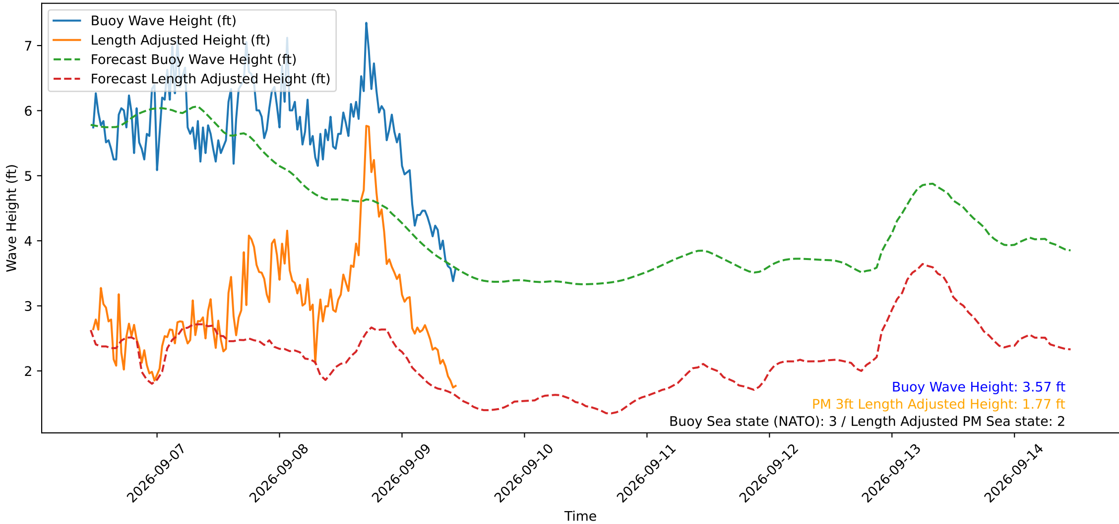
Wave Heights over Time for Oceanside Harbor at 2026-09-09 11:20:29
