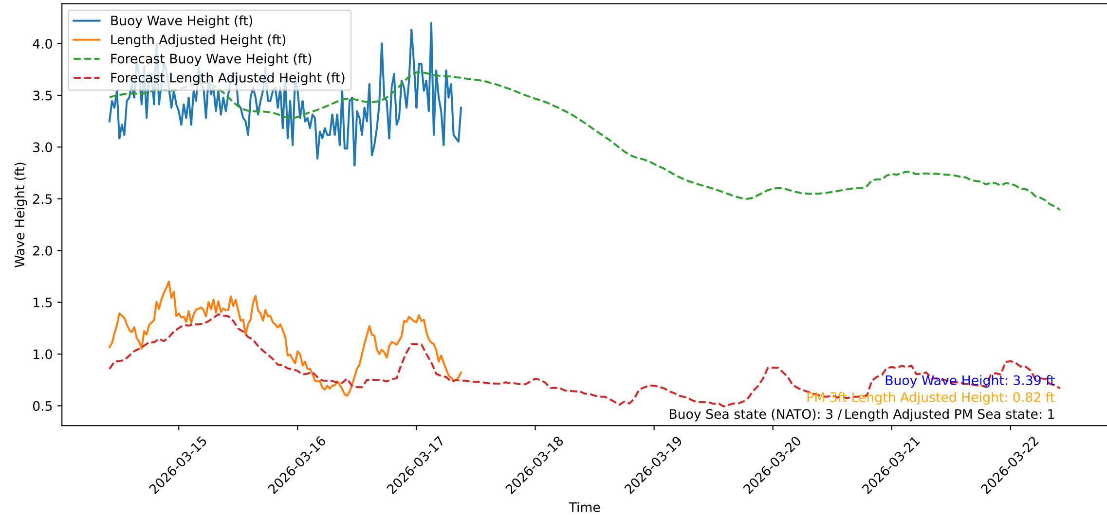
Wave Heights over Time for Green Beach at 2026-03-17 10:02:01
