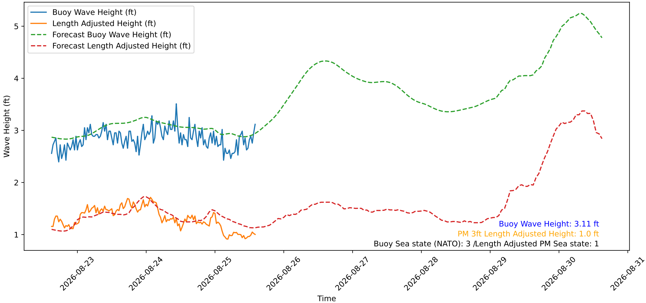
Wave Heights over Time for Oceanside Harbor at 2026-08-25 14:50:30
