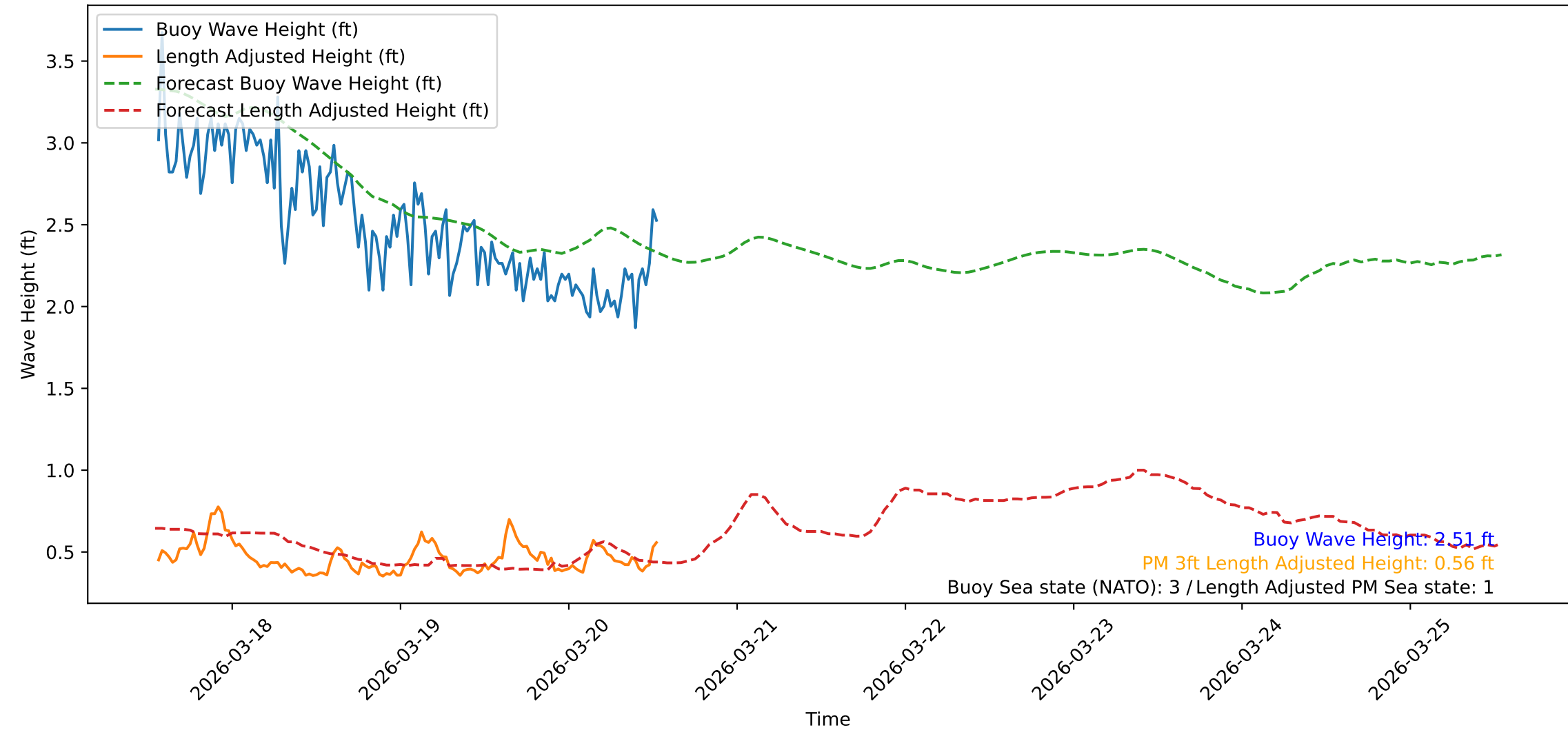
Wave Heights over Time for Red Beach at 2026-03-20 13:20:47
