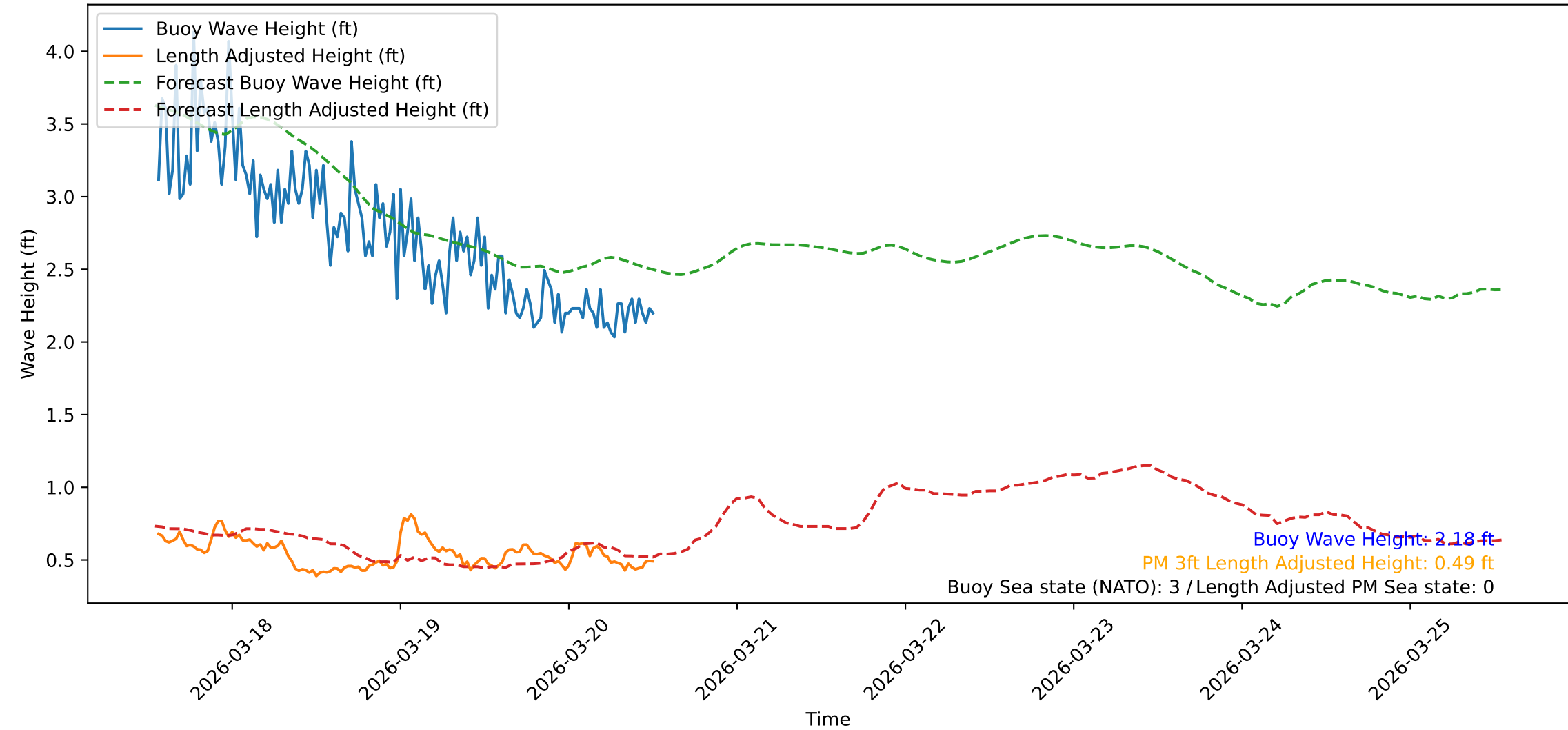
Wave Heights over Time for Green Beach at 2026-03-20 13:21:10
