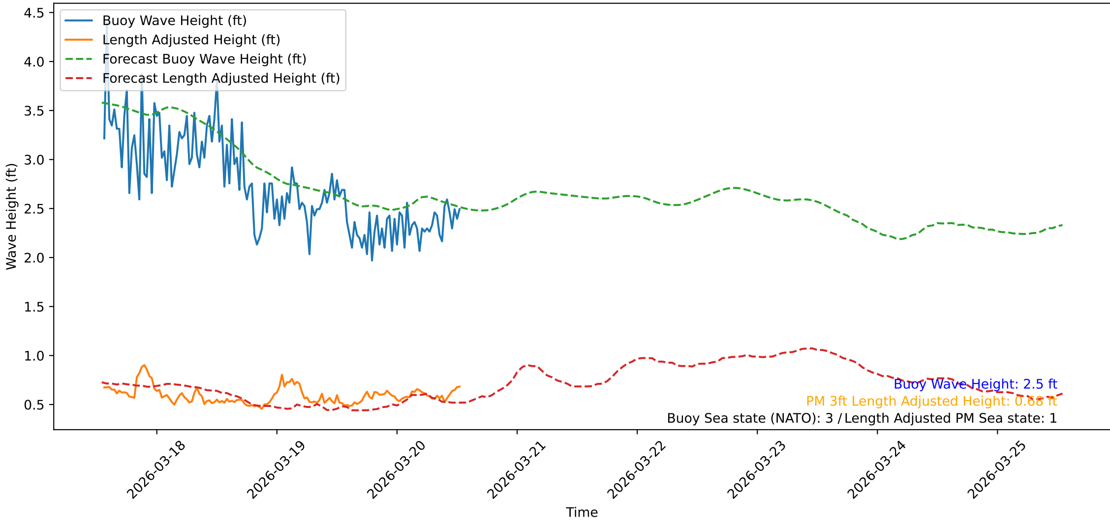
Wave Heights over Time for Oceanside Harbor at 2026-03-20 13:20:31
