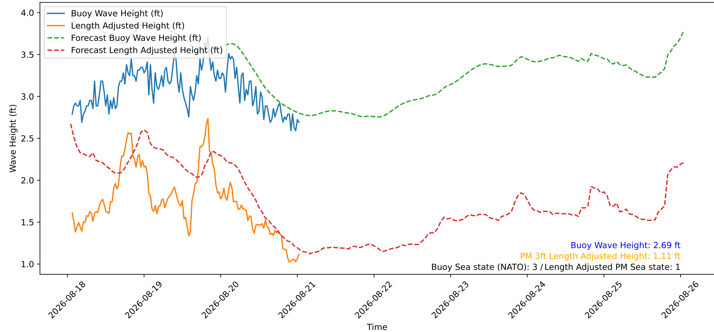
Wave Heights over Time for Green Beach at 2026-08-21 01:21:10
