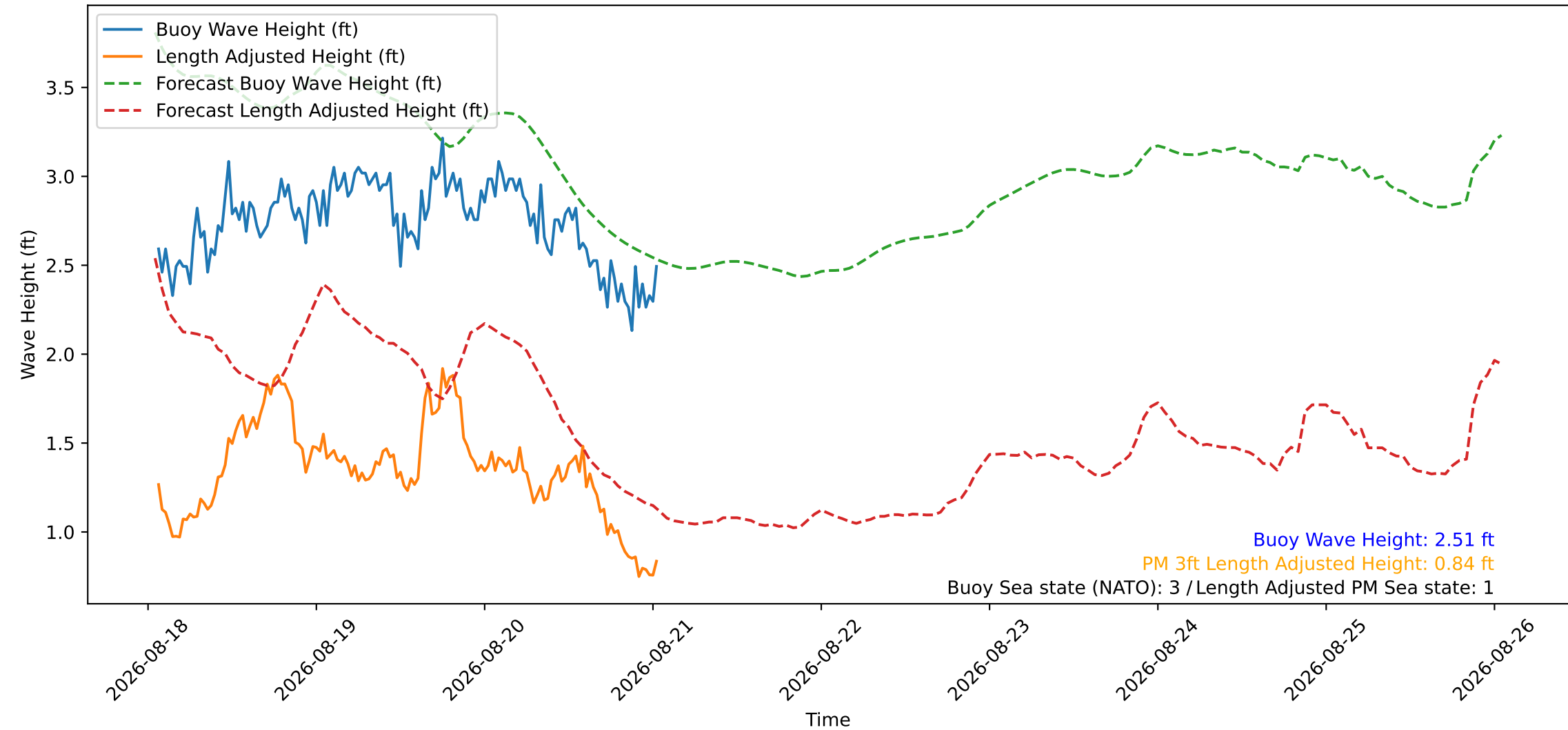
Wave Heights over Time for Red Beach at 2026-08-21 01:20:46
