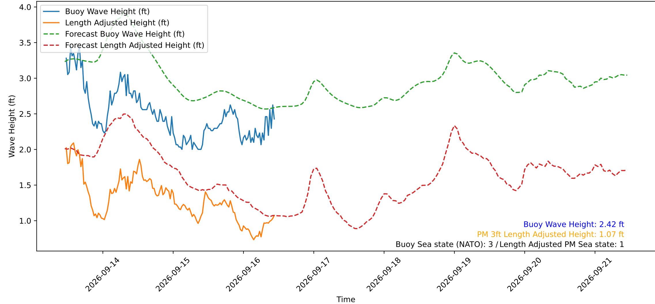
Wave Heights over Time for Red Beach at 2026-09-16 11:20:50
