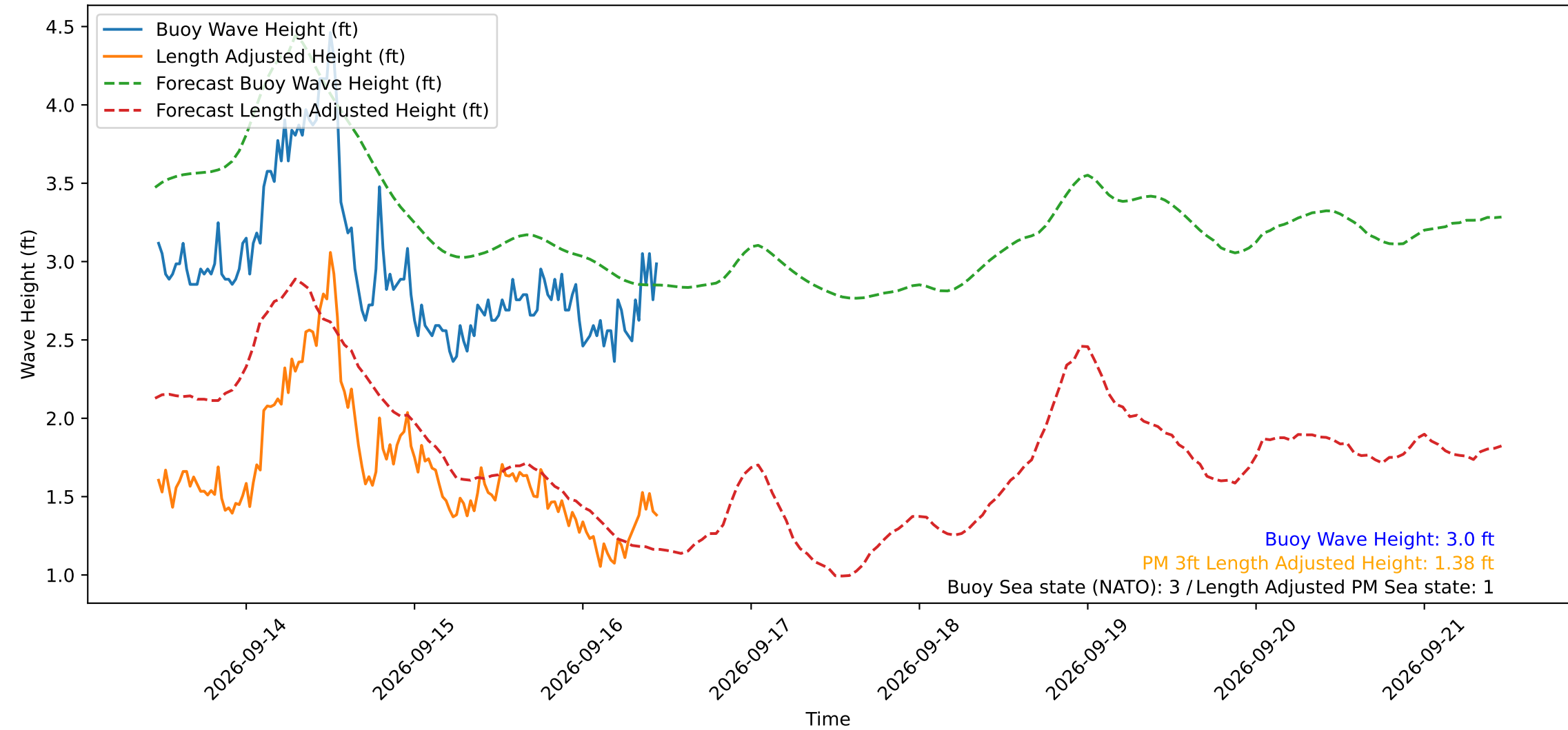
Wave Heights over Time for Oceanside Harbor at 2026-09-16 11:20:29
