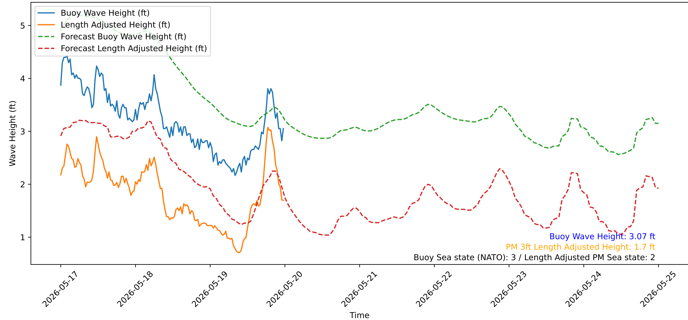
Wave Heights over Time for Green Beach at 2026-05-20 00:11:13
