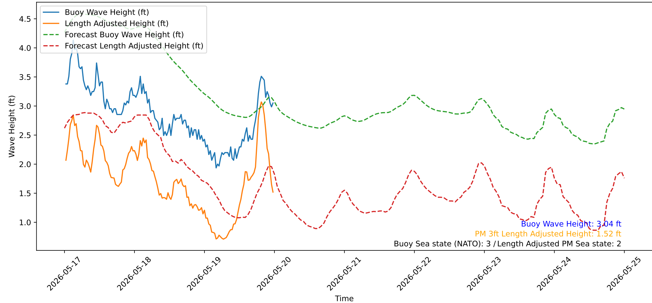
Wave Heights over Time for Red Beach at 2026-05-20 00:10:51
