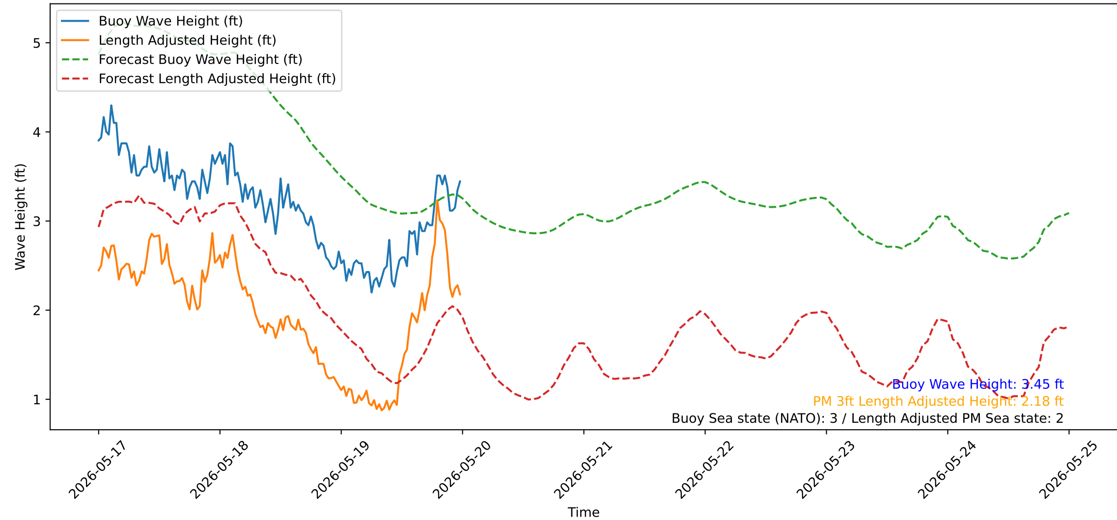
Wave Heights over Time for Oceanside Harbor at 2026-05-20 00:10:31
